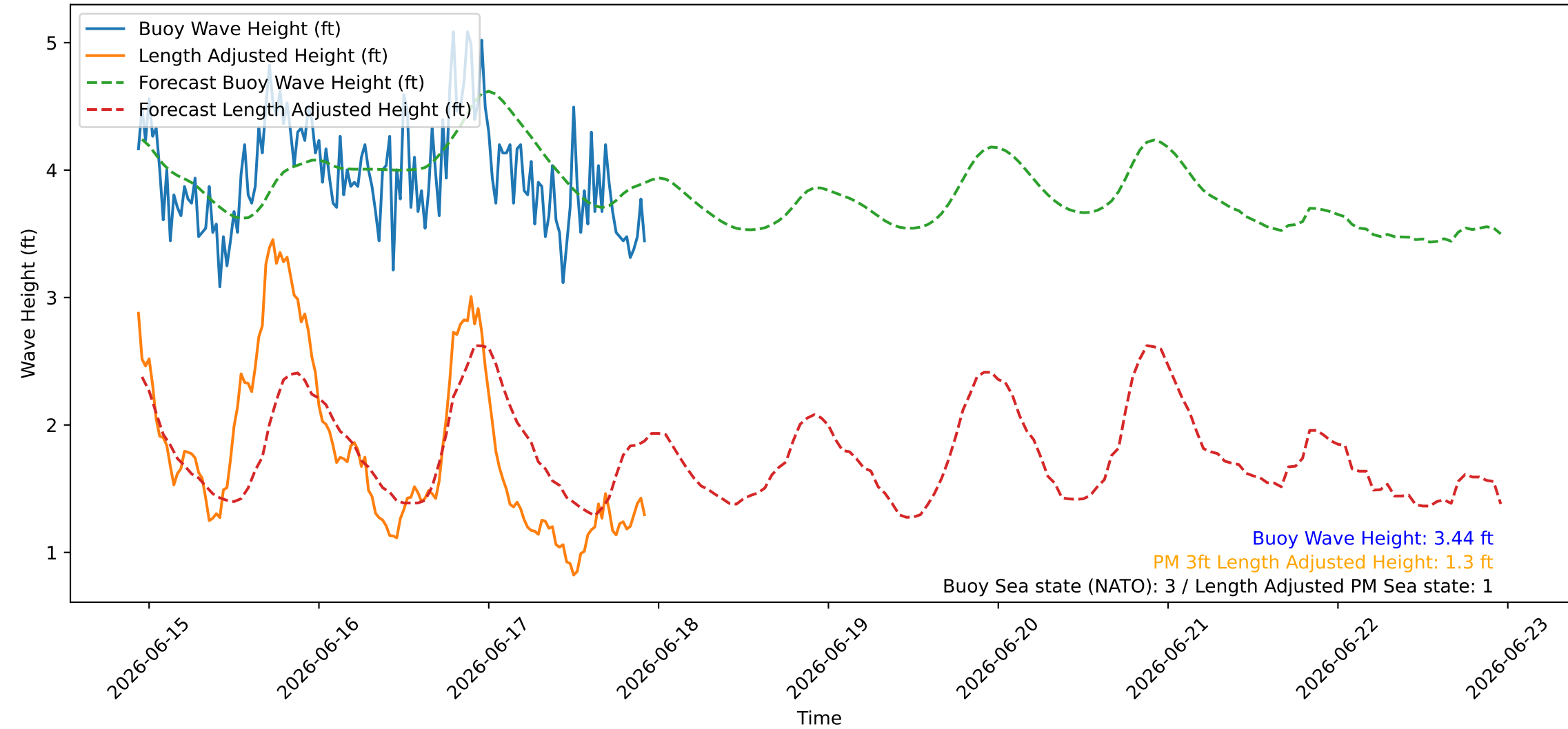
Wave Heights over Time for Green Beach at 2026-06-17 22:41:09
