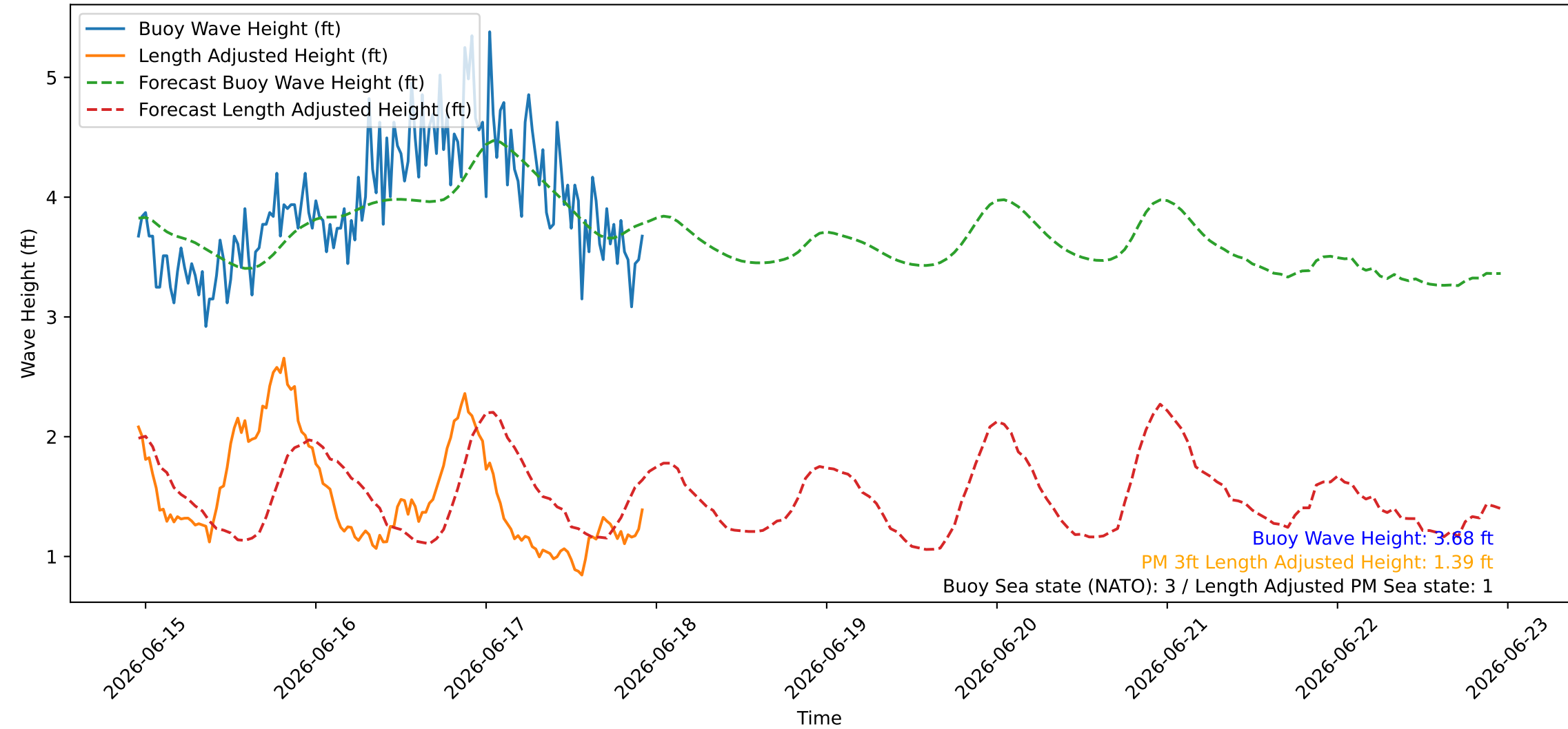
Wave Heights over Time for Red Beach at 2026-06-17 22:40:46
