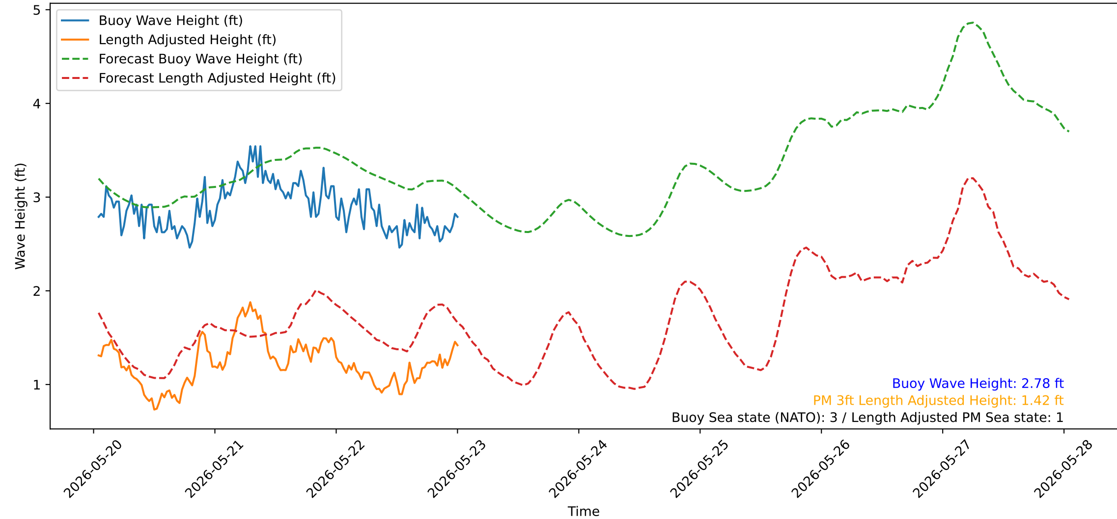
Wave Heights over Time for Green Beach at 2026-05-23 01:01:13
