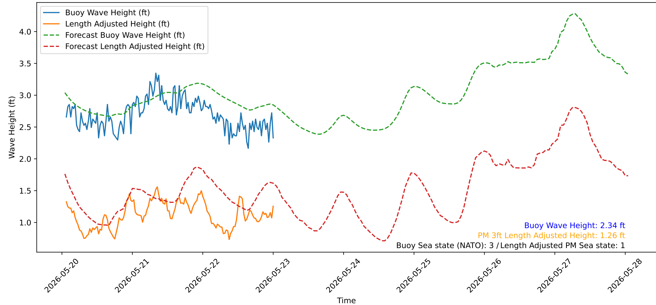
Wave Heights over Time for Red Beach at 2026-05-23 01:00:51
