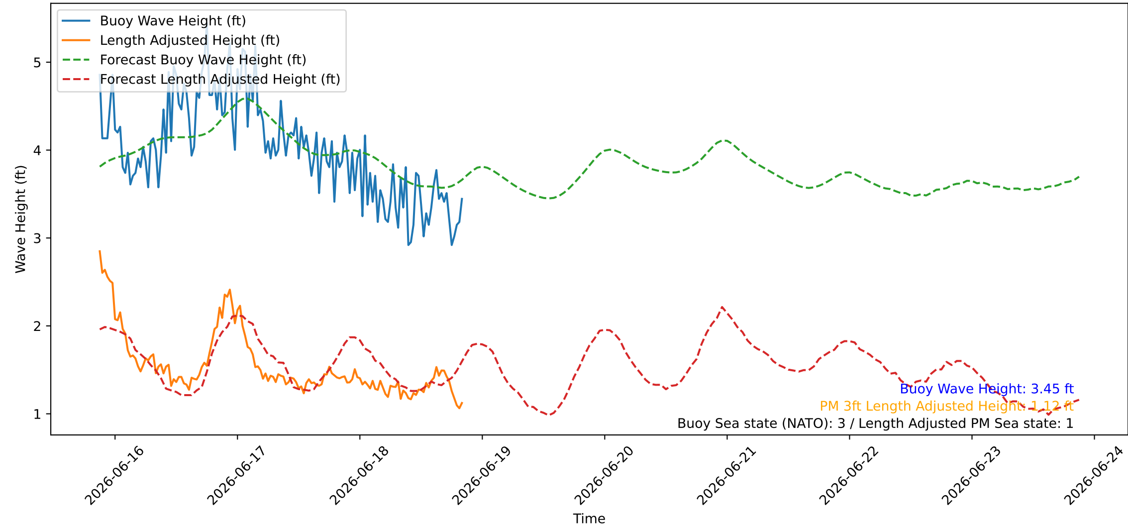
Wave Heights over Time for Oceanside Harbor at 2026-06-18 20:50:26
