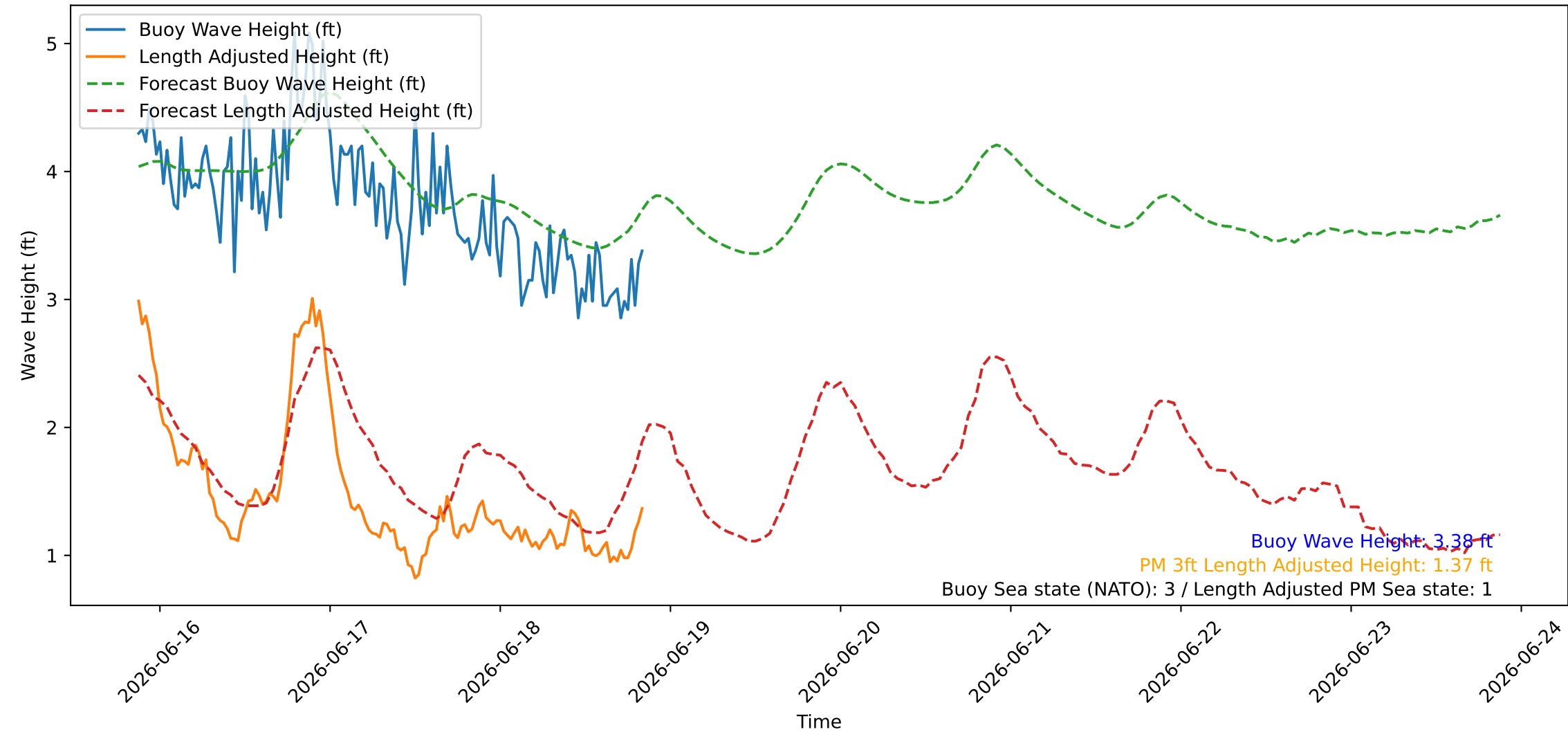
Wave Heights over Time for Green Beach at 2026-06-18 20:51:09
