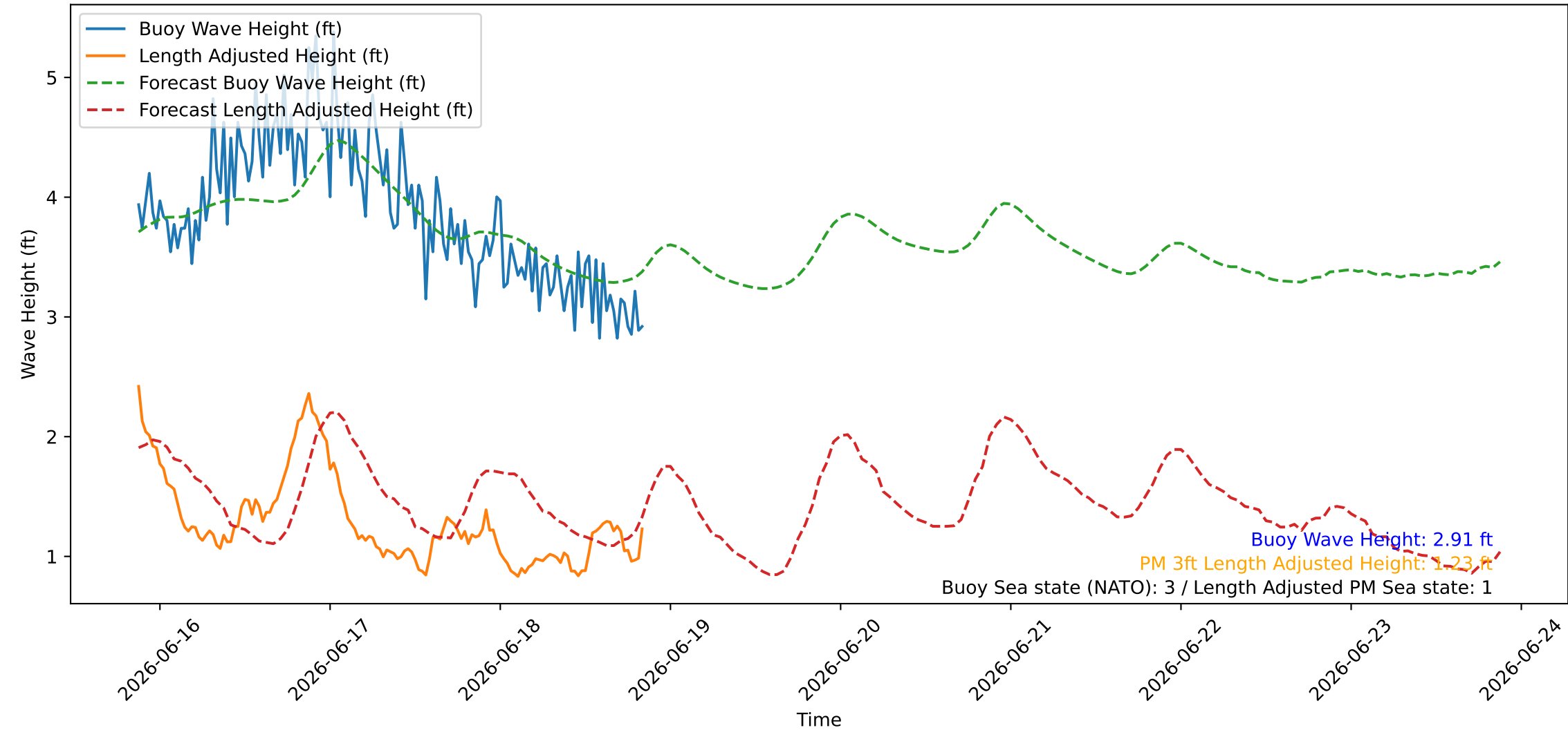
Wave Heights over Time for Red Beach at 2026-06-18 20:50:47
