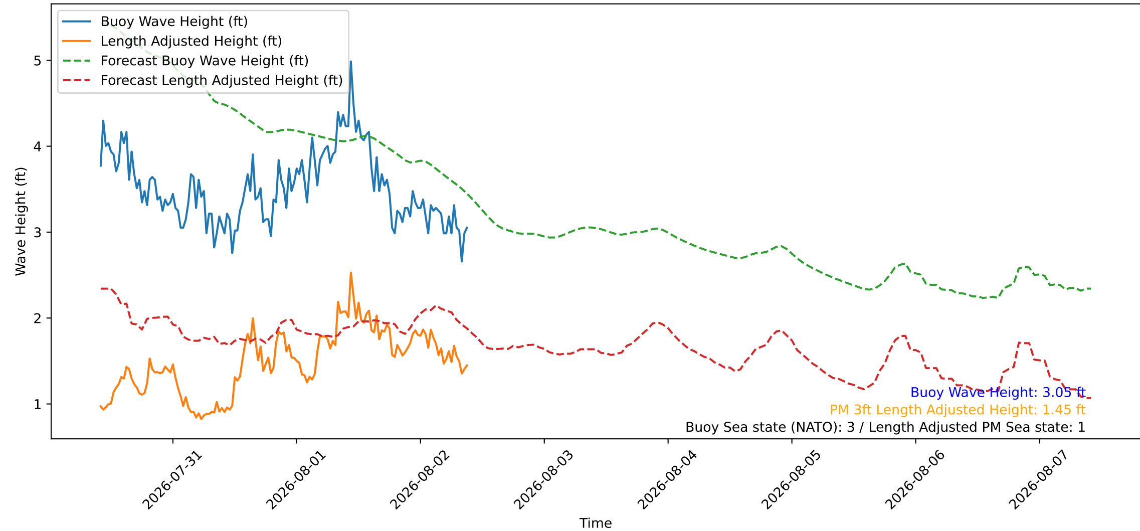
Wave Heights over Time for Green Beach at 2026-08-02 09:51:10
