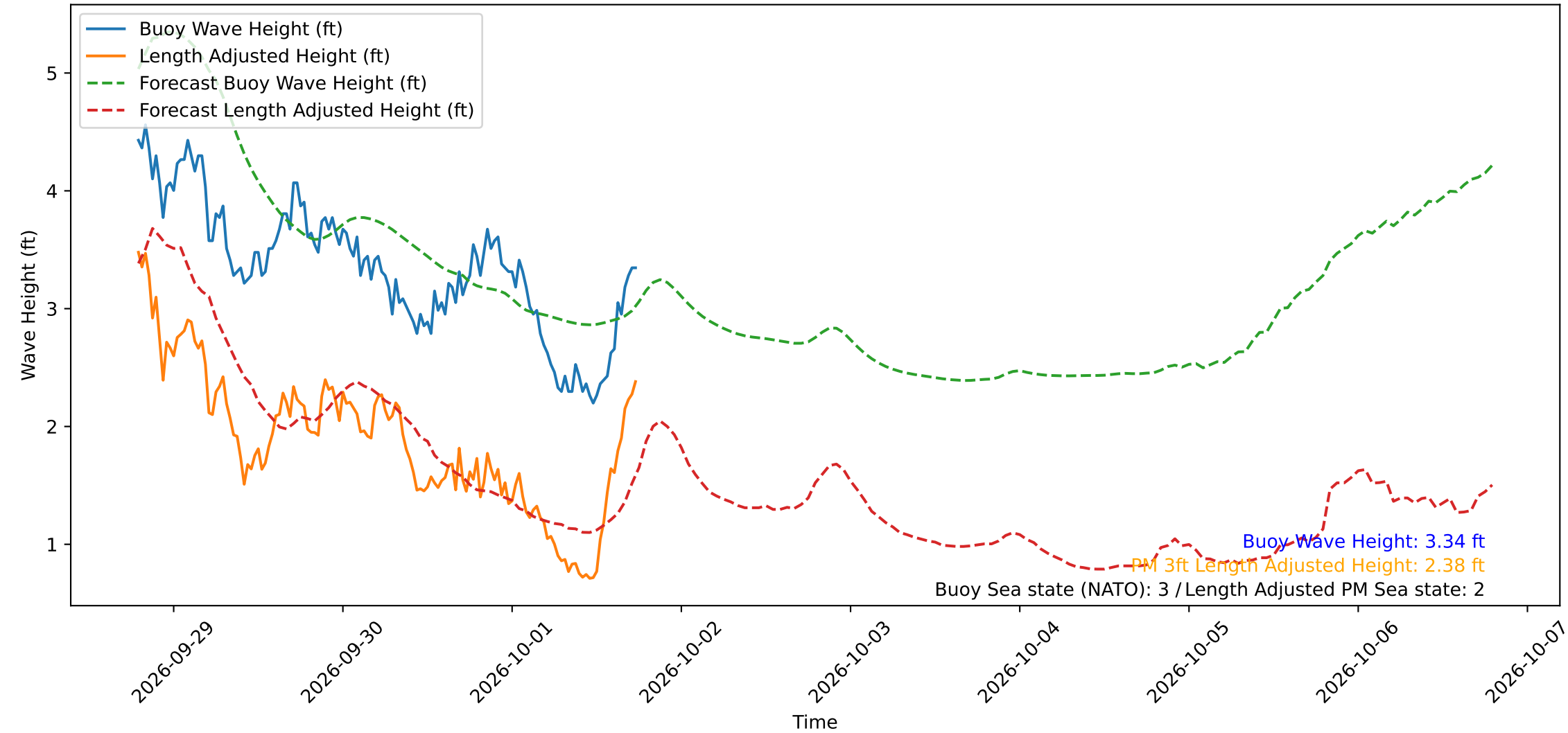
Wave Heights over Time for Green Beach at 2026-10-01 18:31:12
