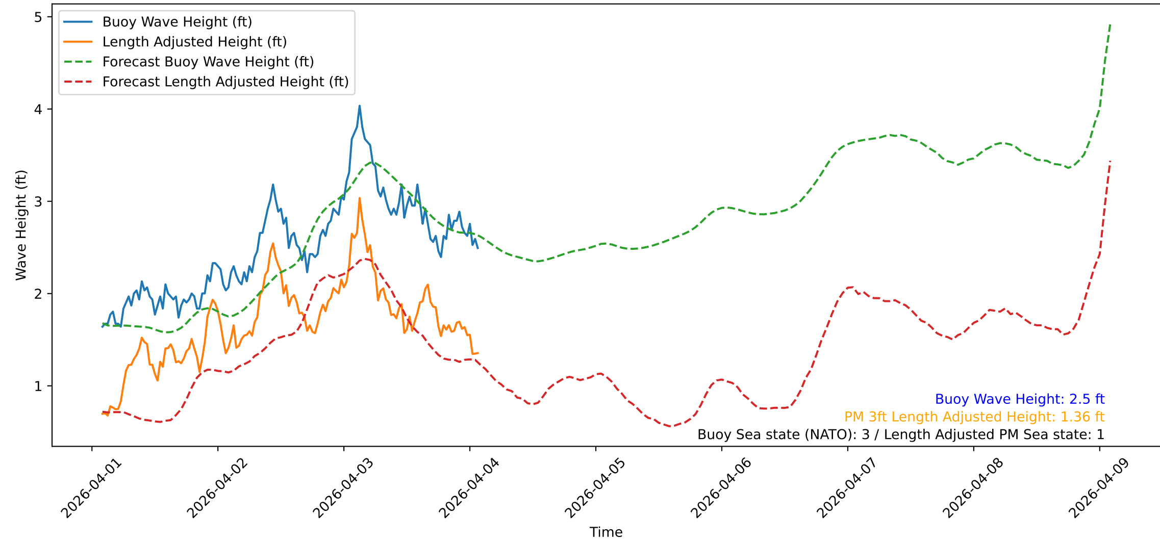
Wave Heights over Time for Oceanside Harbor at 2026-04-04 02:00:31
