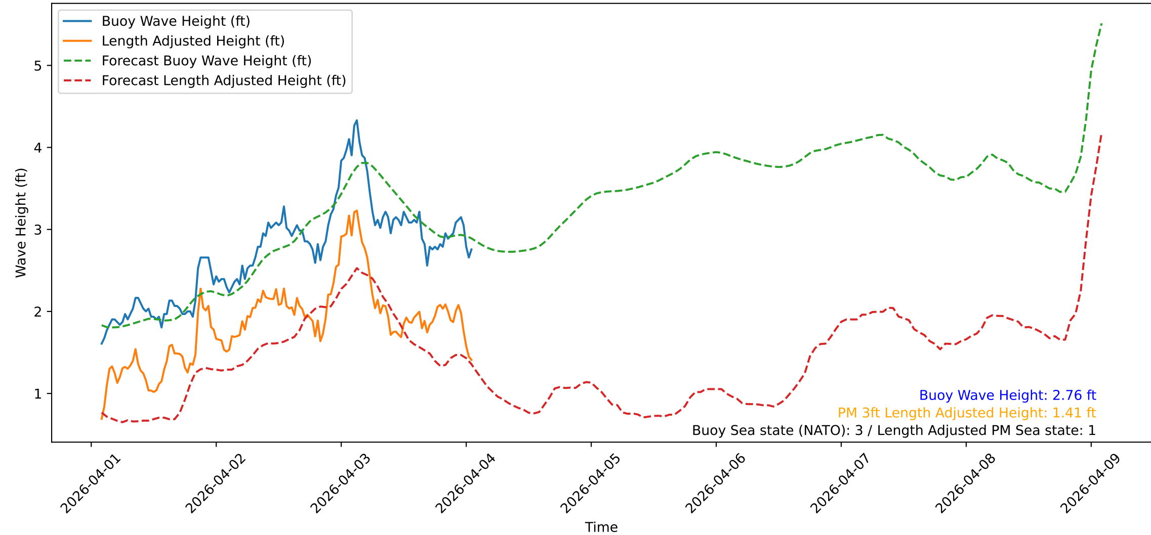
Wave Heights over Time for Green Beach at 2026-04-04 02:01:09
