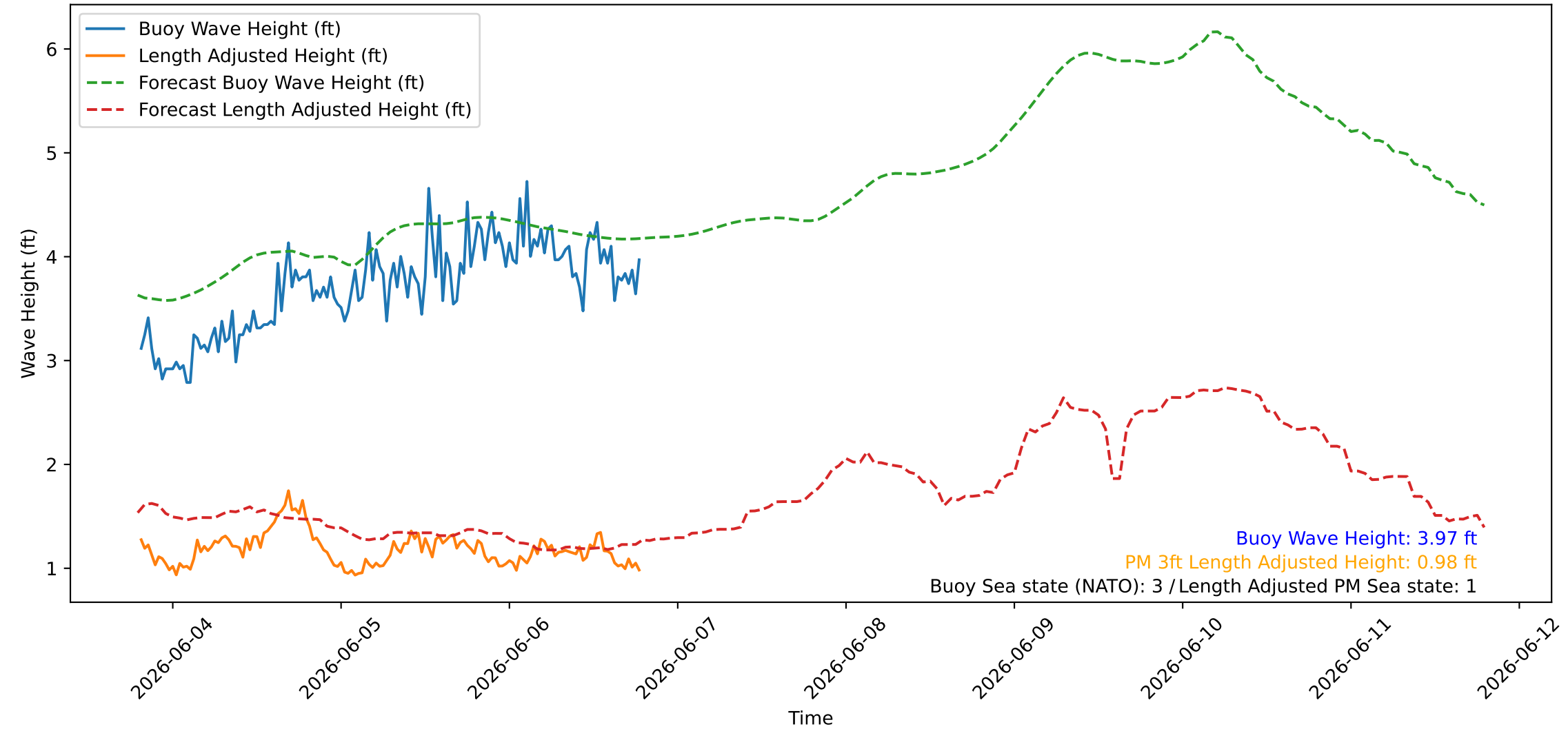
Wave Heights over Time for Green Beach at 2026-06-06 19:21:08
