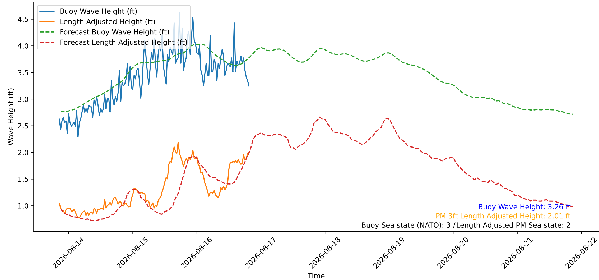
Wave Heights over Time for Oceanside Harbor at 2026-08-16 20:40:26
