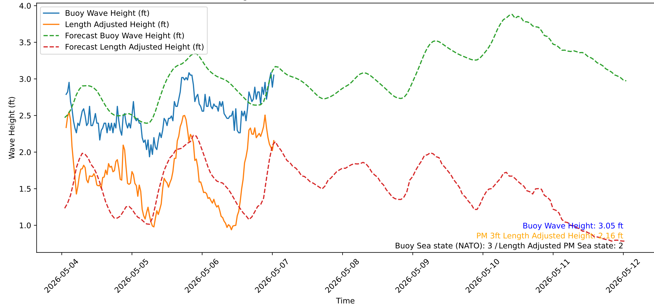
Wave Heights over Time for Red Beach at 2026-05-07 01:20:52
