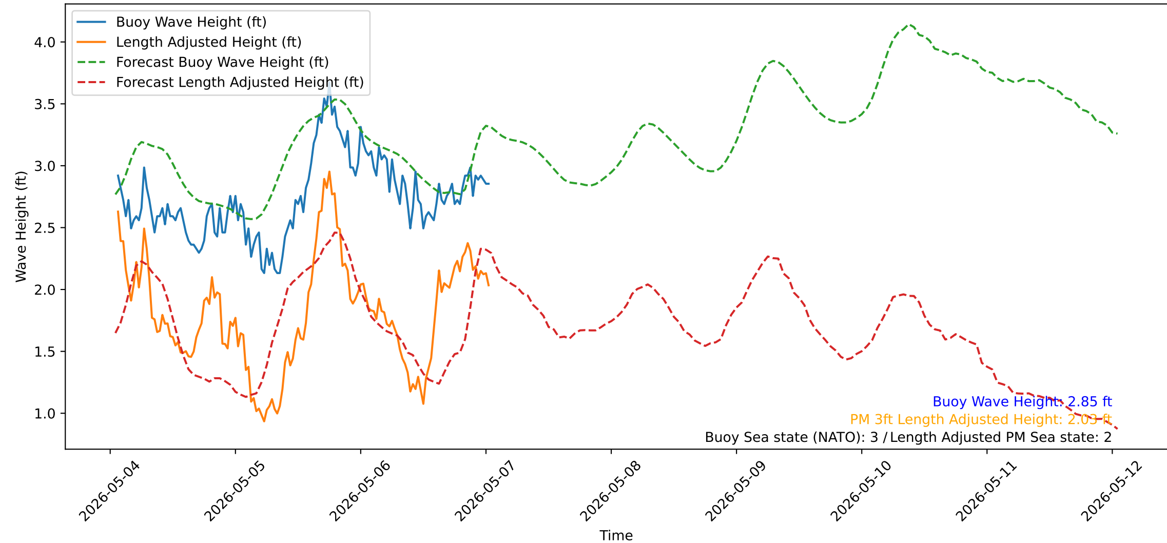
Wave Heights over Time for Green Beach at 2026-05-07 01:21:14
