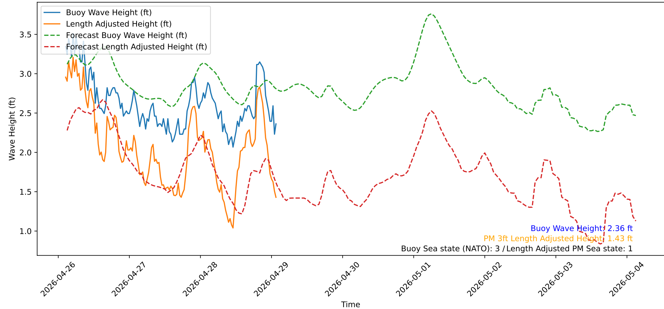
Wave Heights over Time for Green Beach at 2026-04-29 02:31:13
