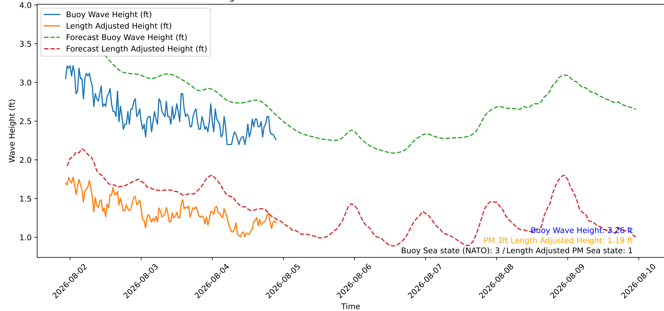
Wave Heights over Time for Oceanside Harbor at 2026-08-04 22:30:27
