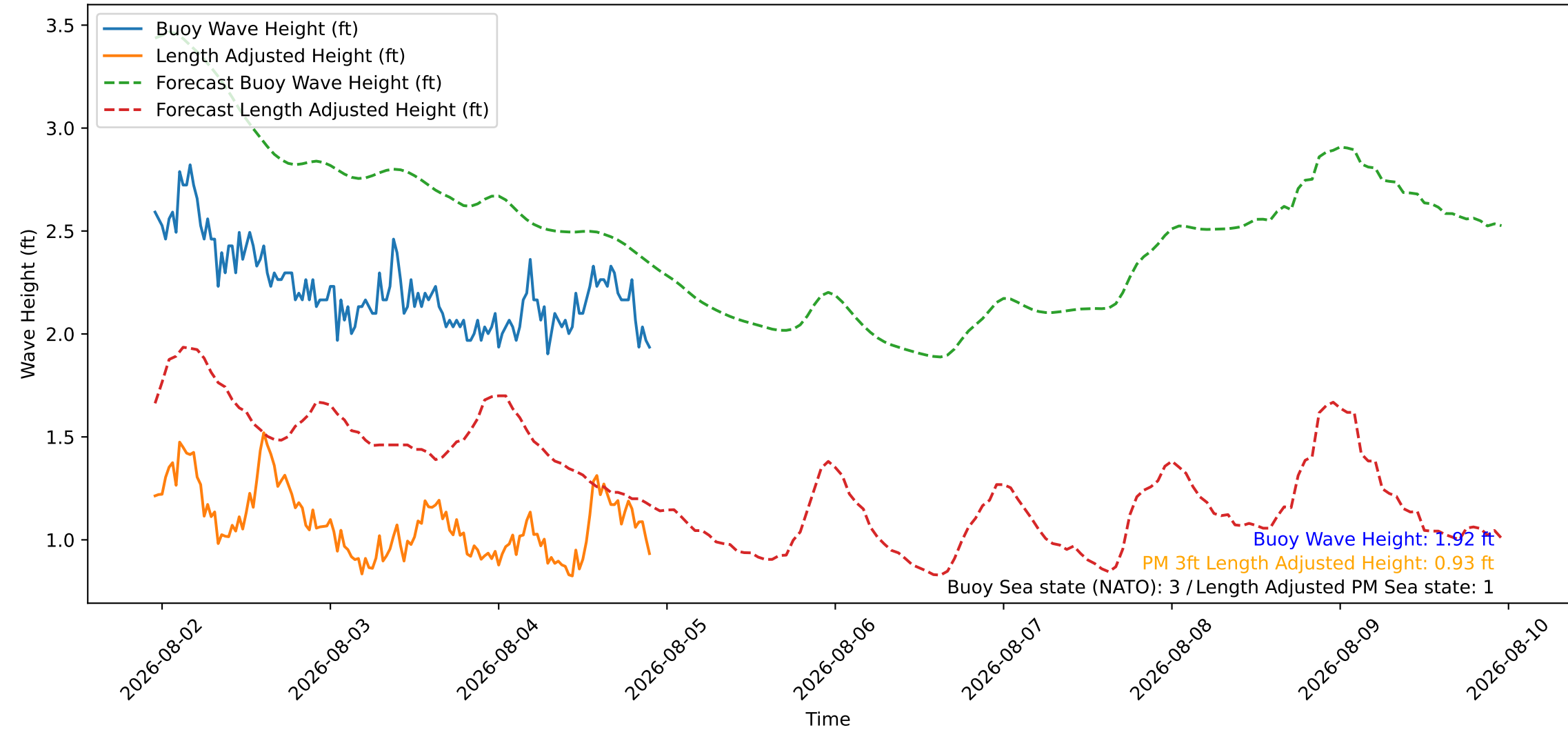
Wave Heights over Time for Red Beach at 2026-08-04 22:30:46
