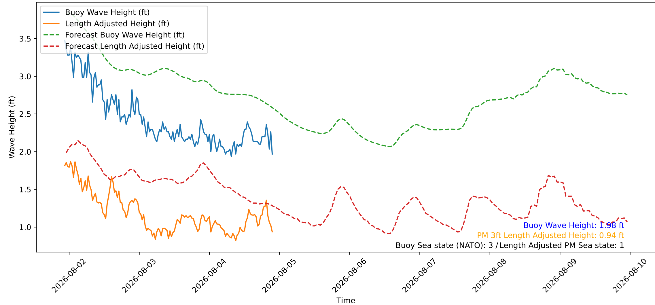
Wave Heights over Time for Green Beach at 2026-08-04 22:31:09
