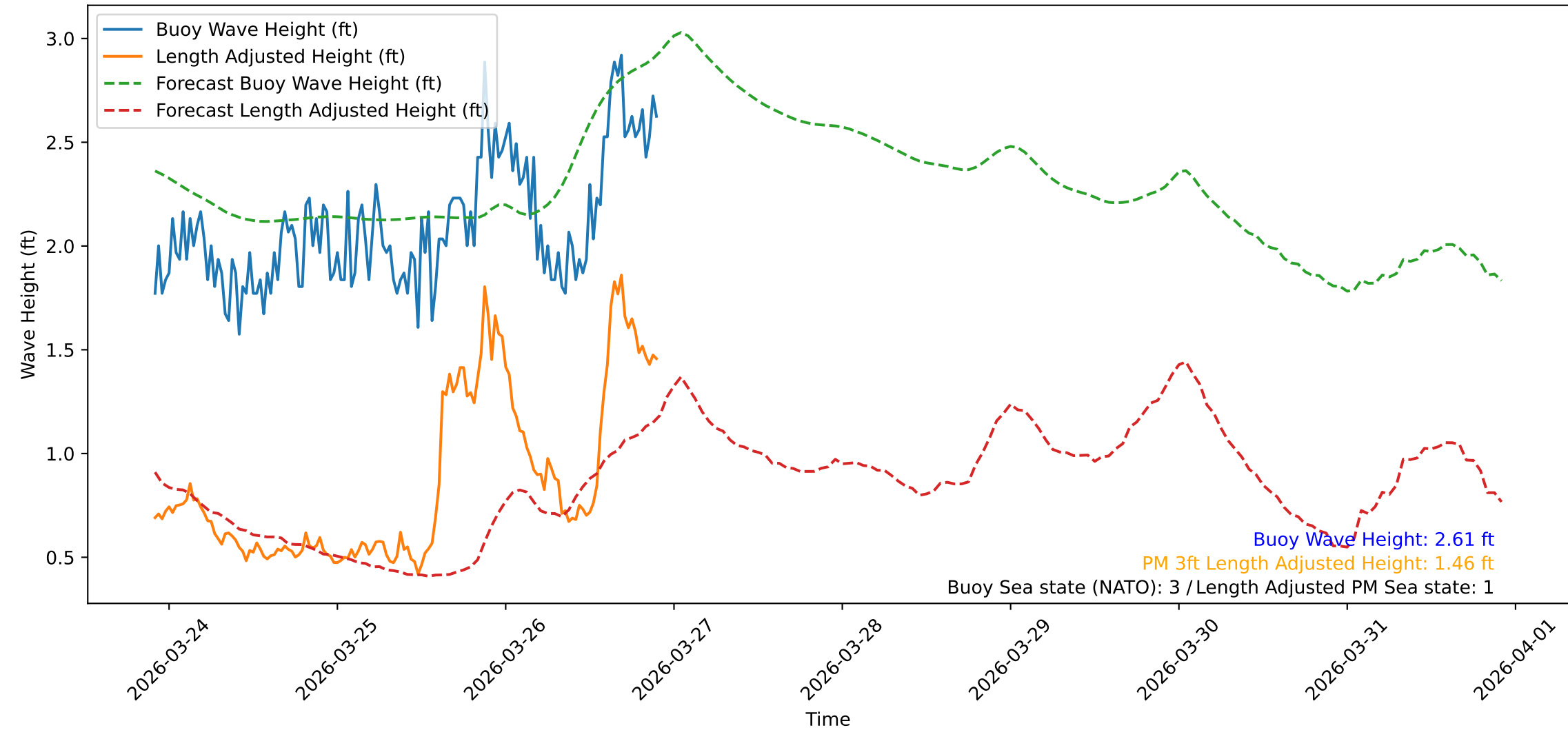
Wave Heights over Time for Oceanside Harbor at 2026-03-26 22:10:31
