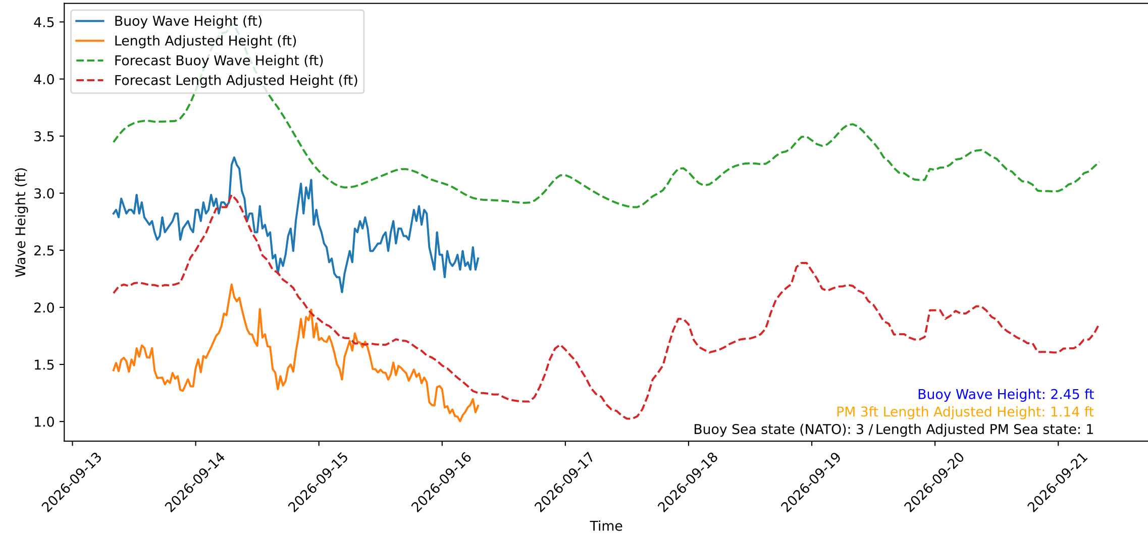
Wave Heights over Time for Green Beach at 2026-09-16 07:51:14
