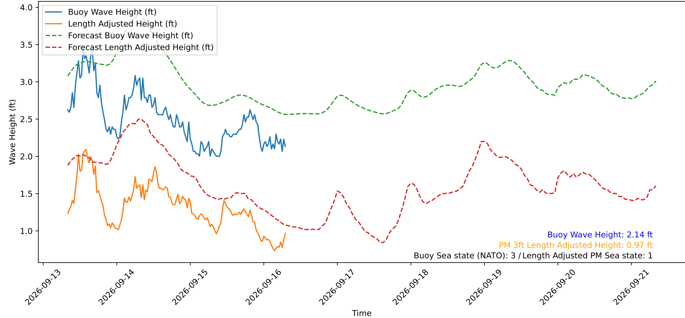
Wave Heights over Time for Red Beach at 2026-09-16 07:50:50
