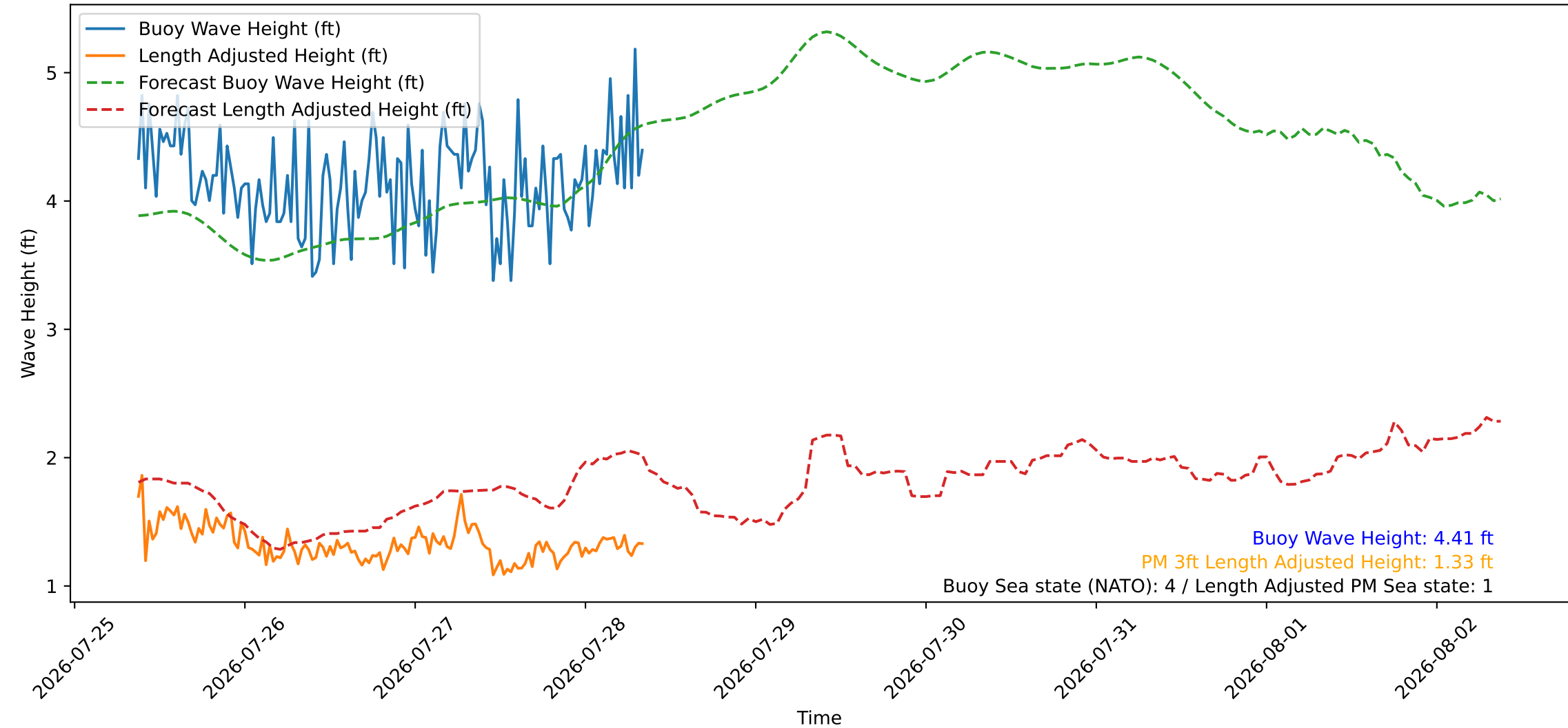
Wave Heights over Time for Green Beach at 2026-07-28 08:51:12
