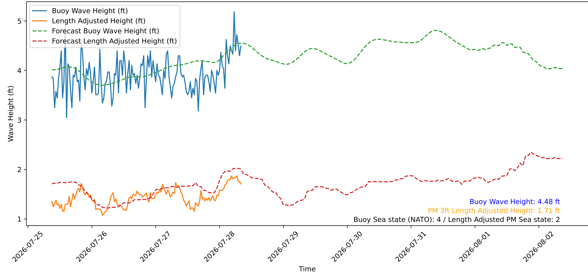
Wave Heights over Time for Oceanside Harbor at 2026-07-28 08:50:29
