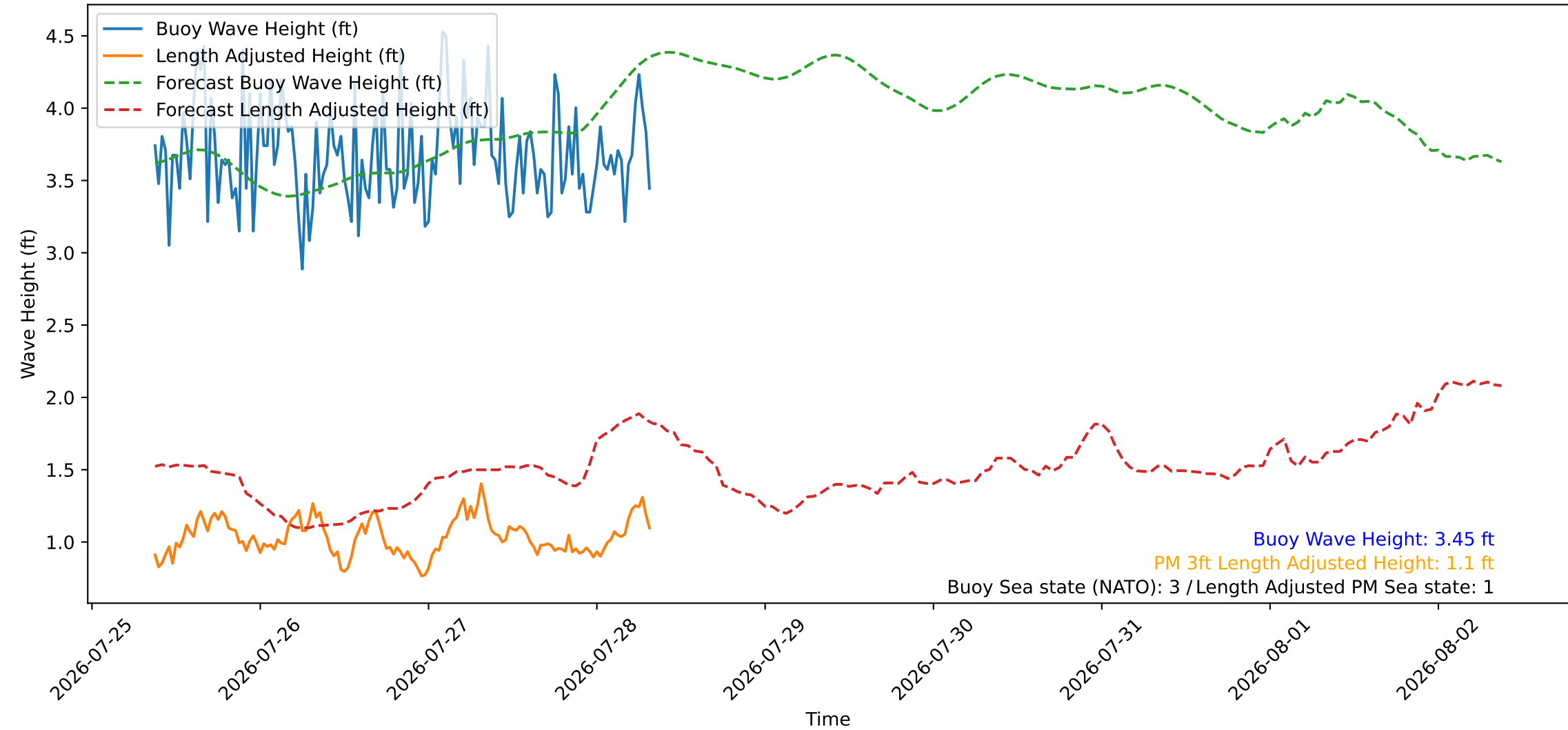
Wave Heights over Time for Red Beach at 2026-07-28 08:50:50
