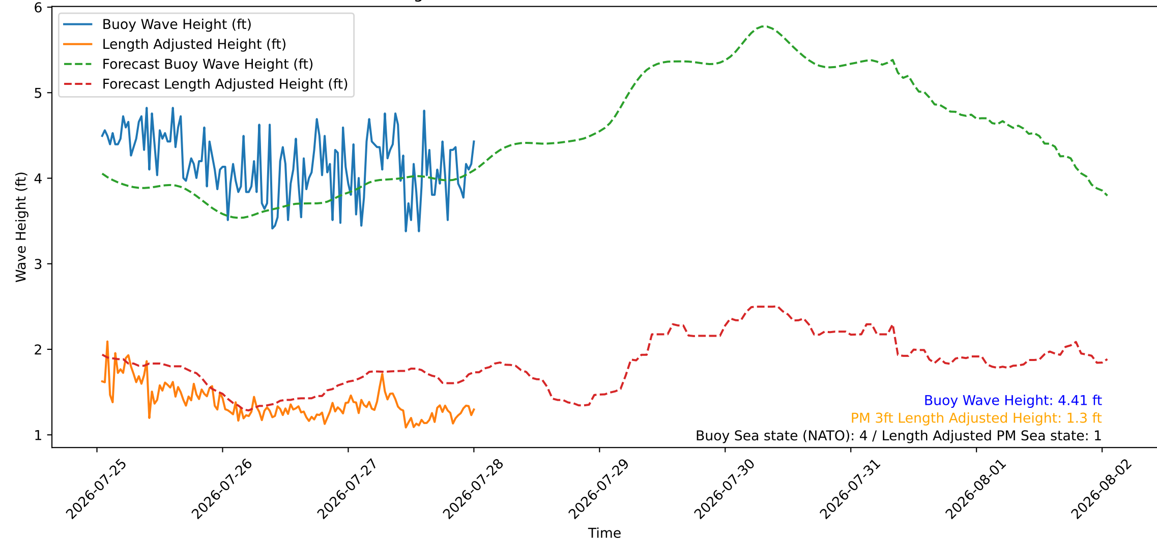
Wave Heights over Time for Green Beach at 2026-07-28 00:51:10
