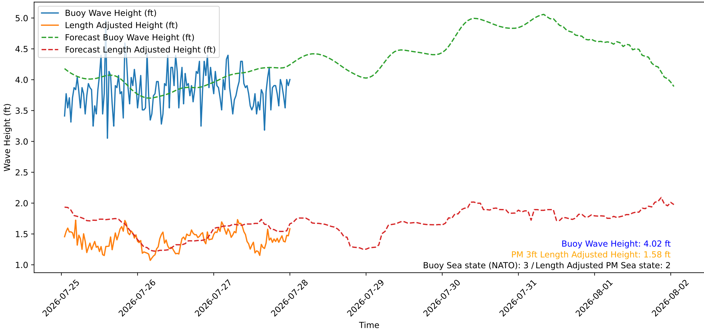
Wave Heights over Time for Oceanside Harbor at 2026-07-28 00:50:26
