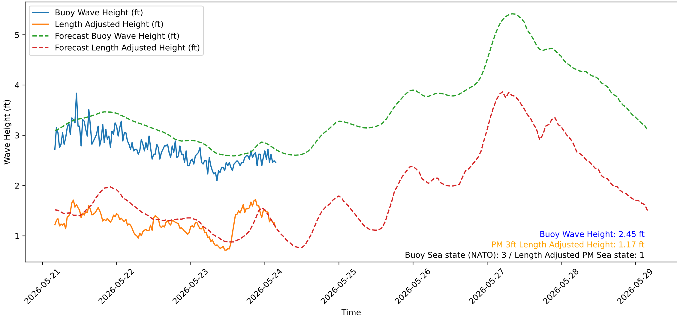
Wave Heights over Time for Oceanside Harbor at 2026-05-24 04:10:31
