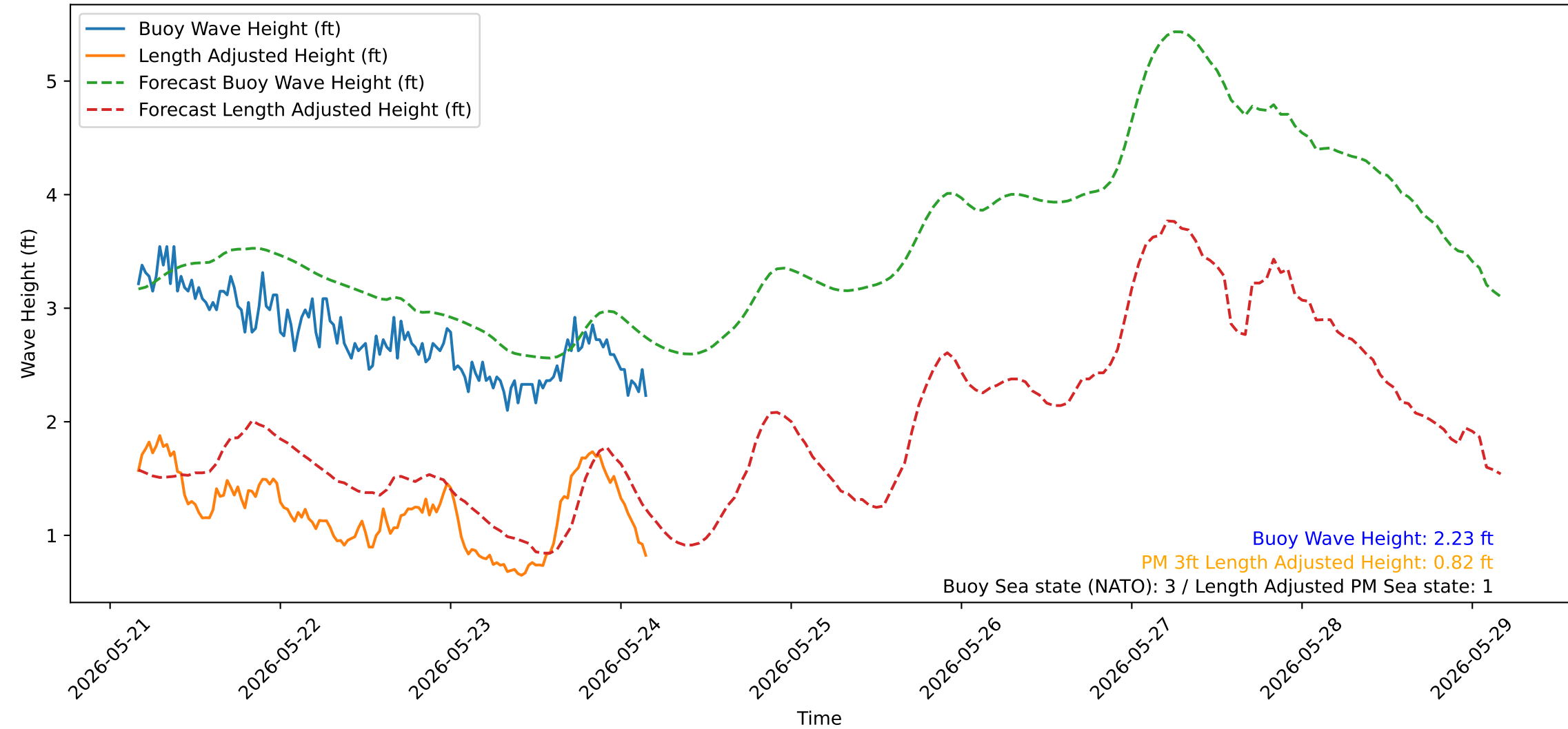
Wave Heights over Time for Green Beach at 2026-05-24 04:11:15
