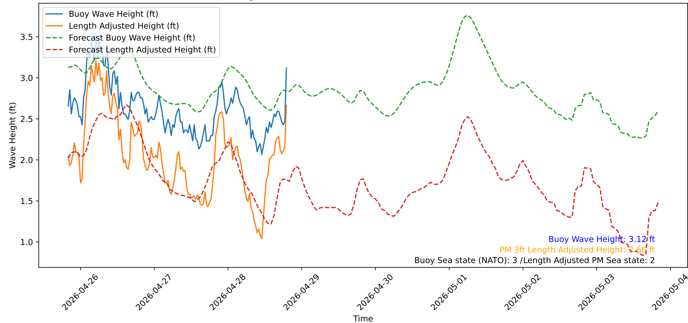
Wave Heights over Time for Green Beach at 2026-04-28 20:01:14
