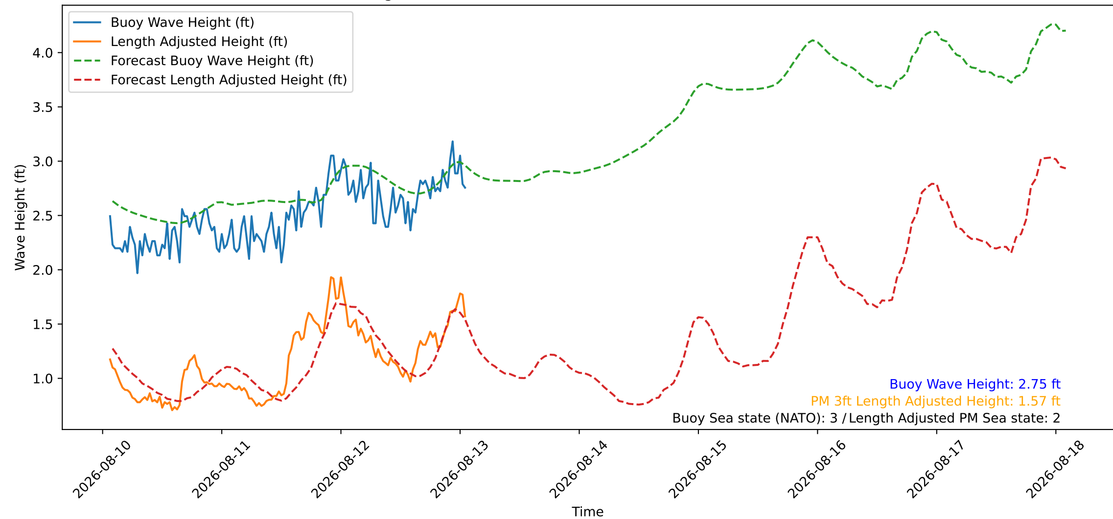
Wave Heights over Time for Oceanside Harbor at 2026-08-13 01:30:26
