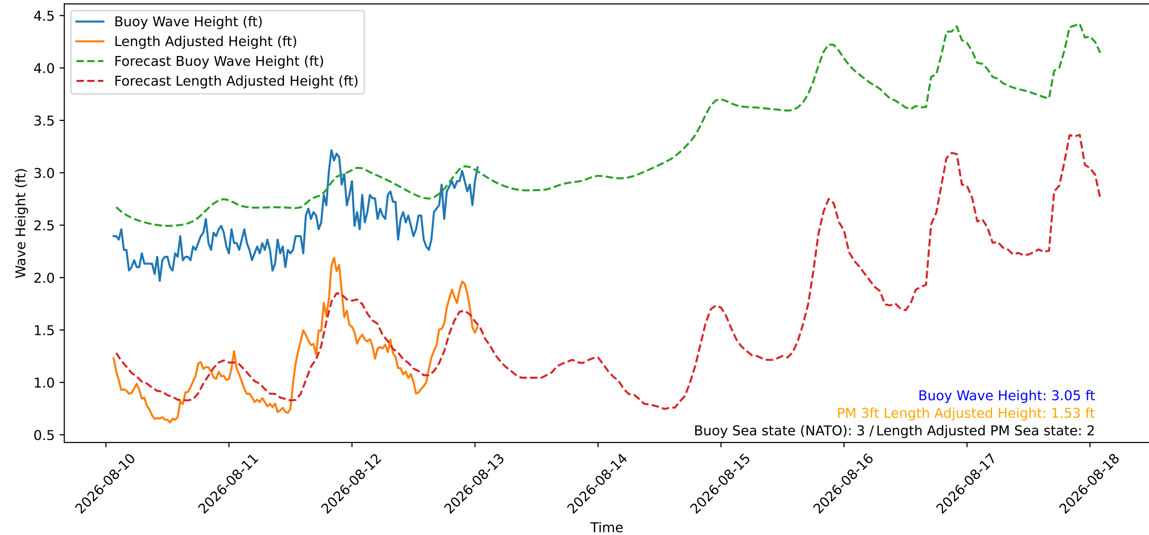
Wave Heights over Time for Green Beach at 2026-08-13 01:31:08
