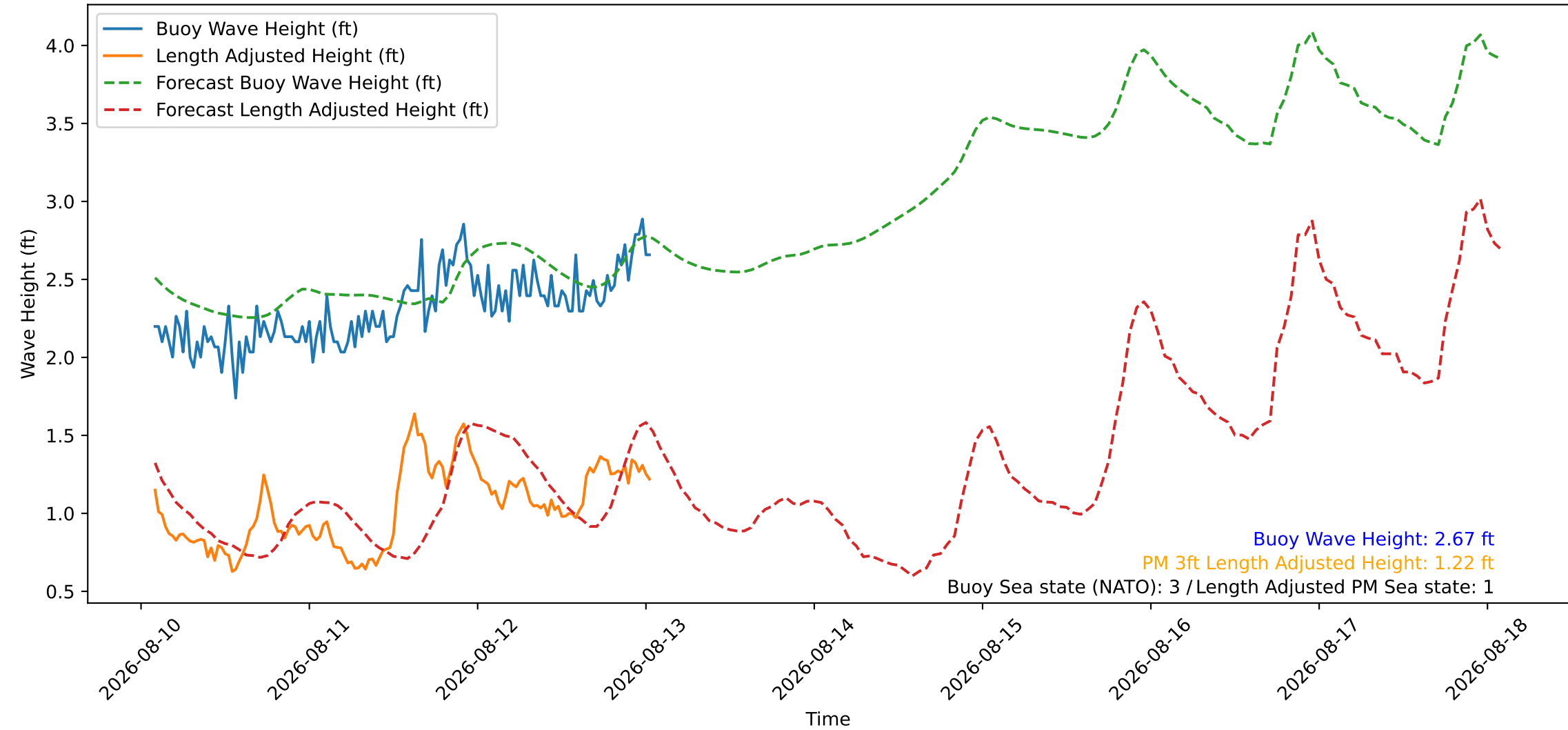
Wave Heights over Time for Red Beach at 2026-08-13 01:30:45
