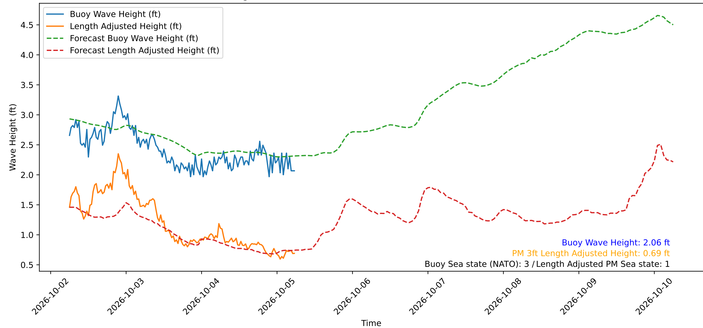
Wave Heights over Time for Oceanside Harbor at 2026-10-05 06:10:30
