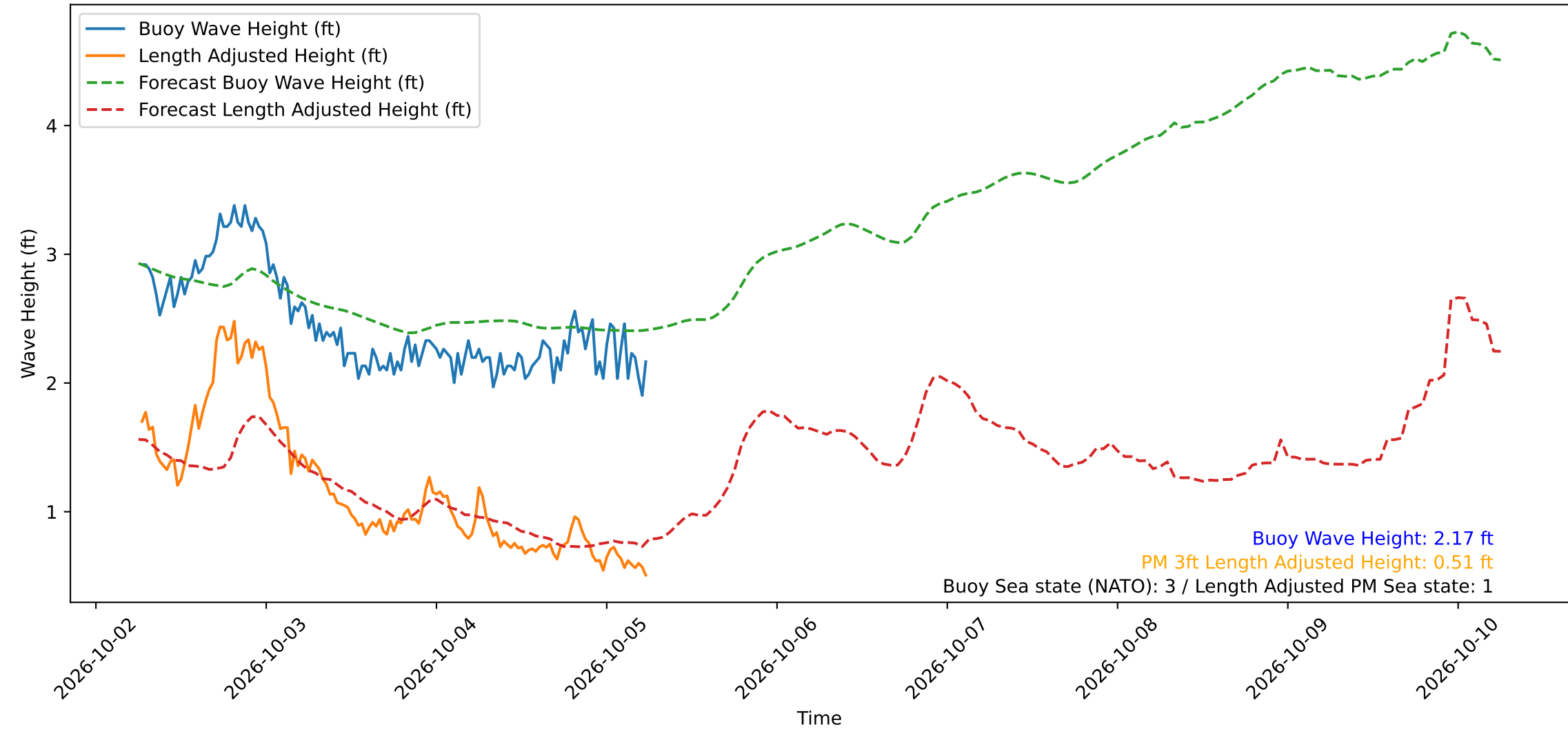
Wave Heights over Time for Green Beach at 2026-10-05 06:11:11
