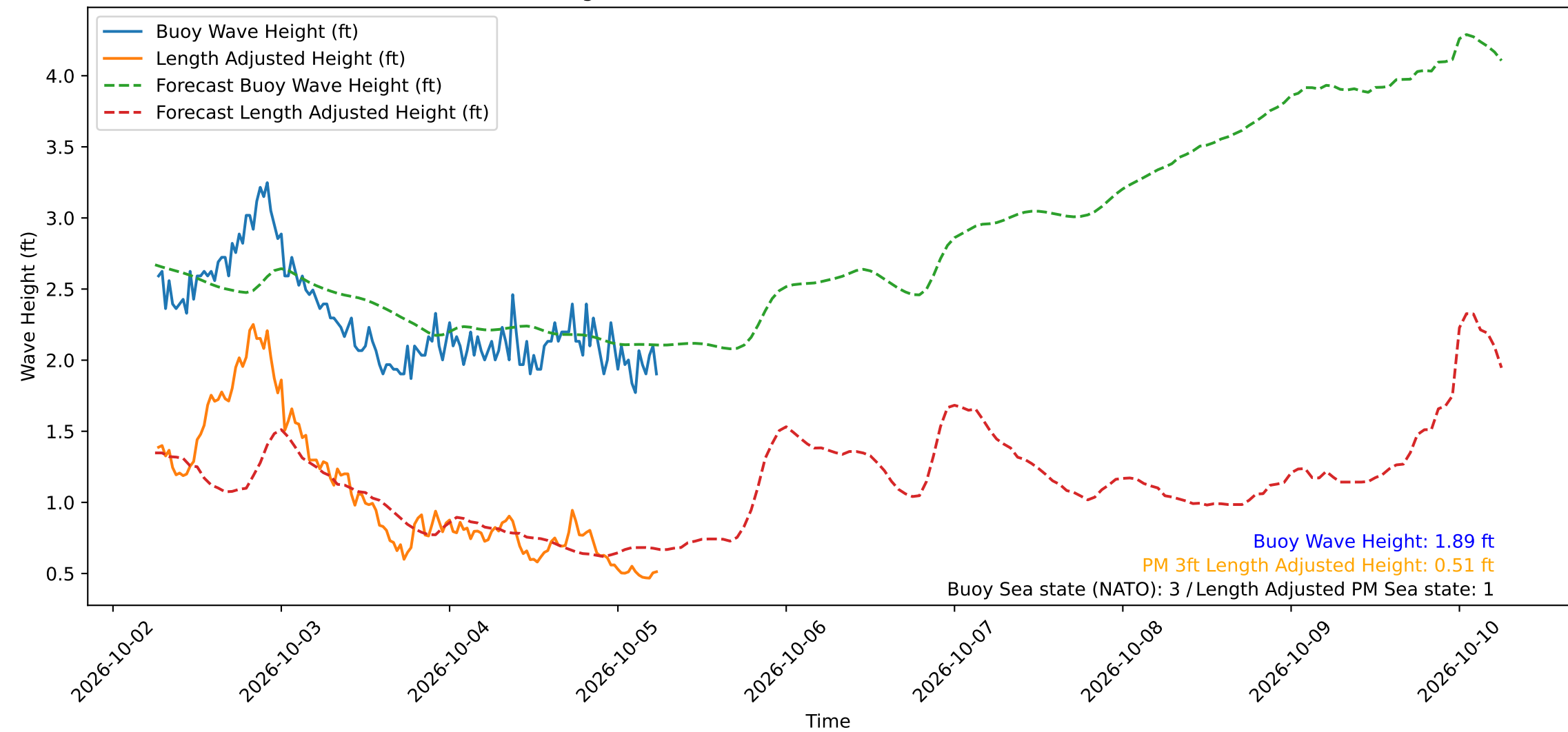
Wave Heights over Time for Red Beach at 2026-10-05 06:10:49
