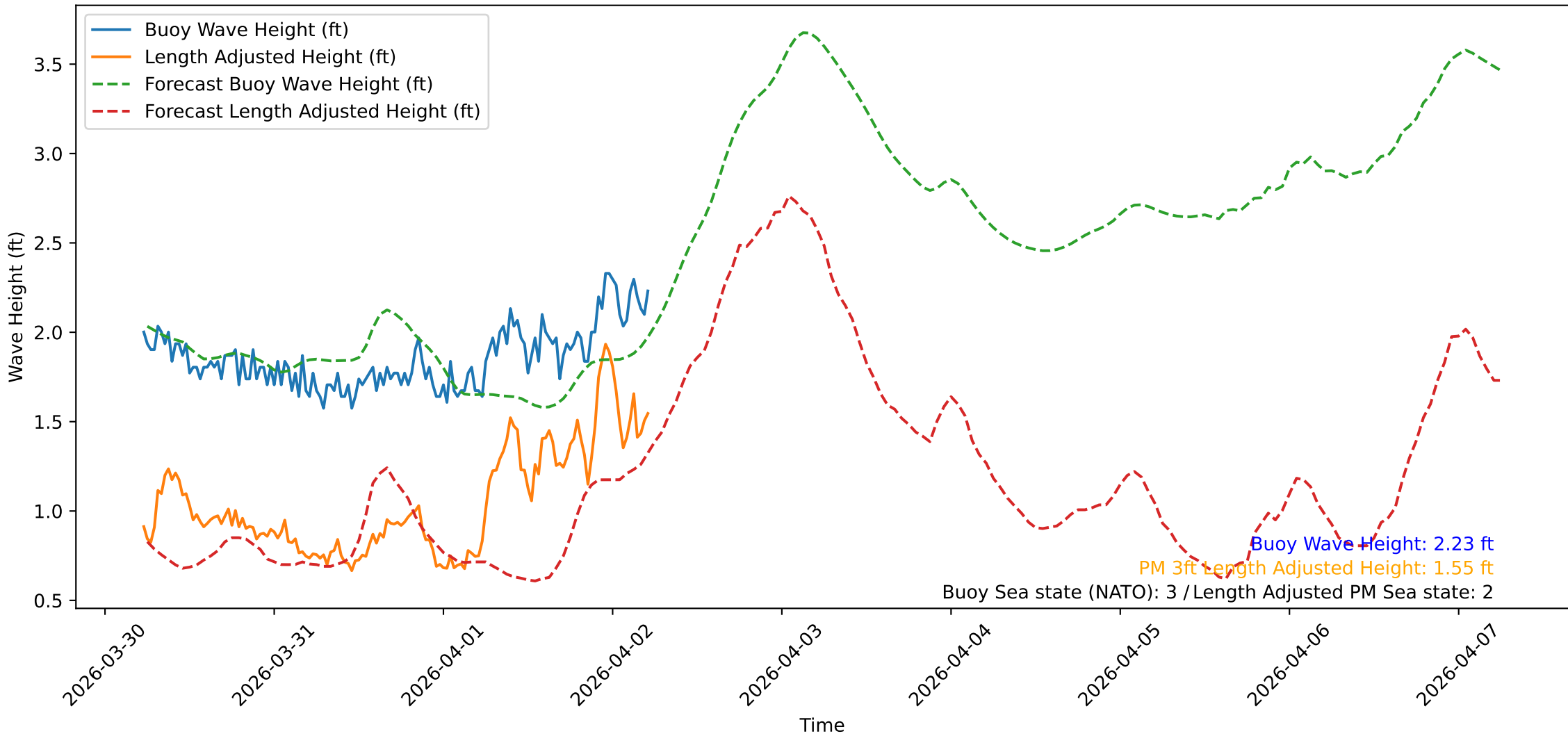
Wave Heights over Time for Oceanside Harbor at 2026-04-02 05:40:31
