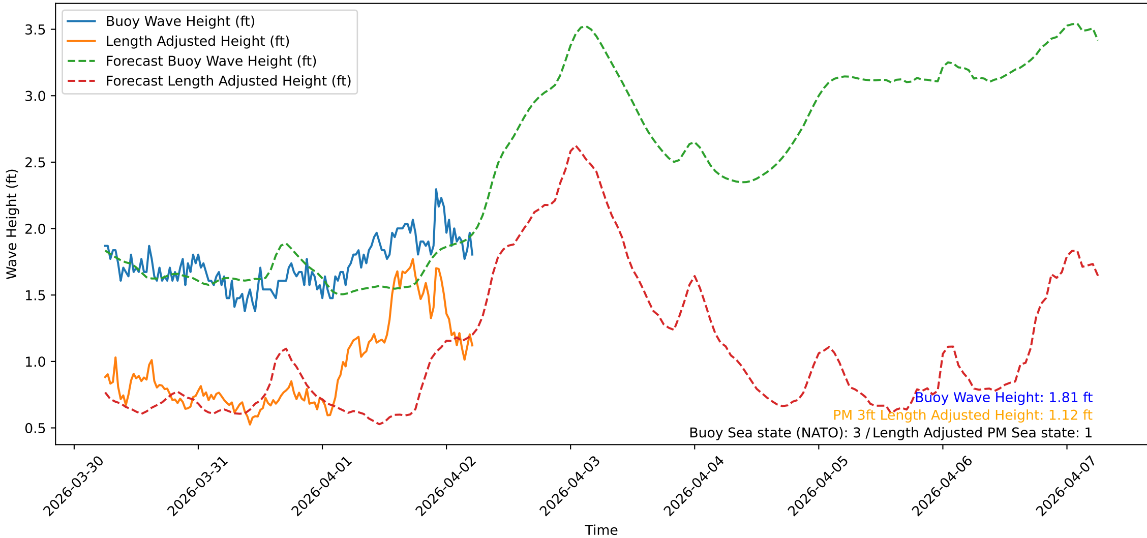
Wave Heights over Time for Red Beach at 2026-04-02 05:40:46
