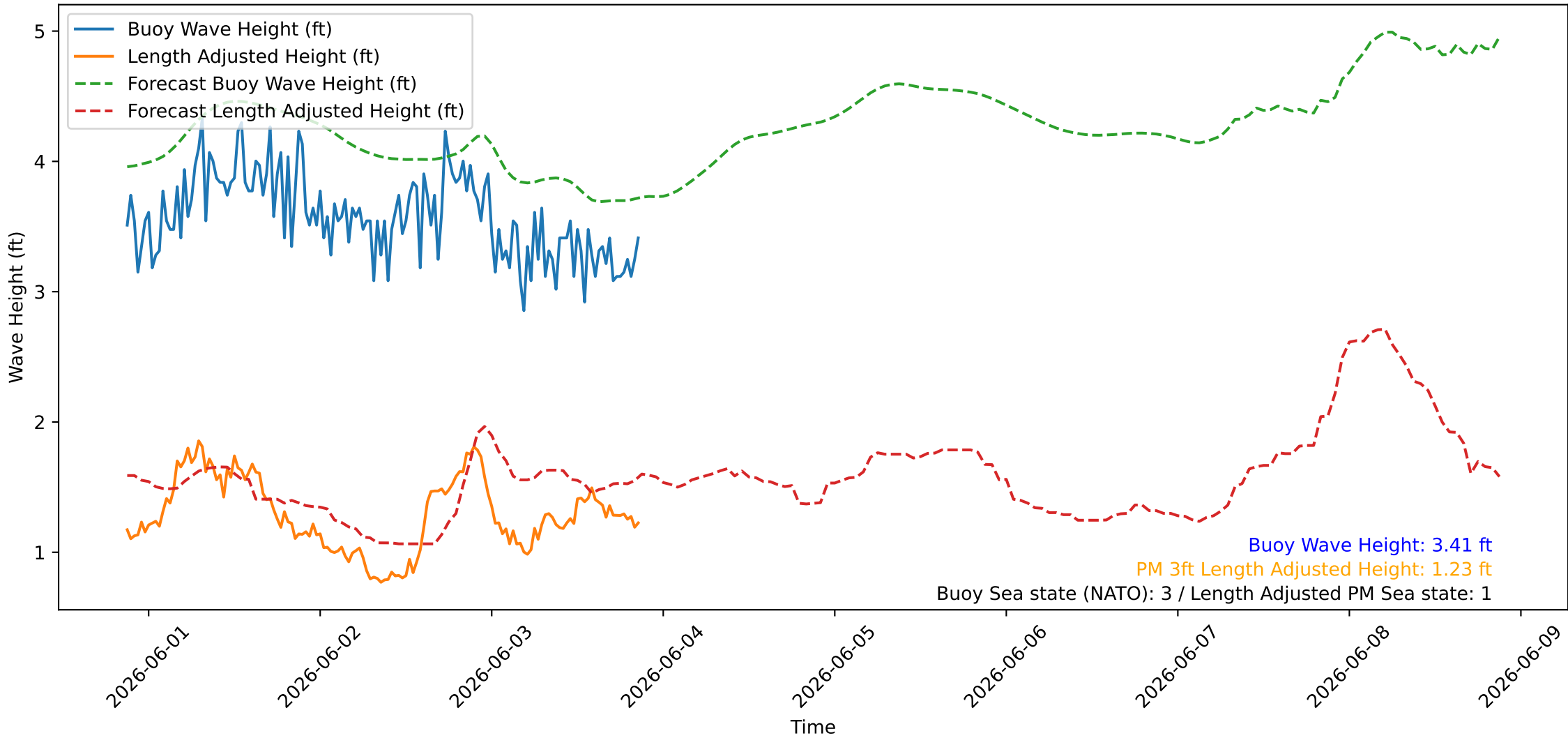
Wave Heights over Time for Green Beach at 2026-06-03 21:11:07
