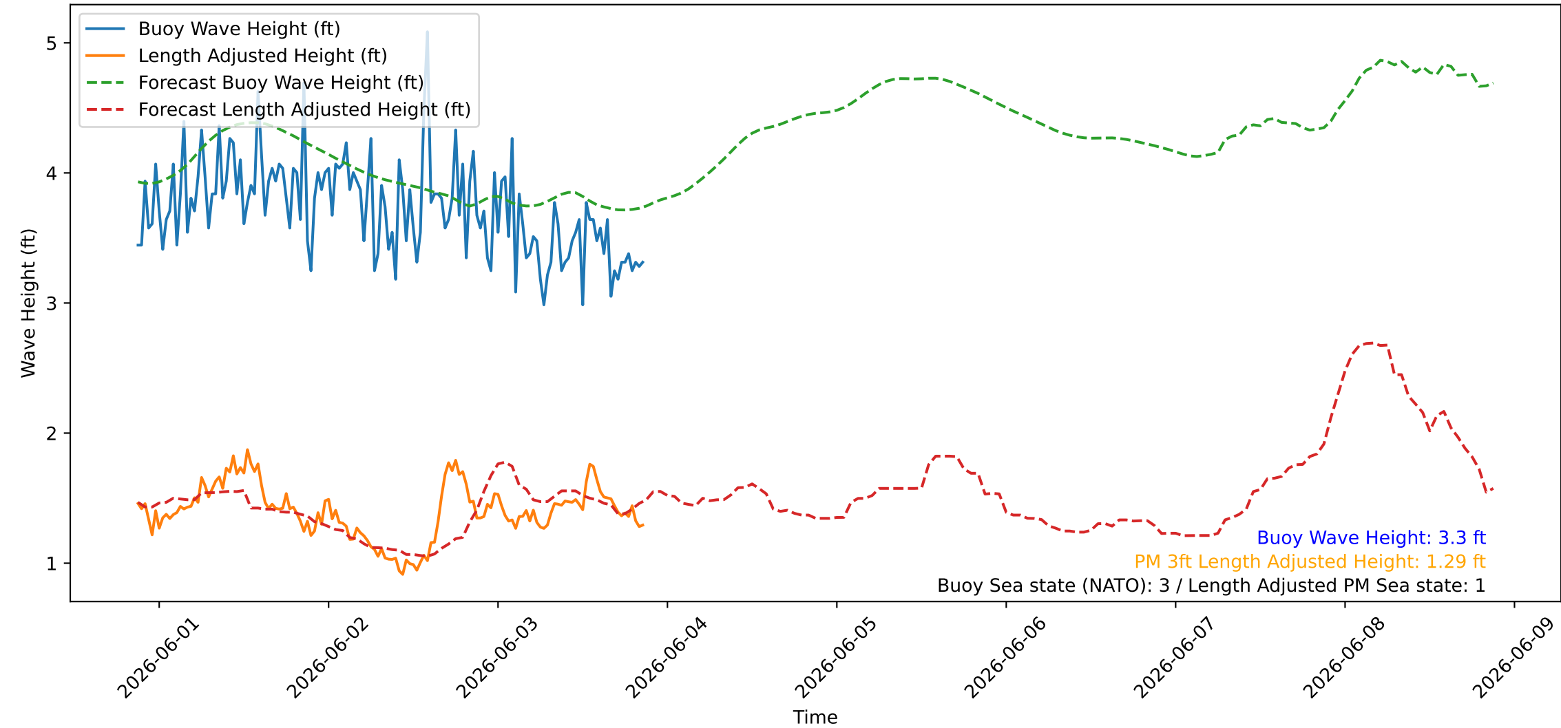
Wave Heights over Time for Oceanside Harbor at 2026-06-03 21:10:25
