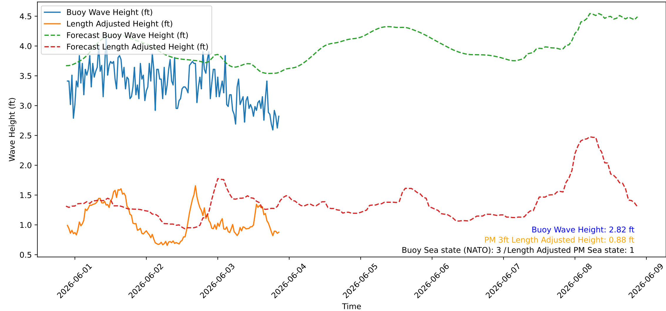
Wave Heights over Time for Red Beach at 2026-06-03 21:10:45
