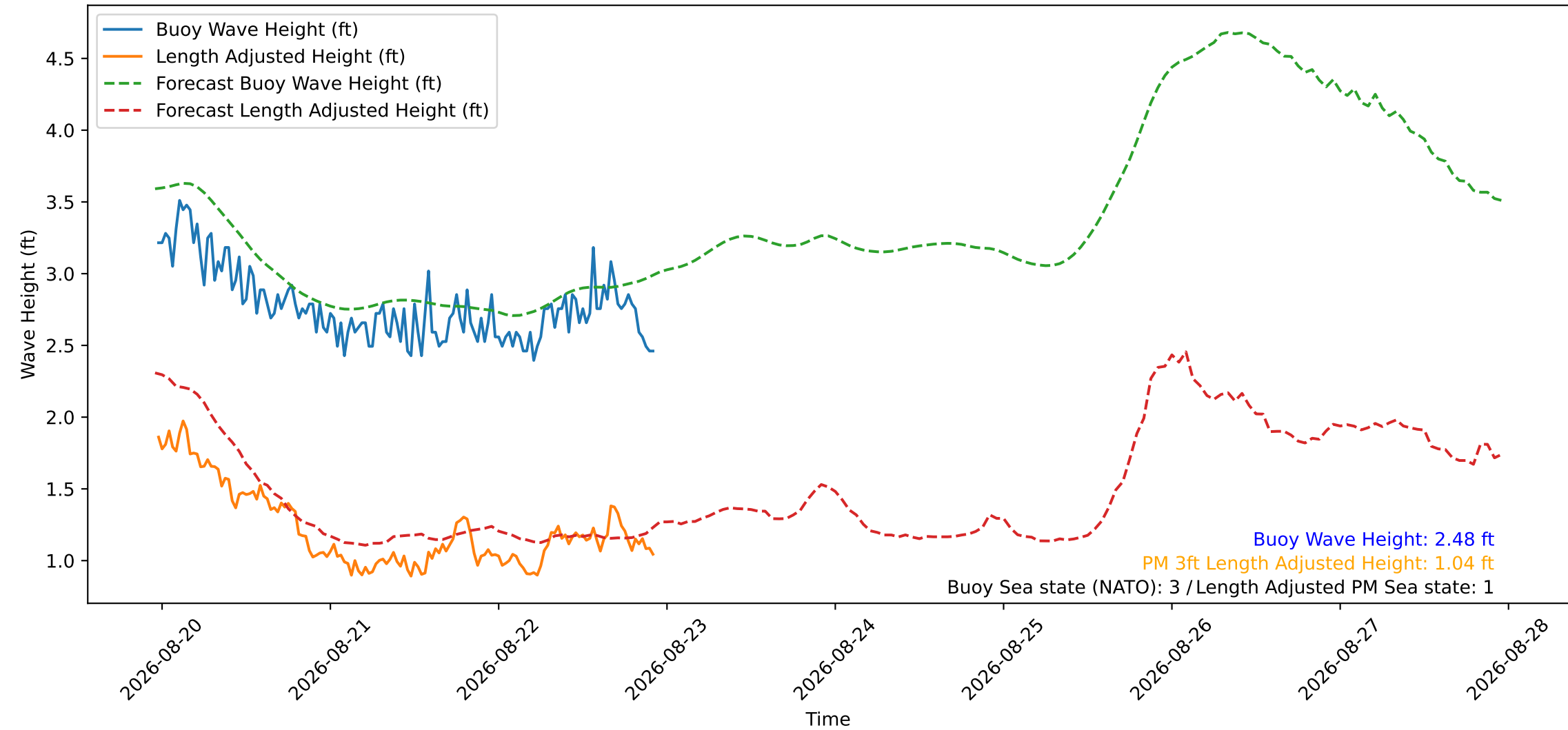
Wave Heights over Time for Green Beach at 2026-08-22 23:01:12
