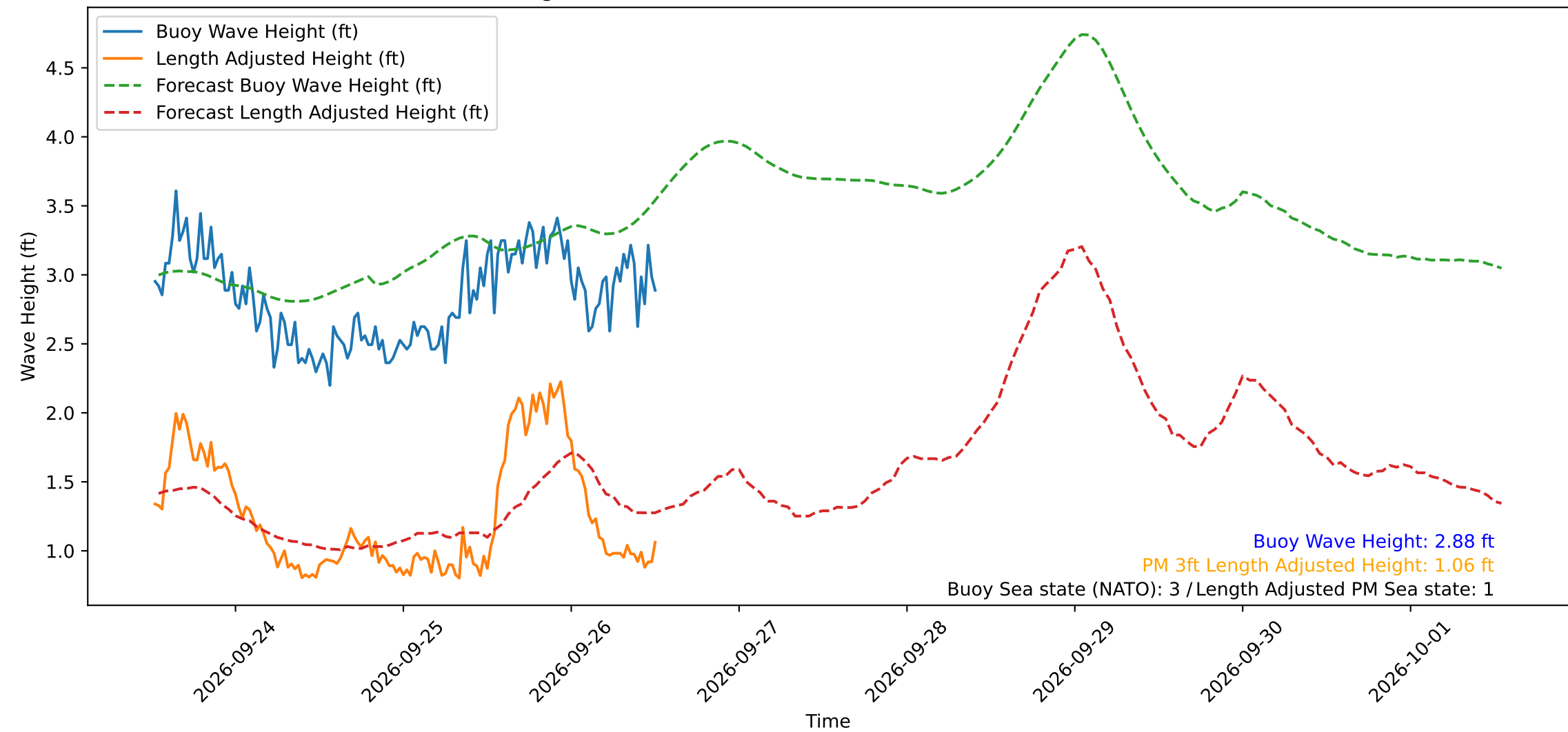
Wave Heights over Time for Oceanside Harbor at 2026-09-26 12:40:30
