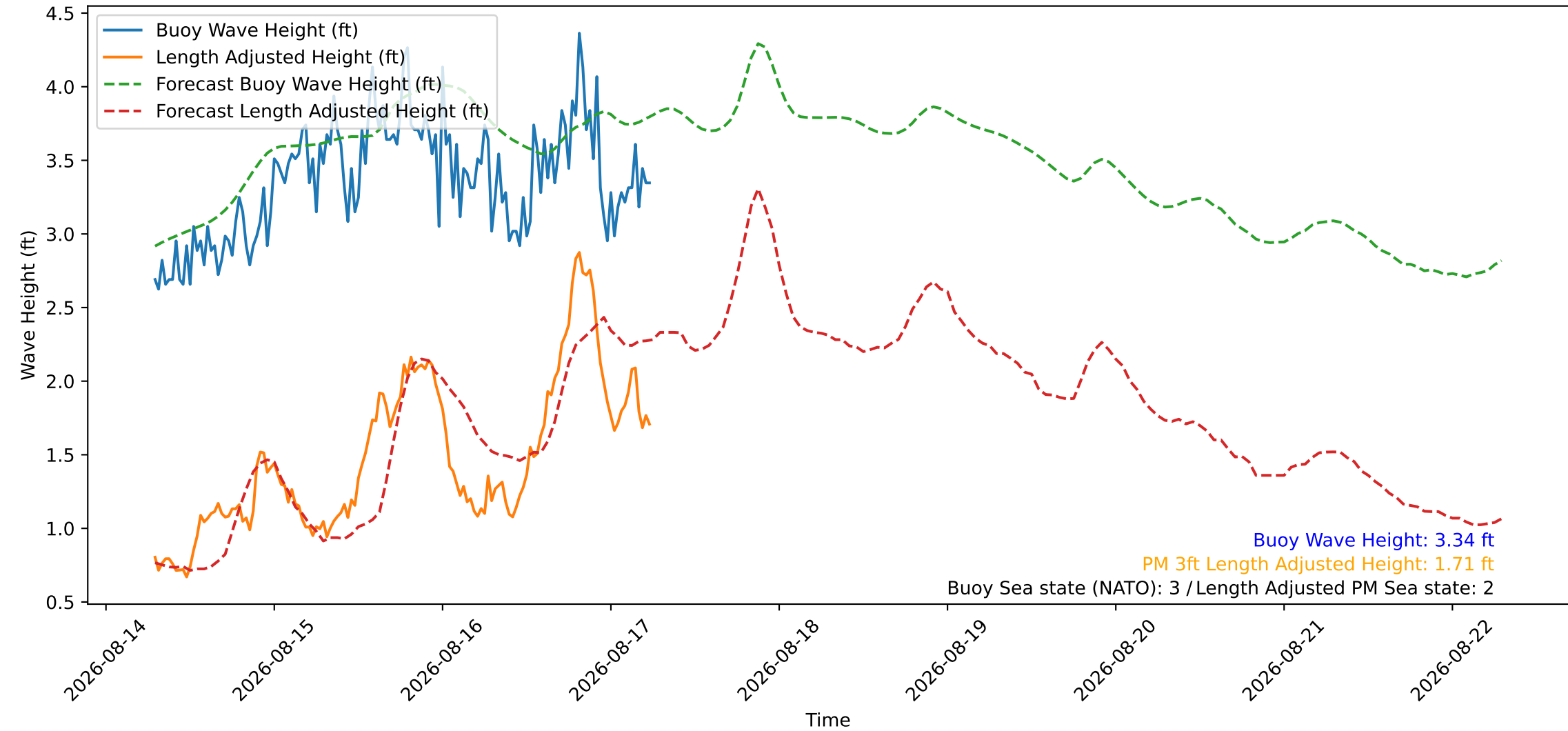
Wave Heights over Time for Green Beach at 2026-08-17 06:51:11
