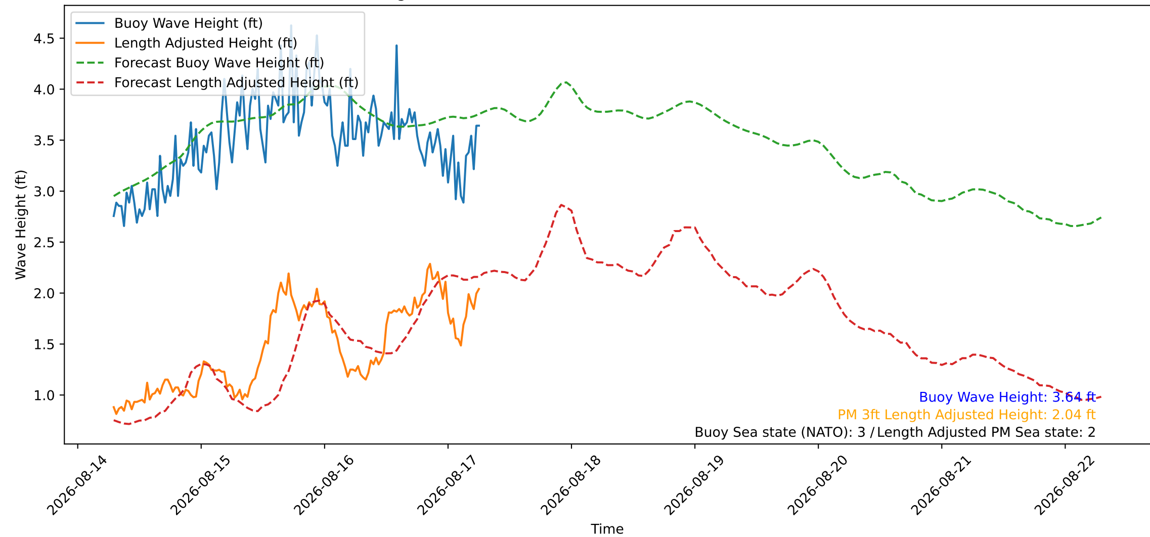
Wave Heights over Time for Oceanside Harbor at 2026-08-17 06:50:26
