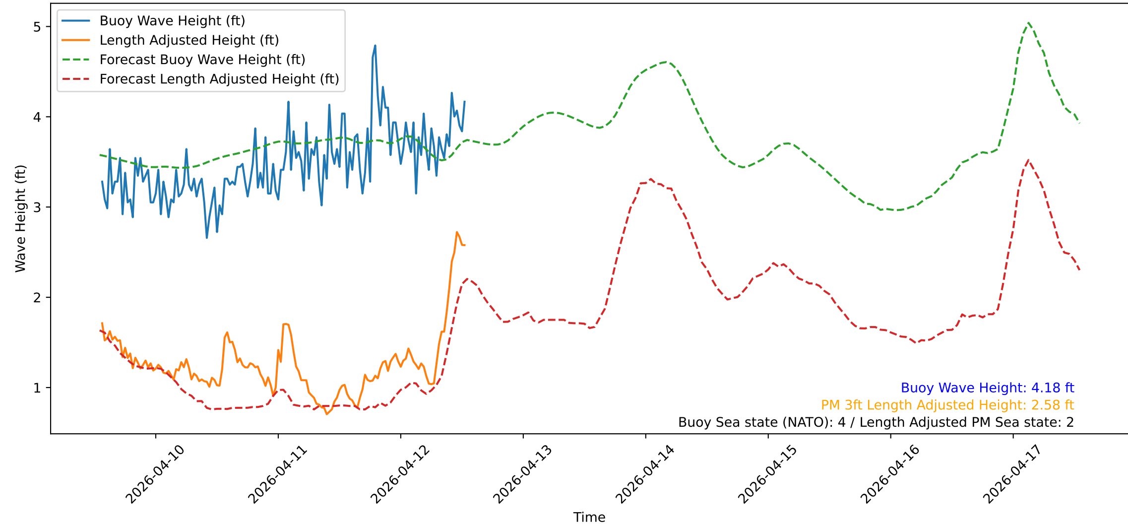
Wave Heights over Time for Oceanside Harbor at 2026-04-12 13:20:31
