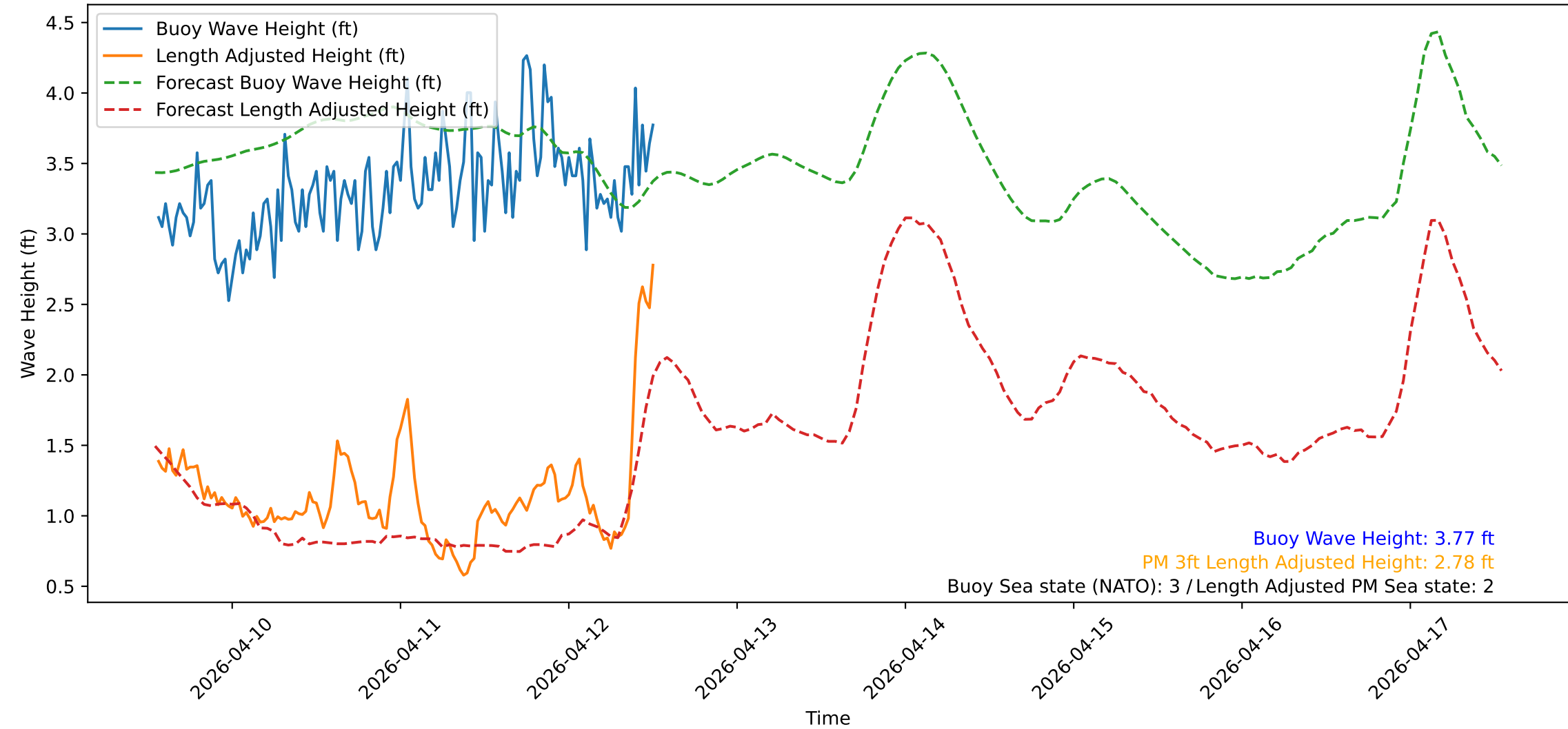
Wave Heights over Time for Red Beach at 2026-04-12 13:20:51
