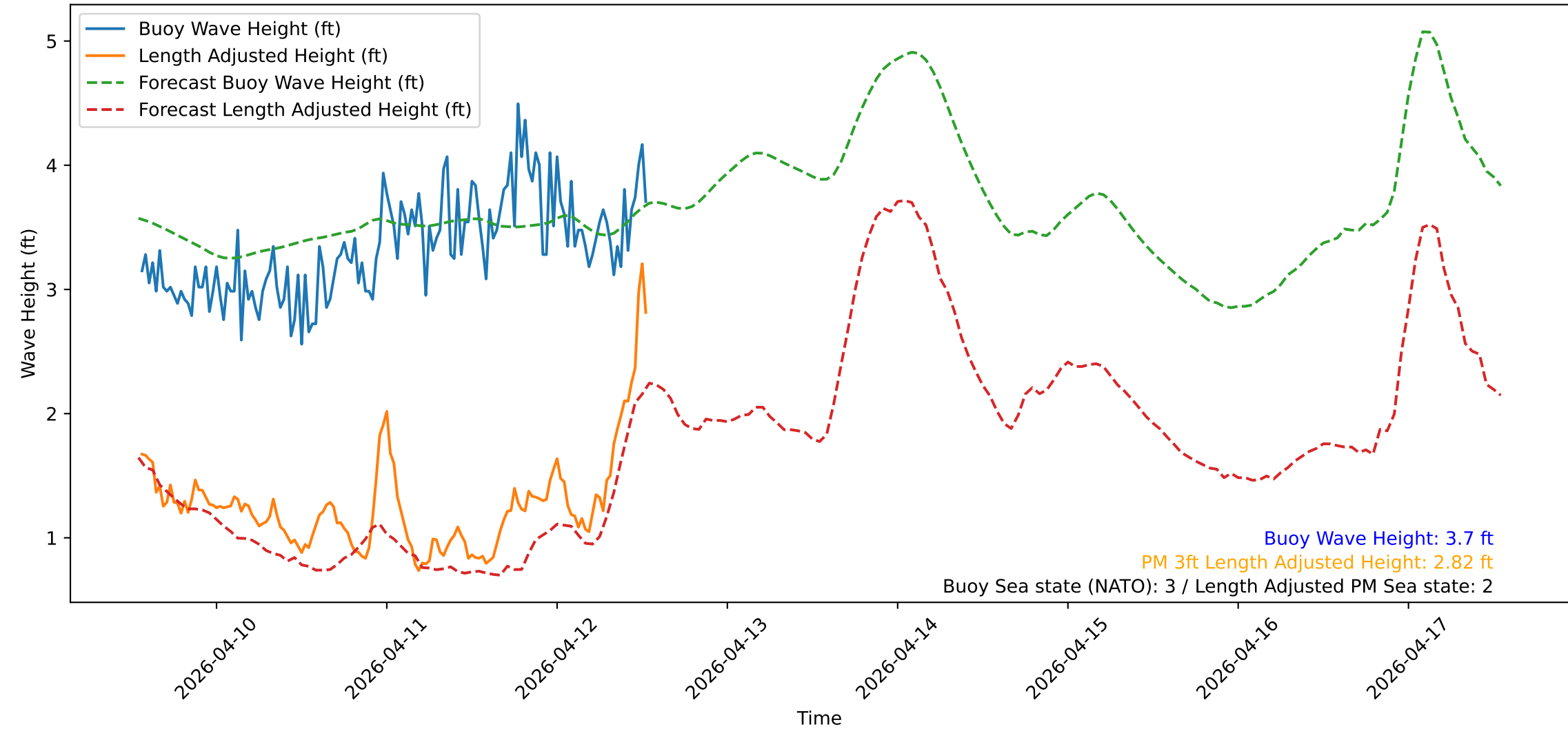
Wave Heights over Time for Green Beach at 2026-04-12 13:21:13
