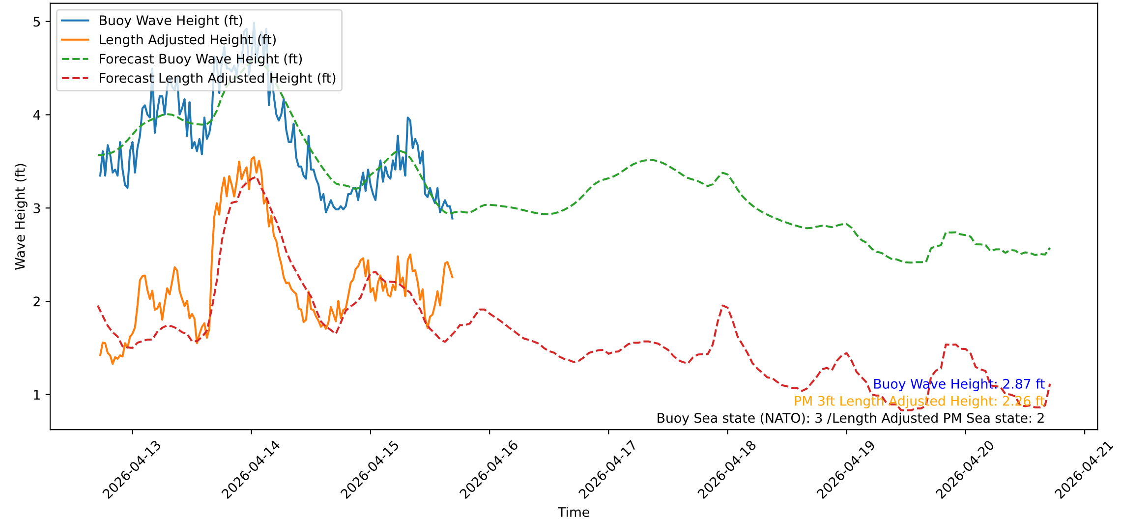
Wave Heights over Time for Green Beach at 2026-04-15 17:21:14
