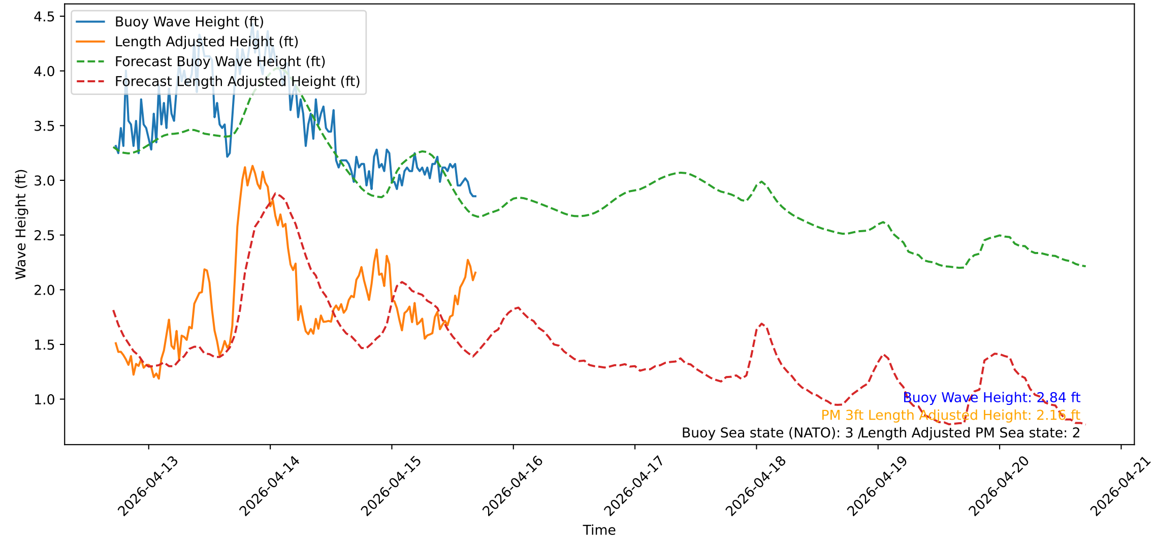
Wave Heights over Time for Red Beach at 2026-04-15 17:20:52
