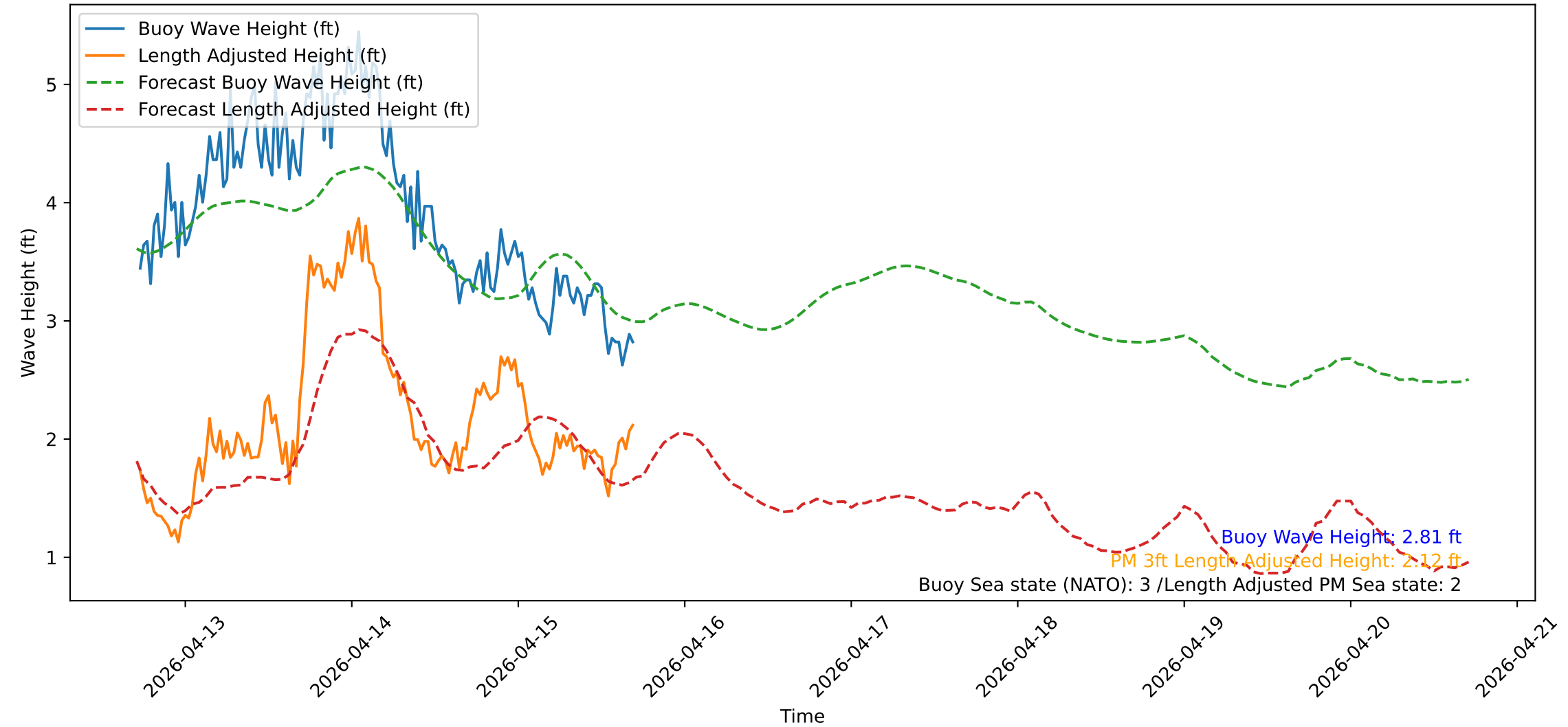
Wave Heights over Time for Oceanside Harbor at 2026-04-15 17:20:31
