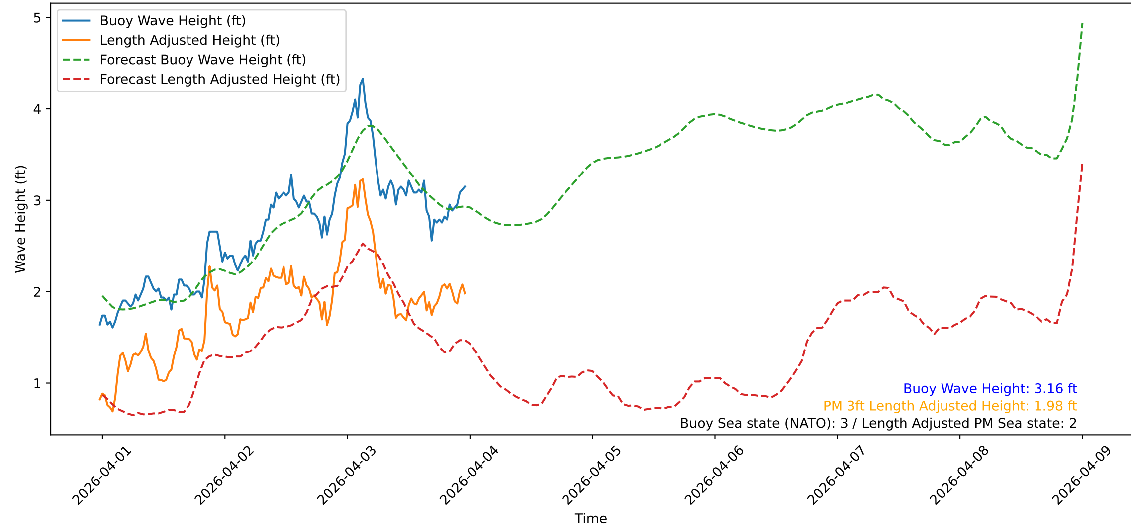
Wave Heights over Time for Green Beach at 2026-04-03 23:41:15
