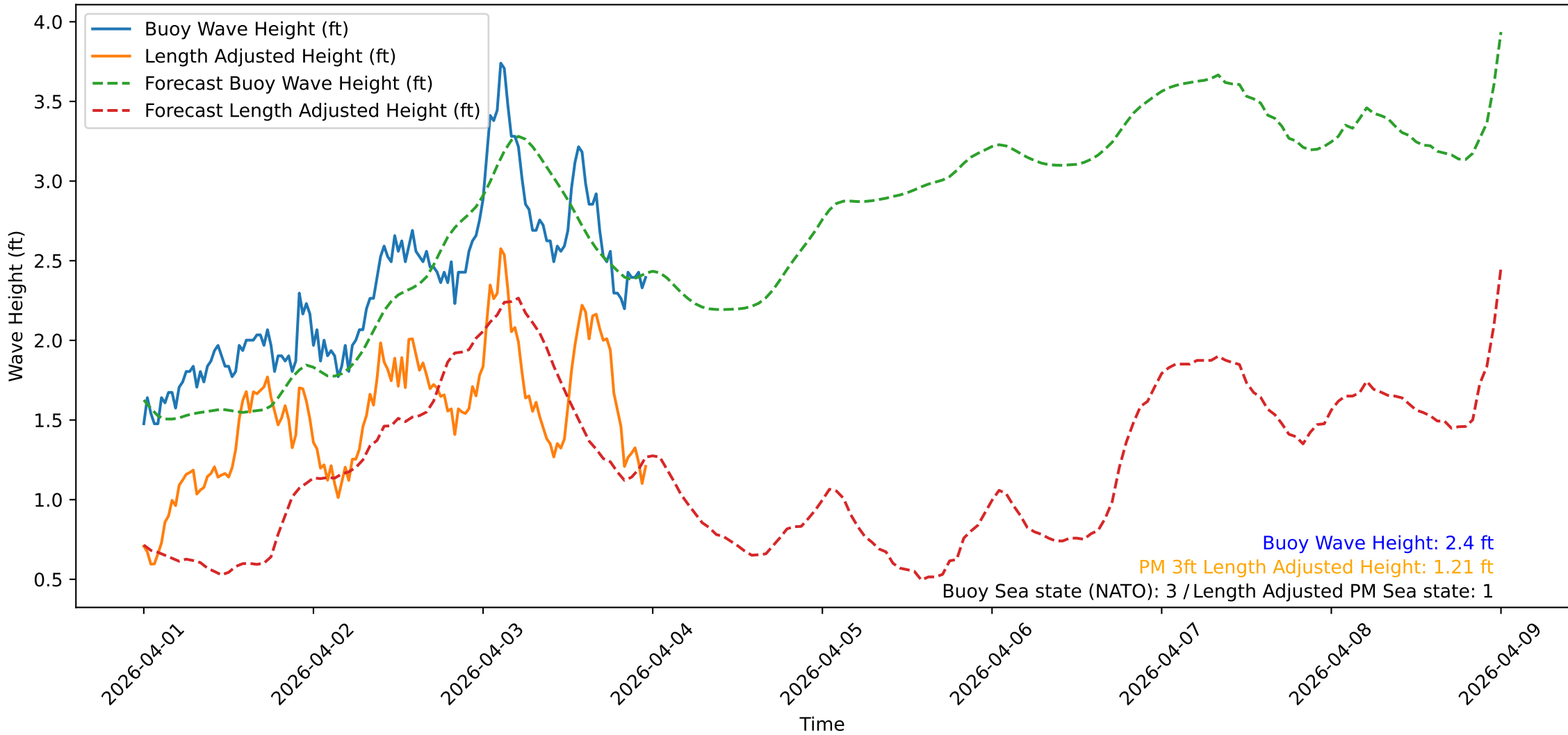
Wave Heights over Time for Red Beach at 2026-04-03 23:40:50
