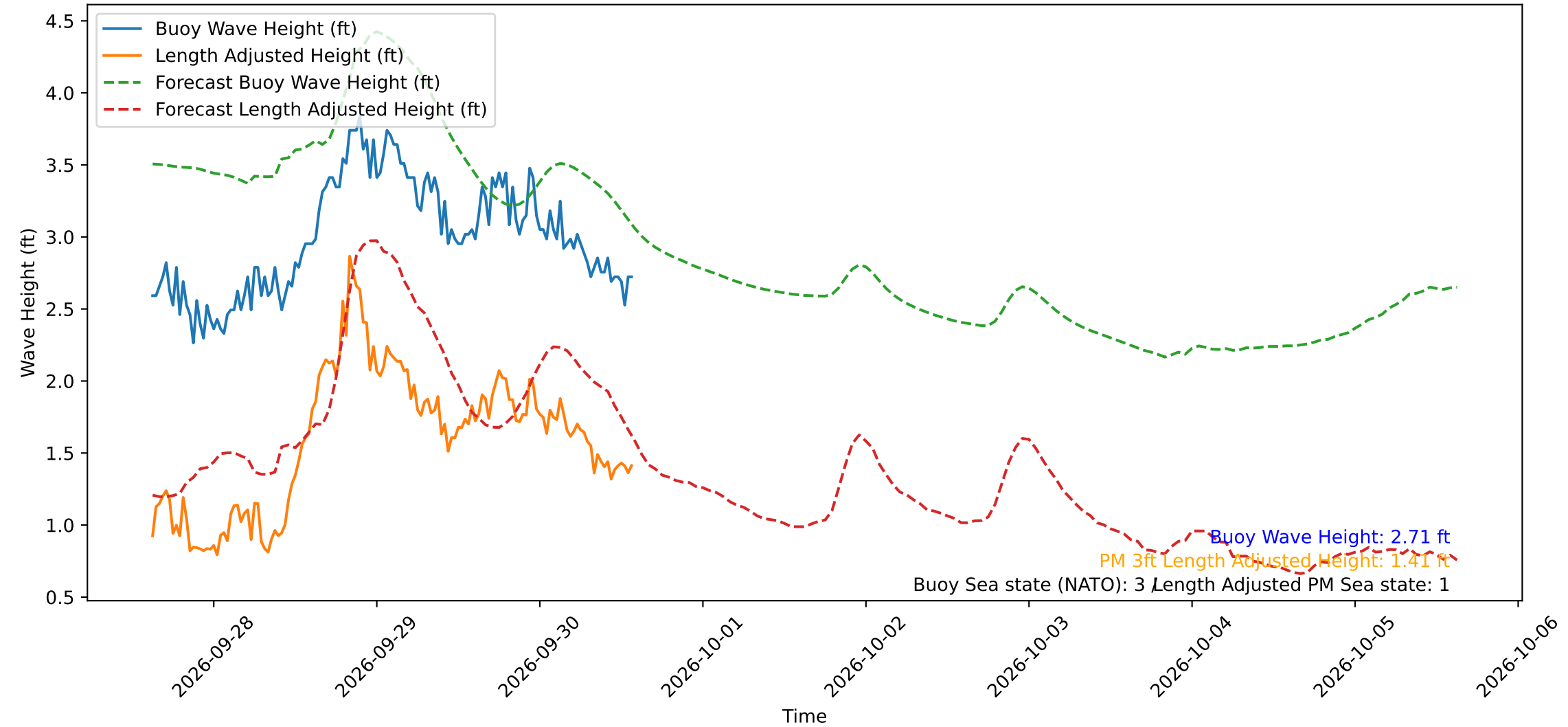
Wave Heights over Time for Red Beach at 2026-09-30 14:30:50
