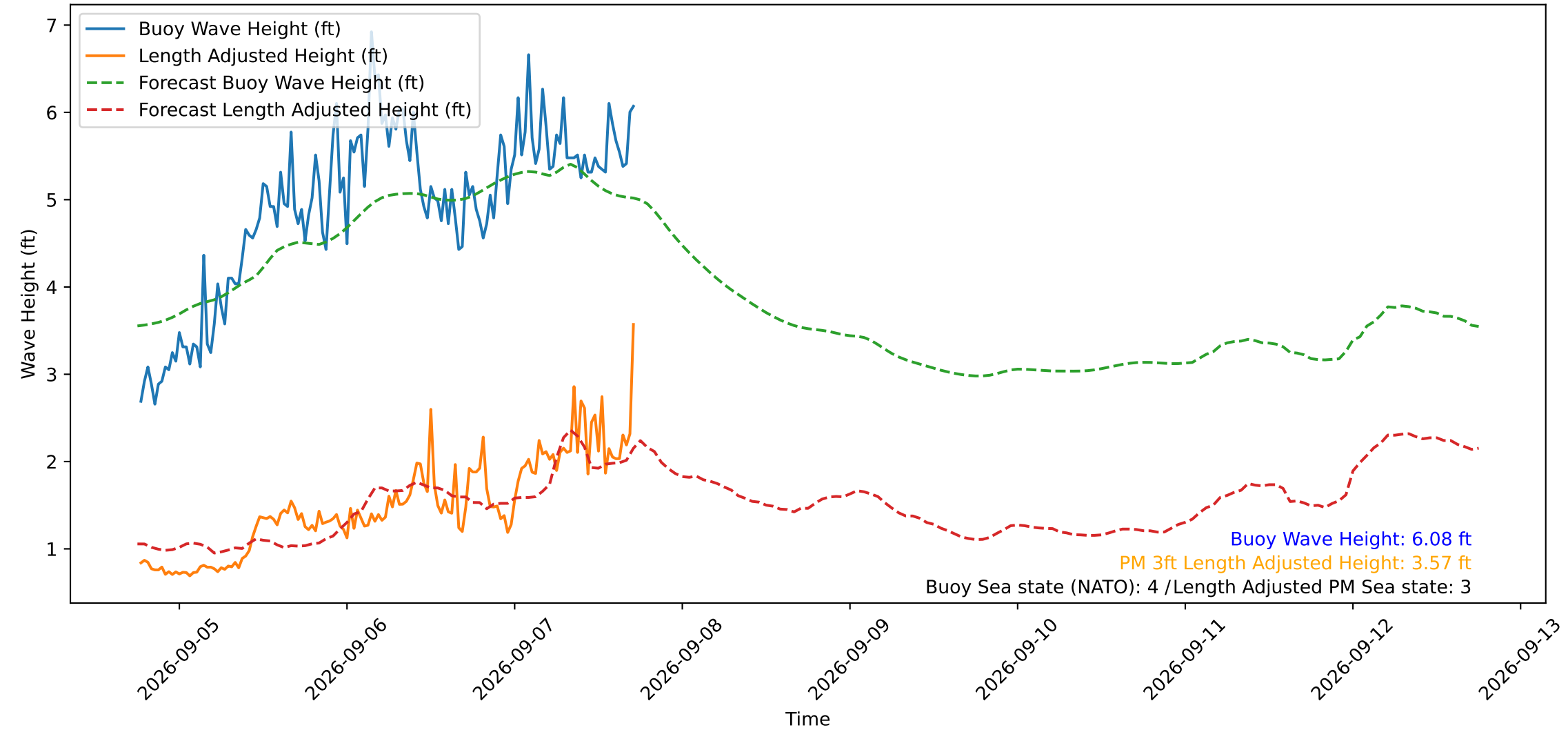
Wave Heights over Time for Red Beach at 2026-09-07 18:00:49
