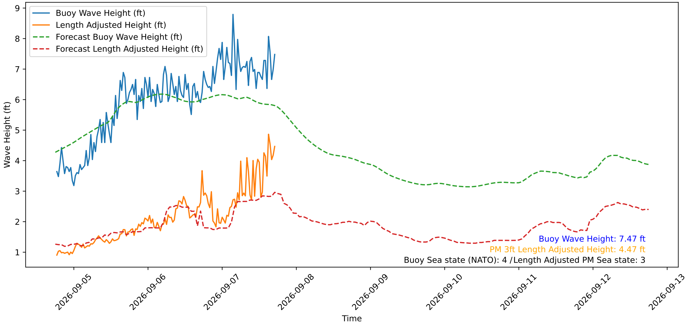
Wave Heights over Time for Green Beach at 2026-09-07 18:01:11
