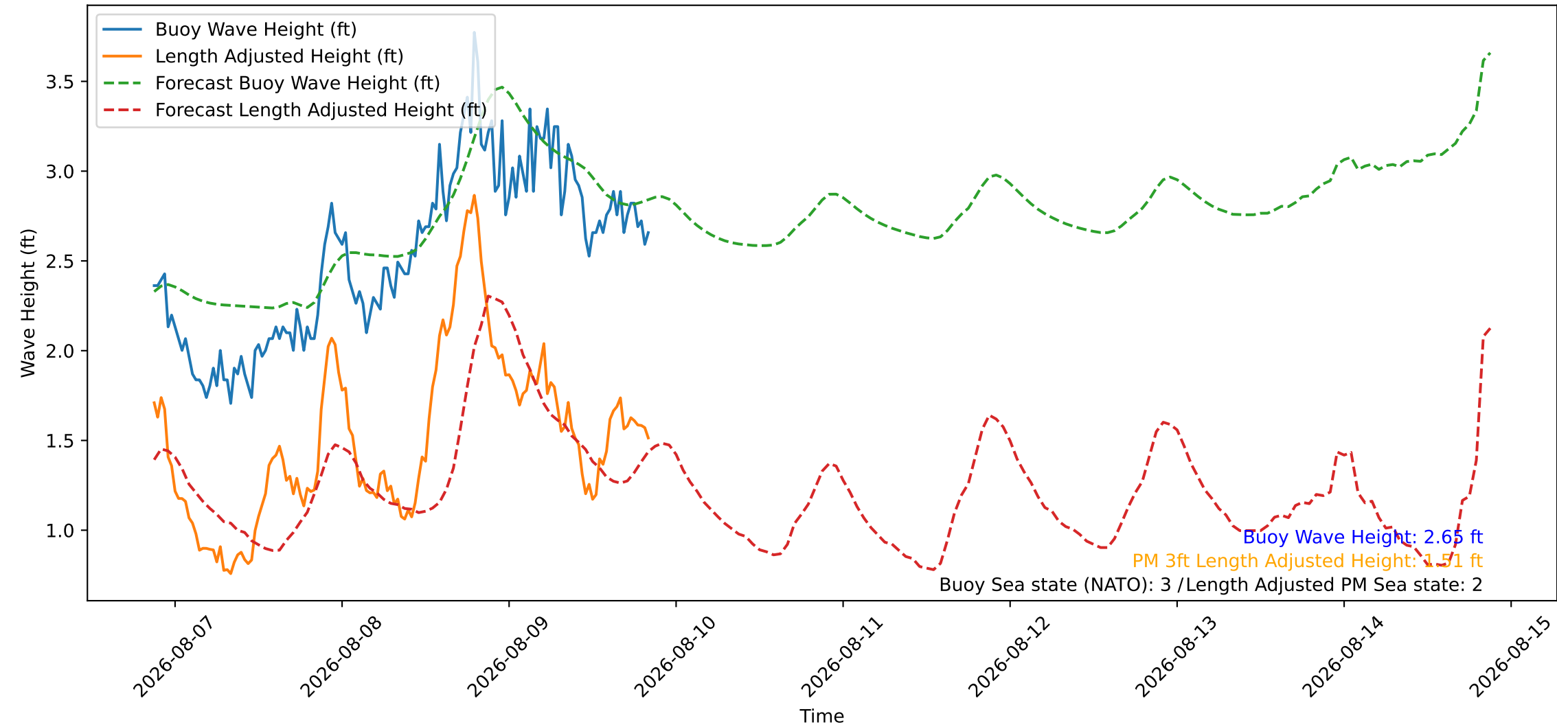
Wave Heights over Time for Green Beach at 2026-08-09 21:01:09
