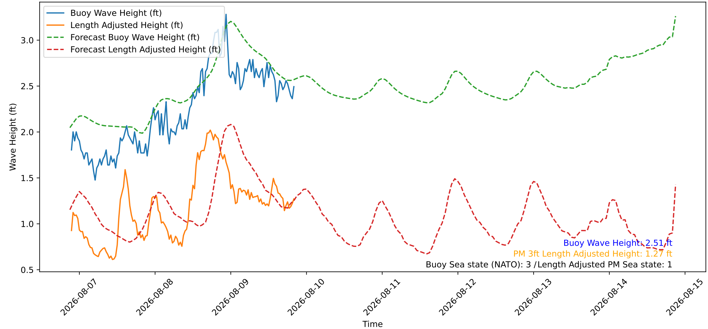
Wave Heights over Time for Red Beach at 2026-08-09 21:00:46
