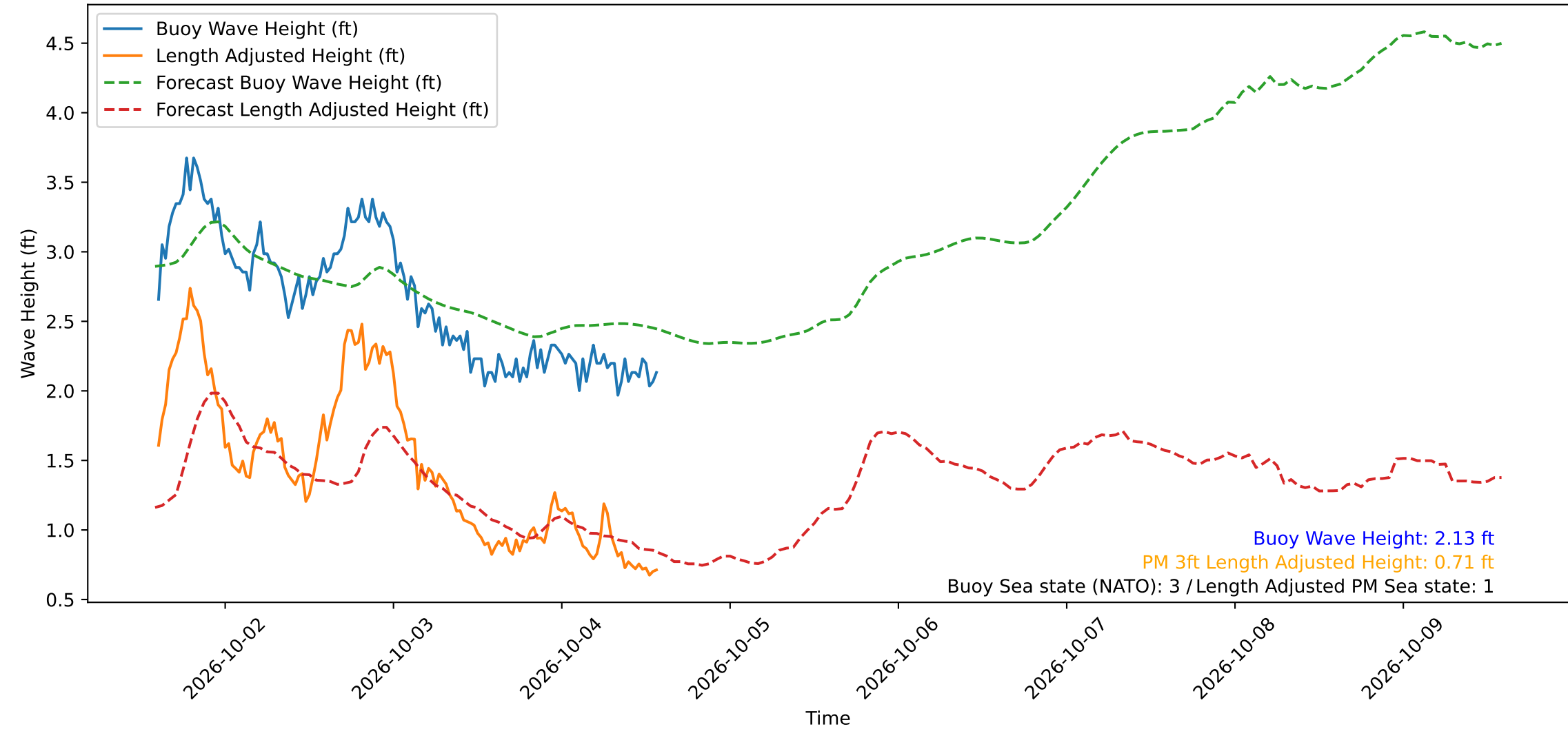
Wave Heights over Time for Green Beach at 2026-10-04 14:21:15
