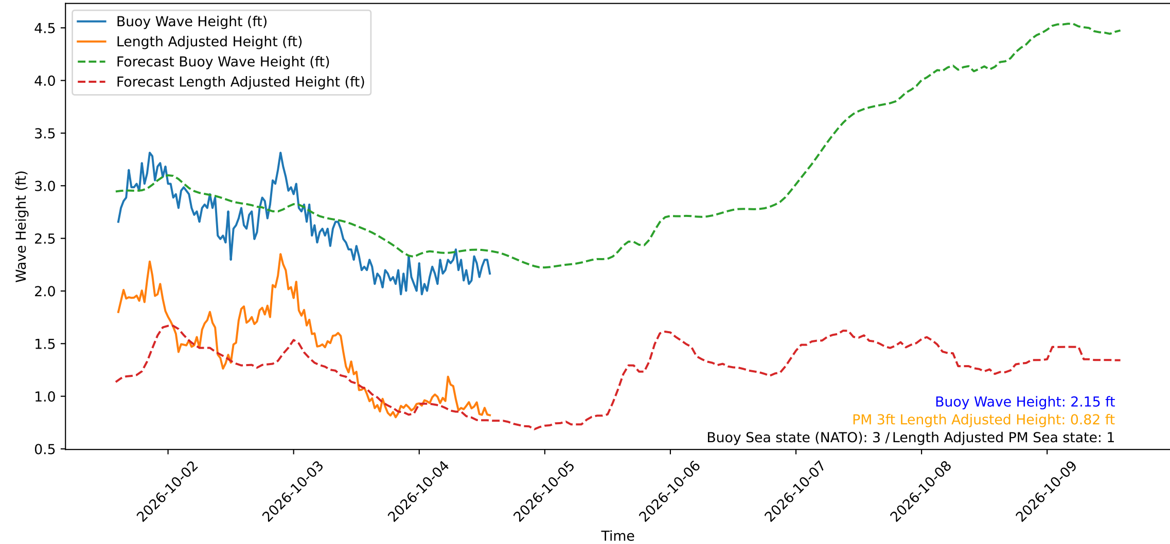
Wave Heights over Time for Oceanside Harbor at 2026-10-04 14:20:30
