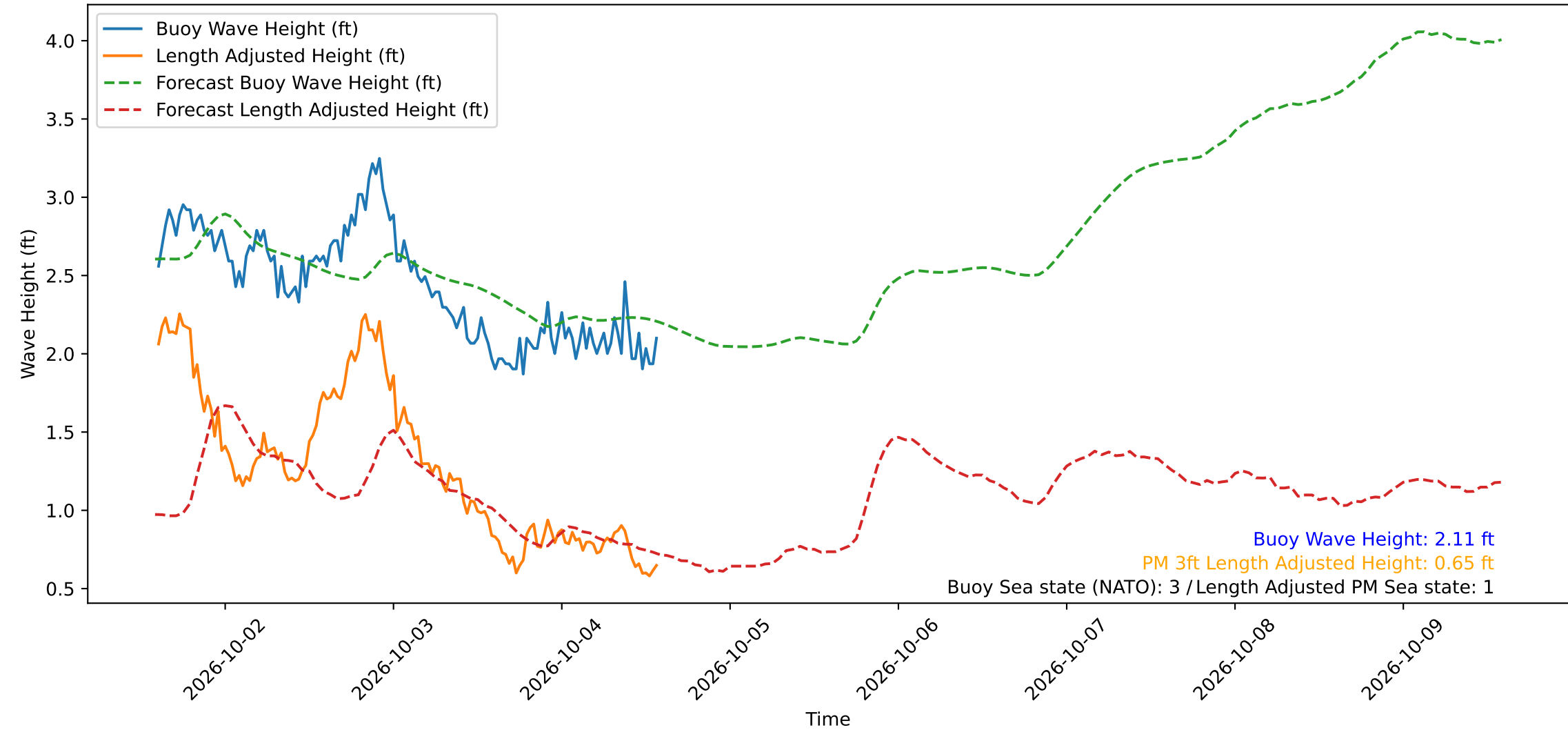
Wave Heights over Time for Red Beach at 2026-10-04 14:20:51
