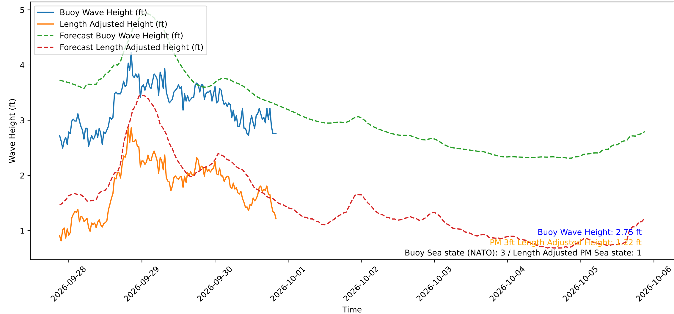
Wave Heights over Time for Oceanside Harbor at 2026-09-30 20:50:29
