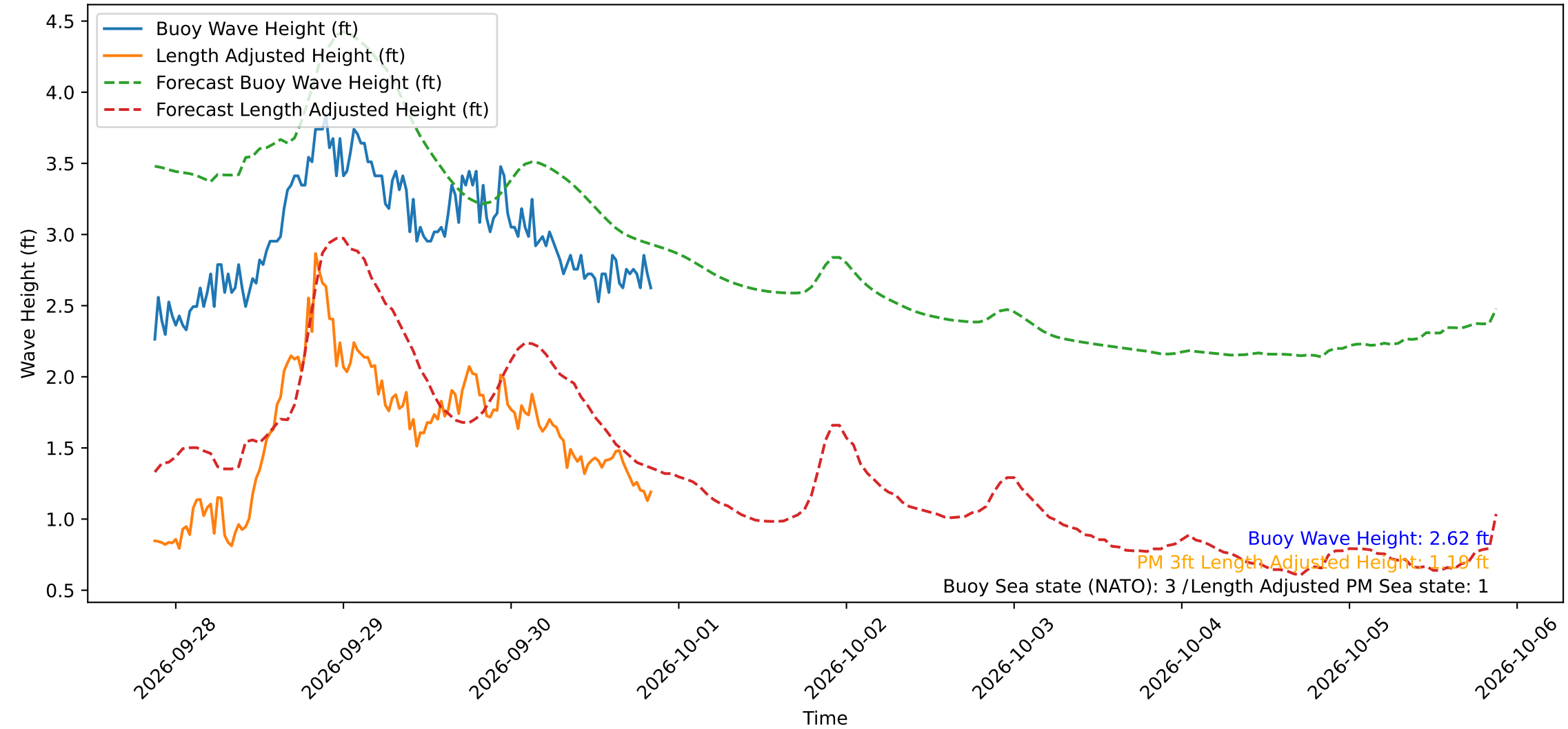
Wave Heights over Time for Red Beach at 2026-09-30 20:50:50
