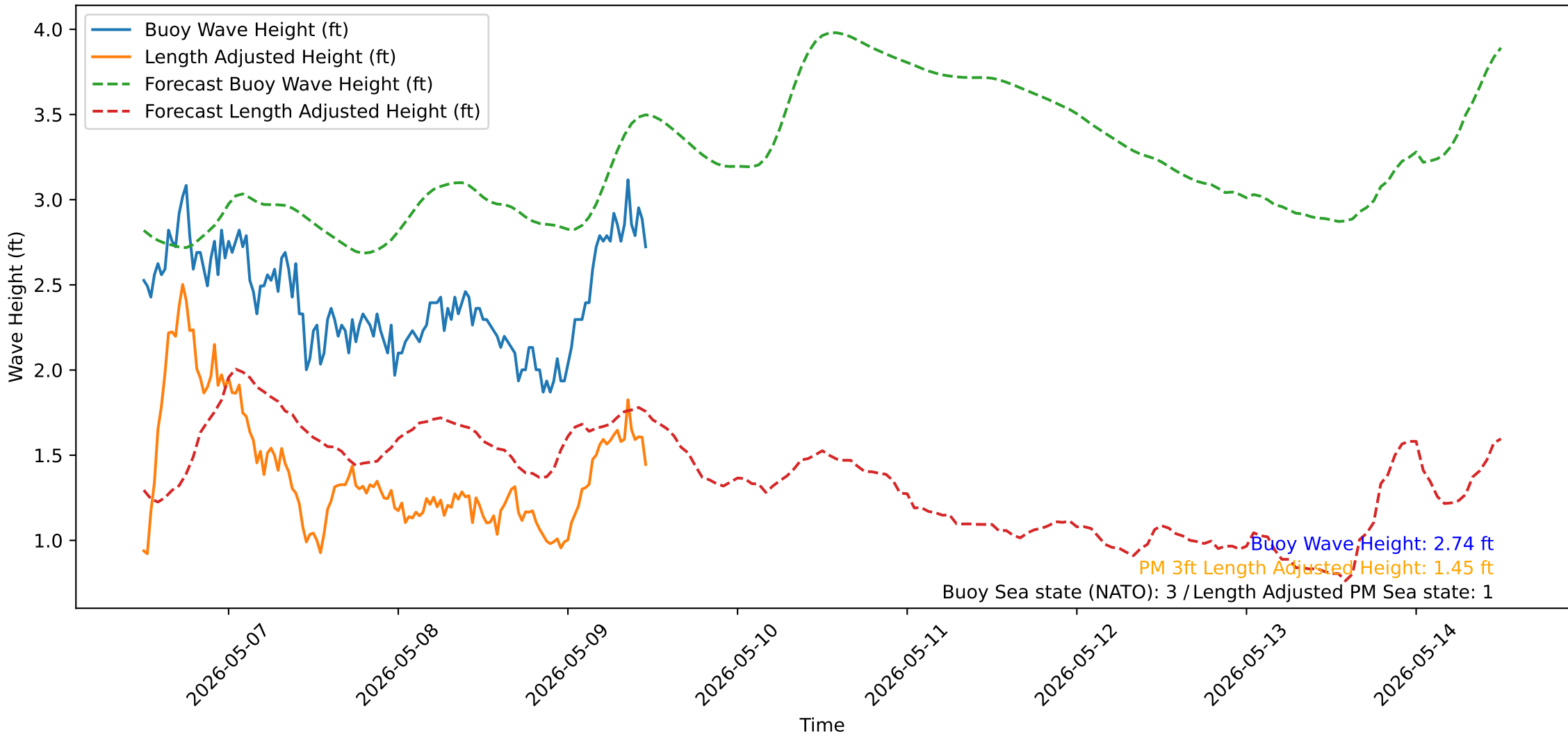
Wave Heights over Time for Oceanside Harbor at 2026-05-09 11:50:31
