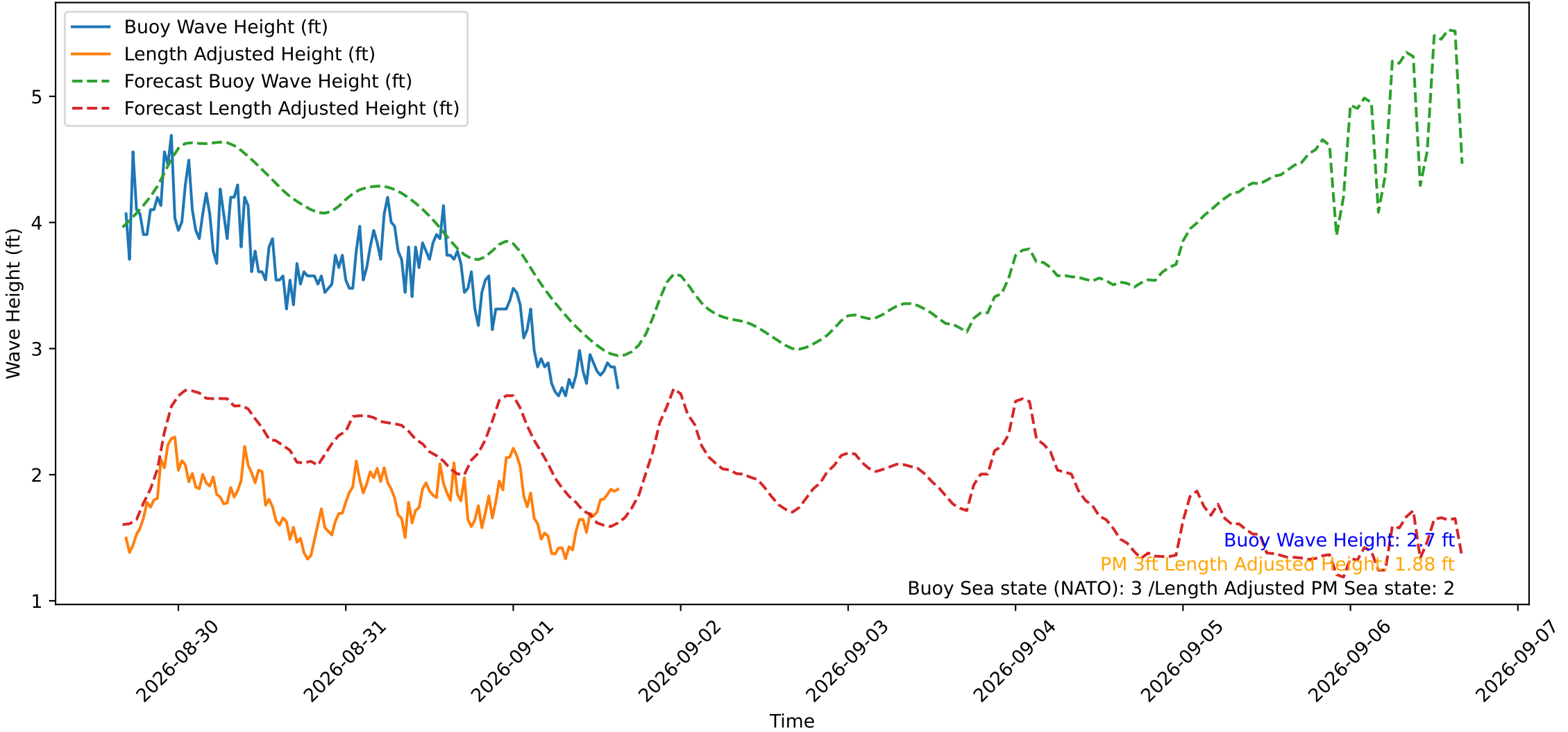
Wave Heights over Time for Red Beach at 2026-09-01 16:00:49
