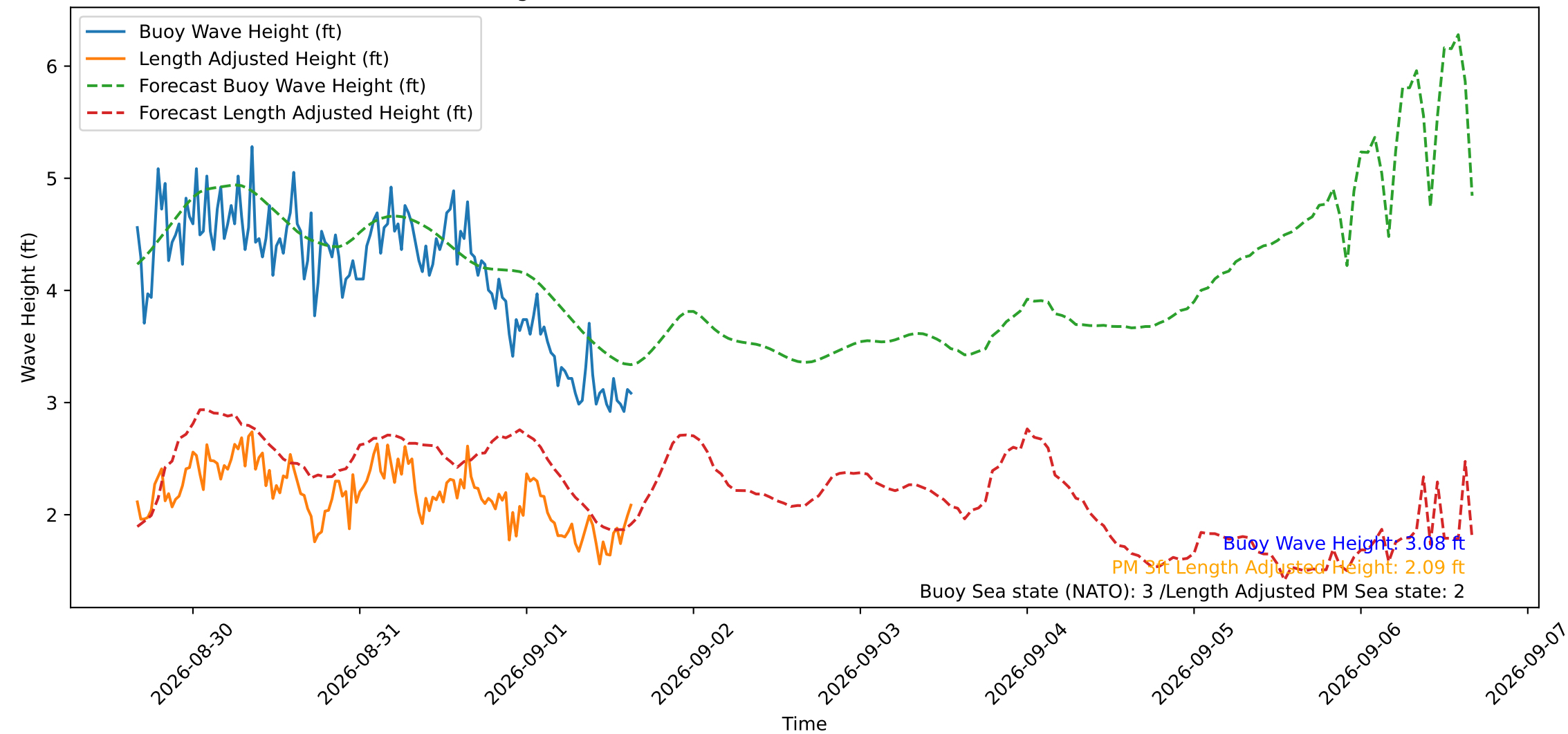
Wave Heights over Time for Oceanside Harbor at 2026-09-01 16:00:29
