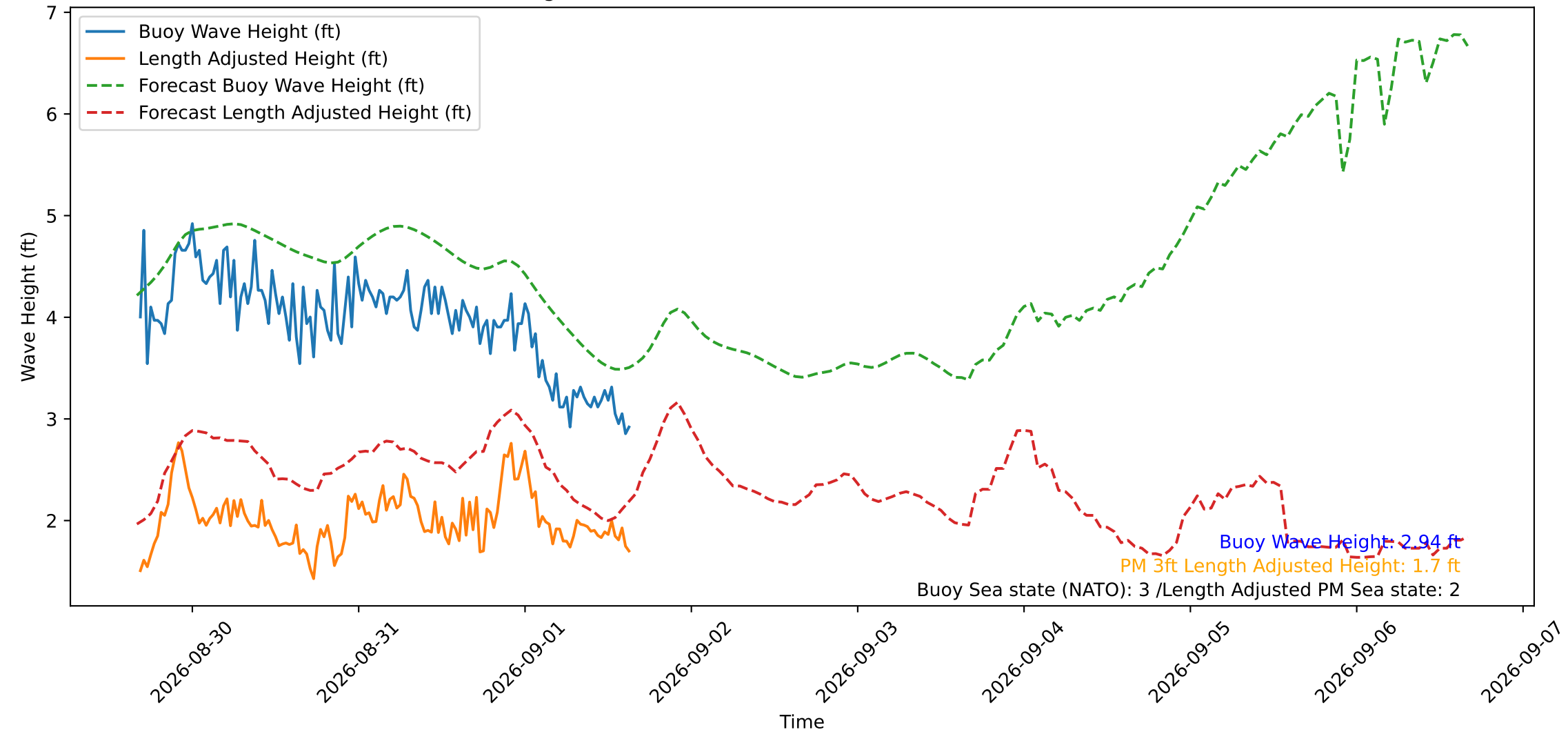
Wave Heights over Time for Green Beach at 2026-09-01 16:01:11
