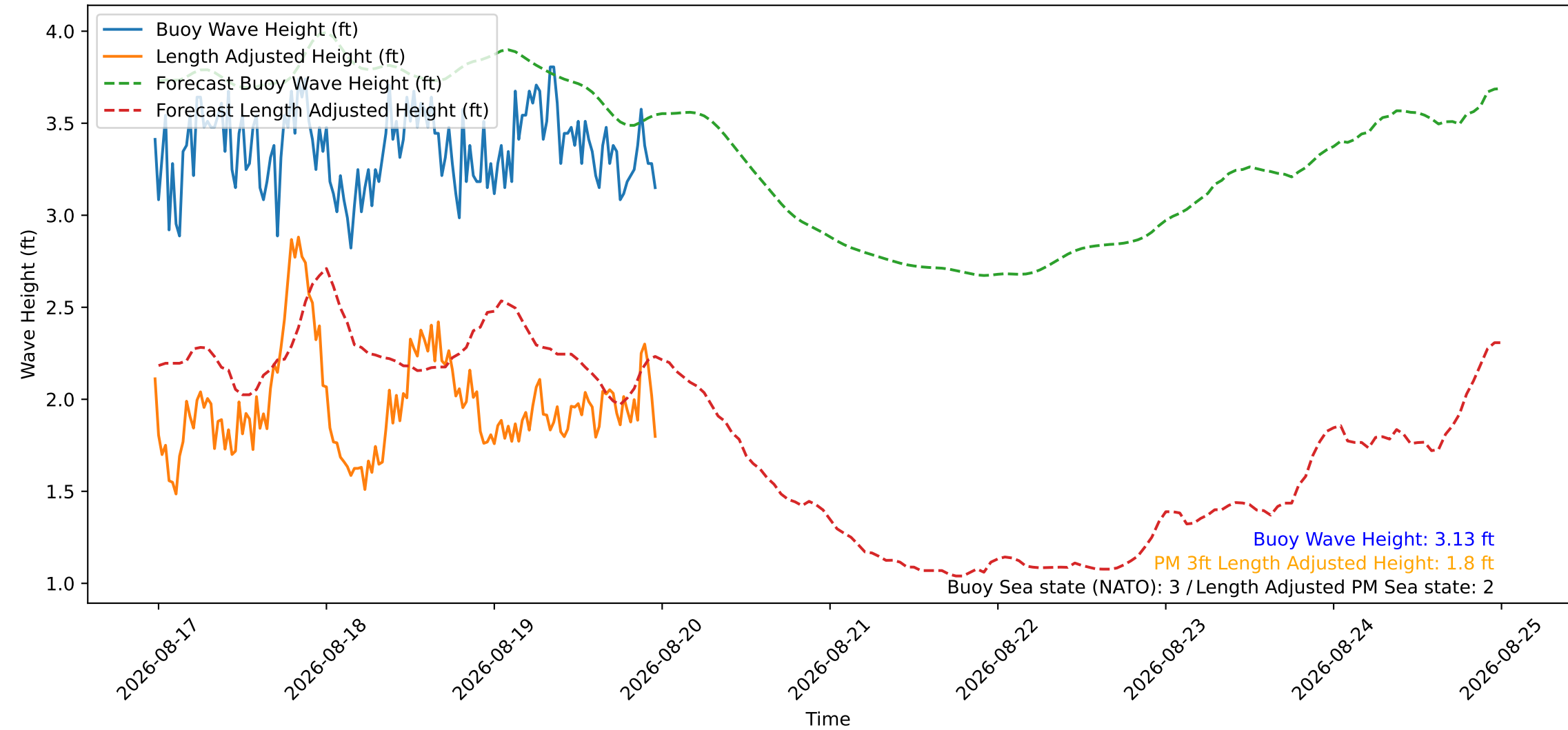
Wave Heights over Time for Oceanside Harbor at 2026-08-19 23:40:26
