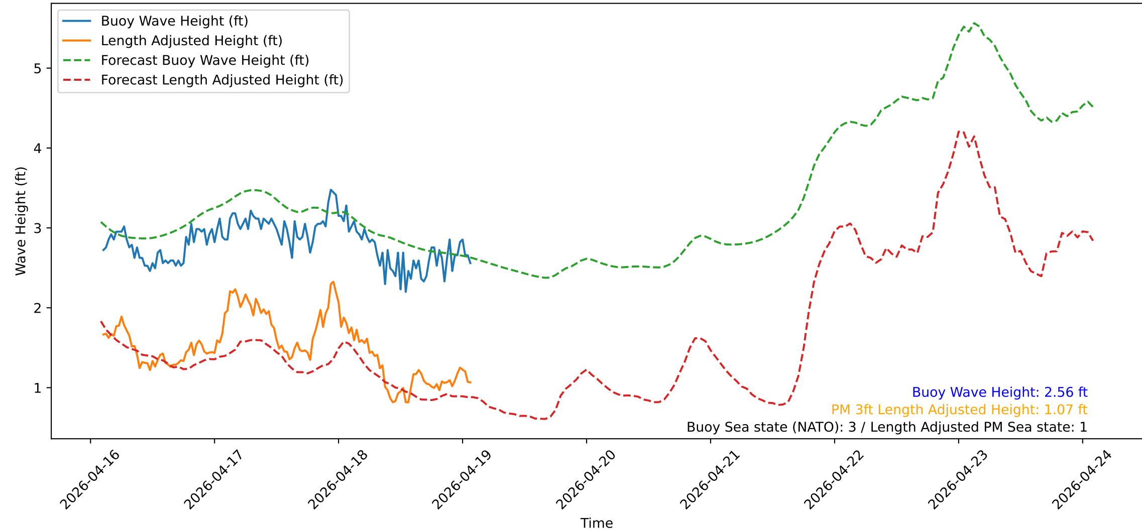
Wave Heights over Time for Green Beach at 2026-04-19 02:21:13
