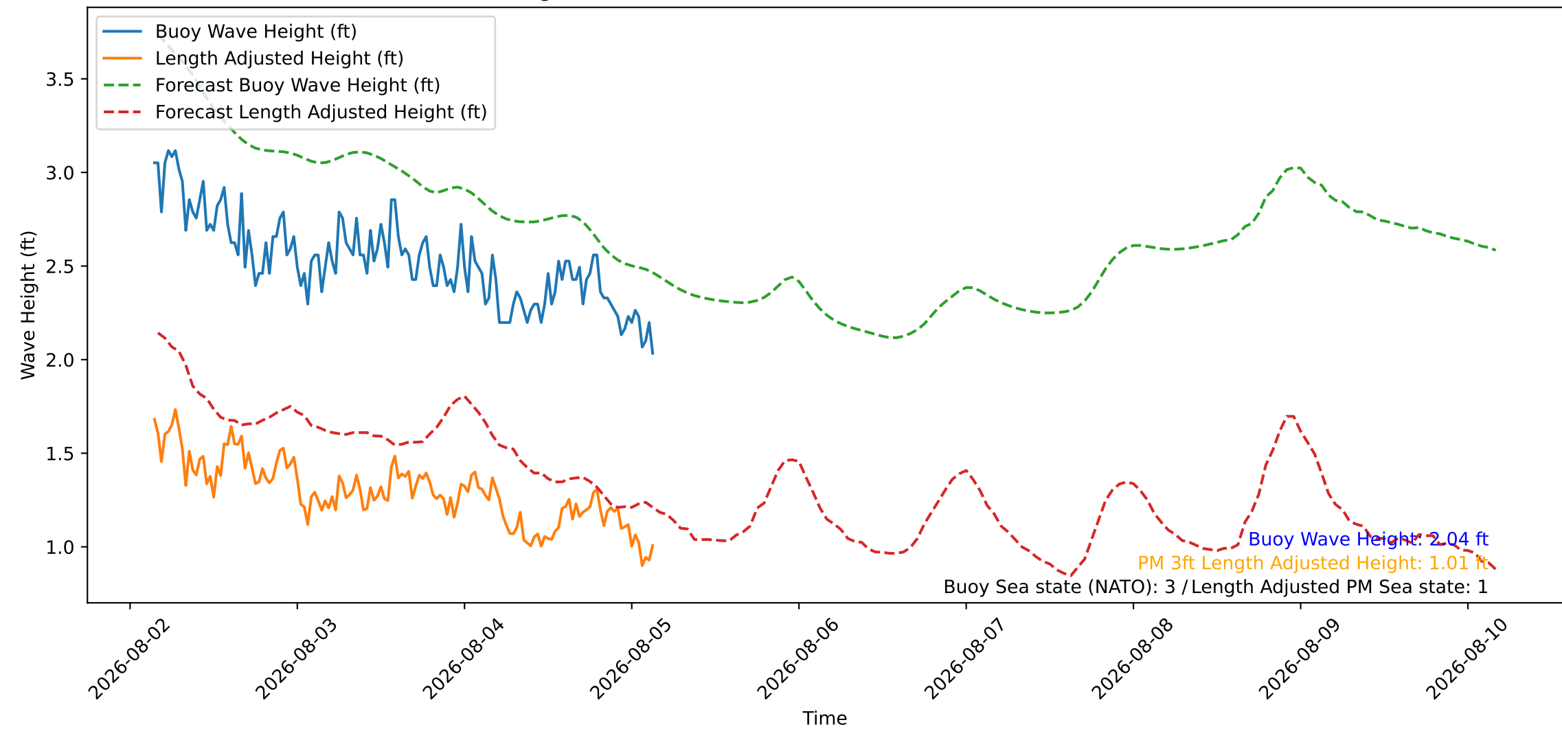
Wave Heights over Time for Oceanside Harbor at 2026-08-05 03:30:27
