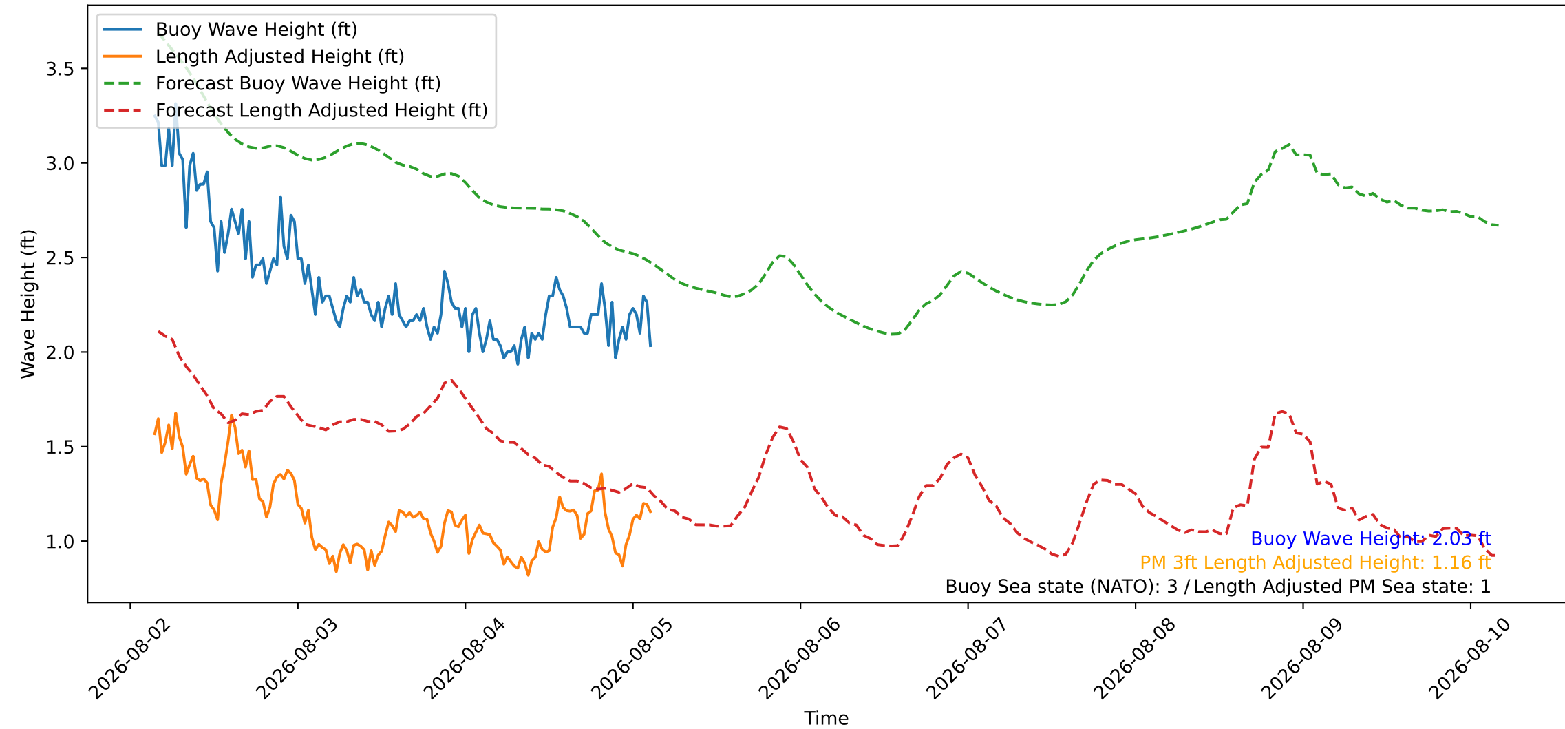
Wave Heights over Time for Green Beach at 2026-08-05 03:31:10
