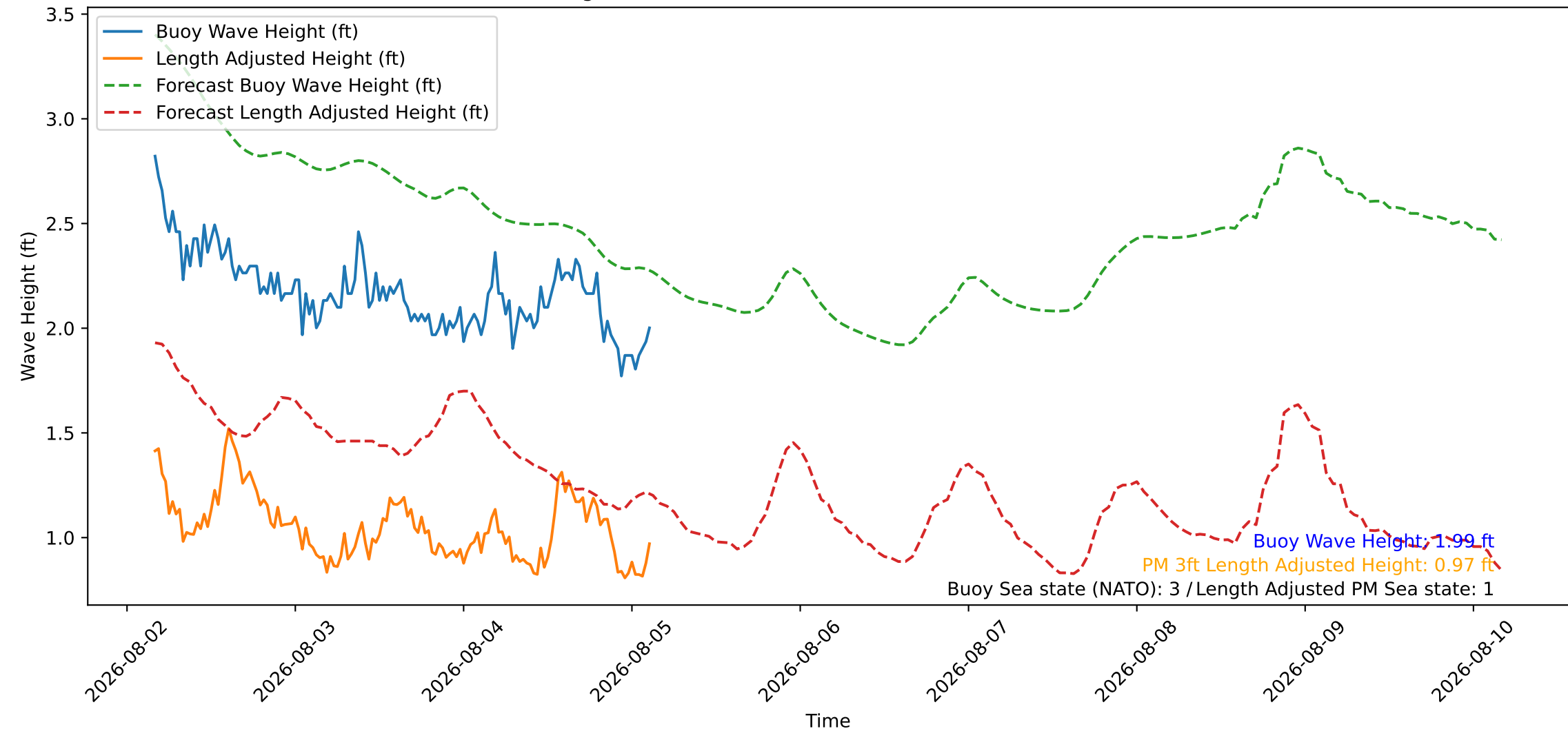
Wave Heights over Time for Red Beach at 2026-08-05 03:30:47
