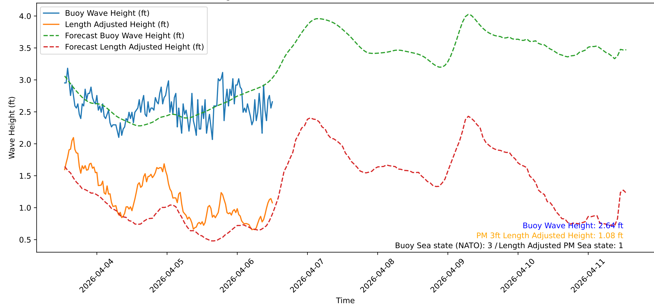
Wave Heights over Time for Oceanside Harbor at 2026-04-06 12:50:31
