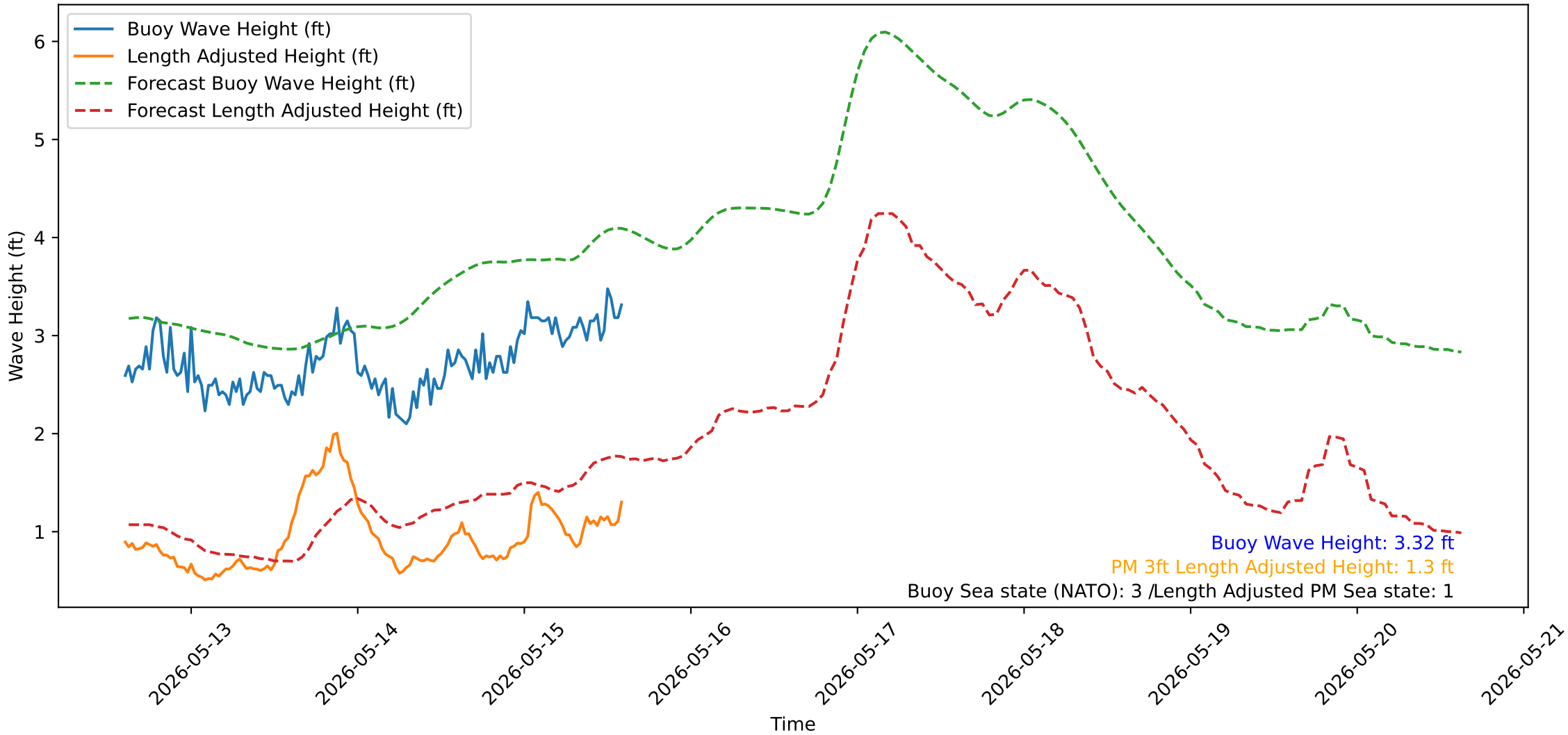
Wave Heights over Time for Green Beach at 2026-05-15 14:41:13
