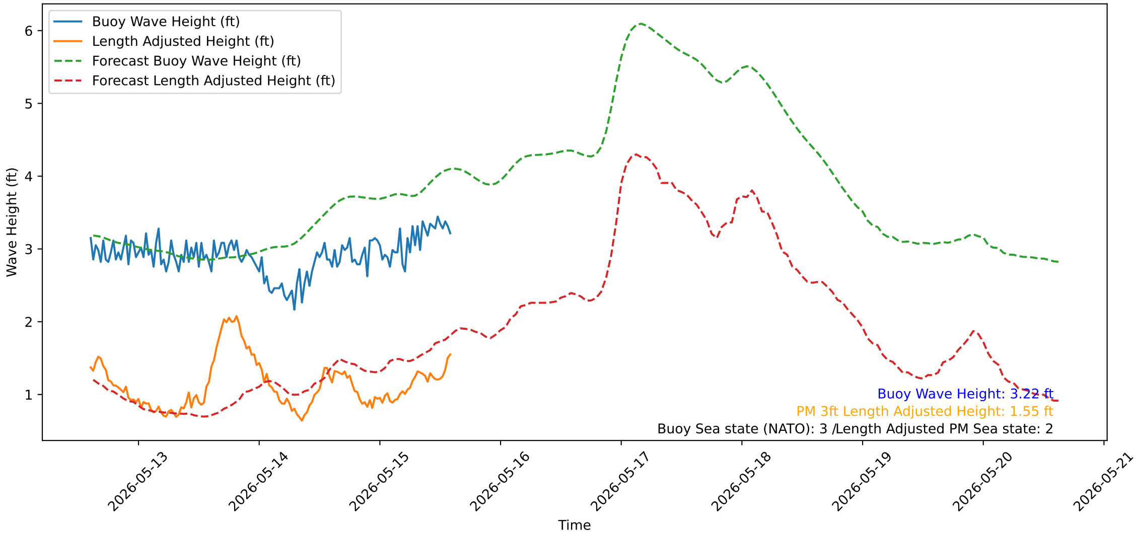
Wave Heights over Time for Oceanside Harbor at 2026-05-15 14:40:31
