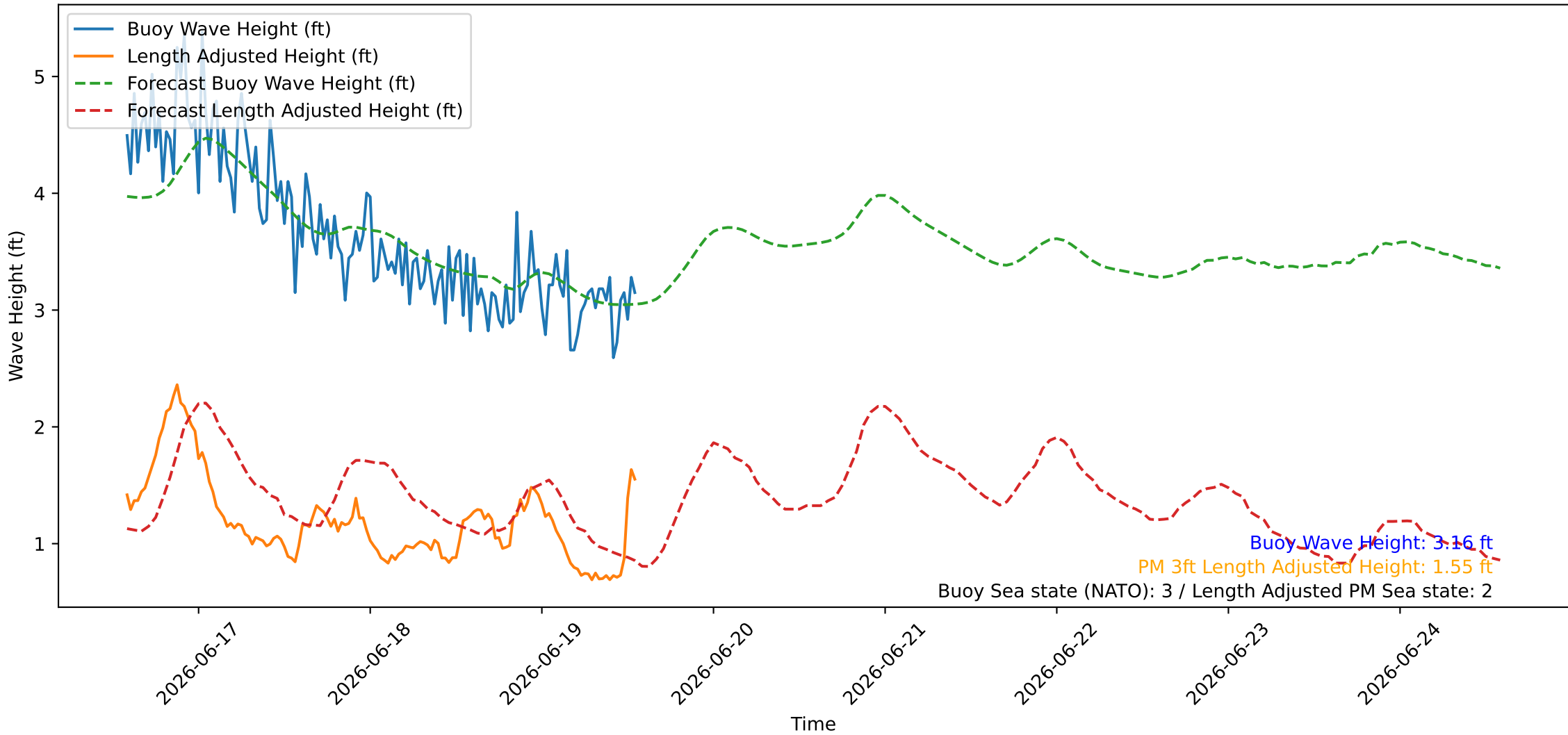
Wave Heights over Time for Red Beach at 2026-06-19 13:50:45
