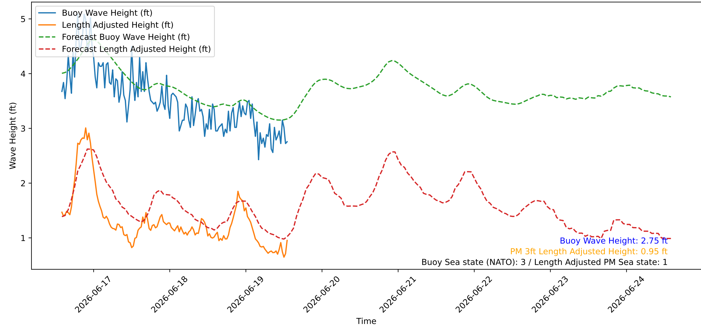
Wave Heights over Time for Green Beach at 2026-06-19 13:51:07
