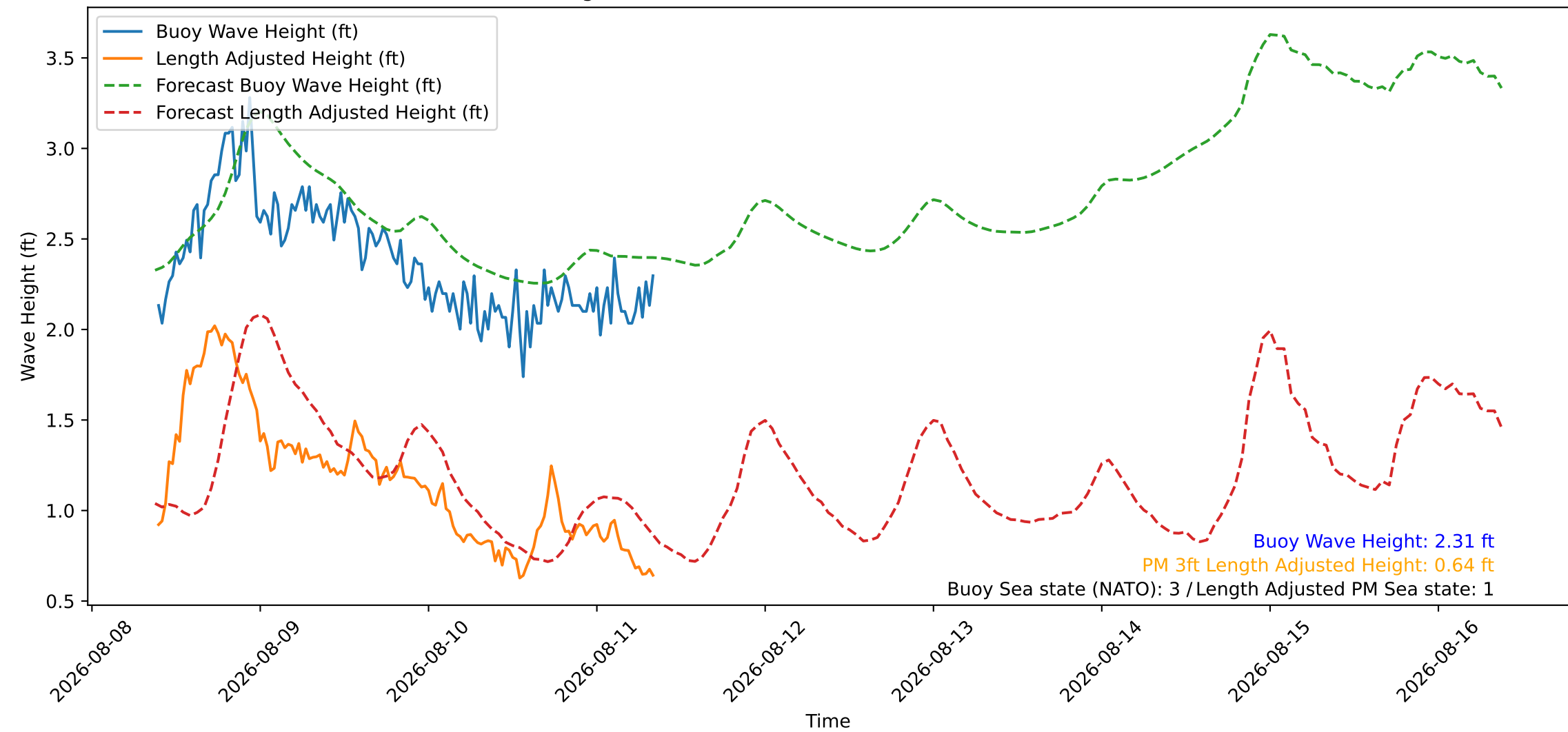
Wave Heights over Time for Red Beach at 2026-08-11 09:00:46
