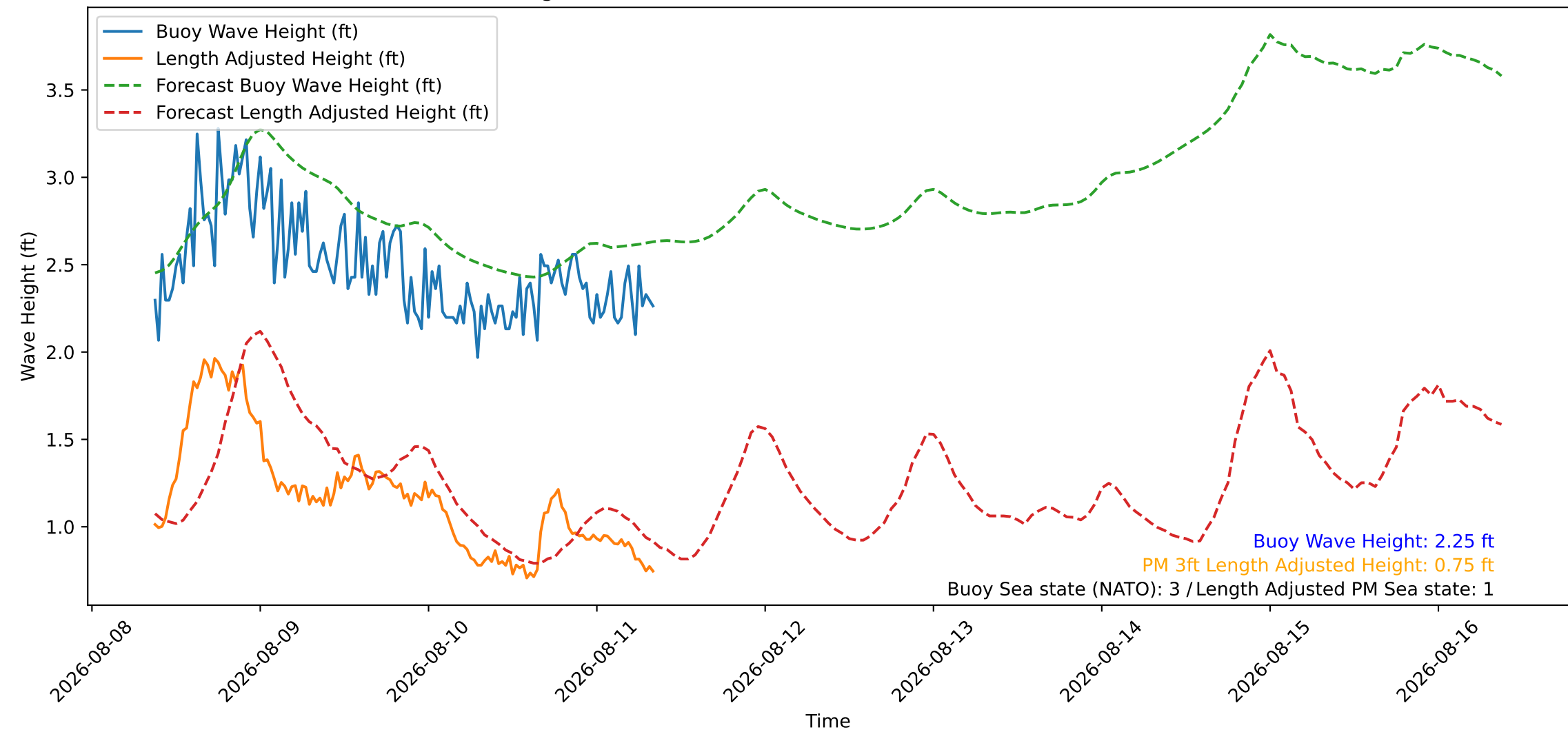
Wave Heights over Time for Oceanside Harbor at 2026-08-11 09:00:26
