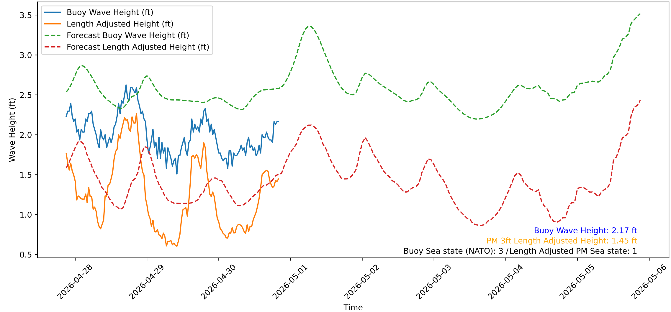
Wave Heights over Time for Red Beach at 2026-04-30 20:40:51
