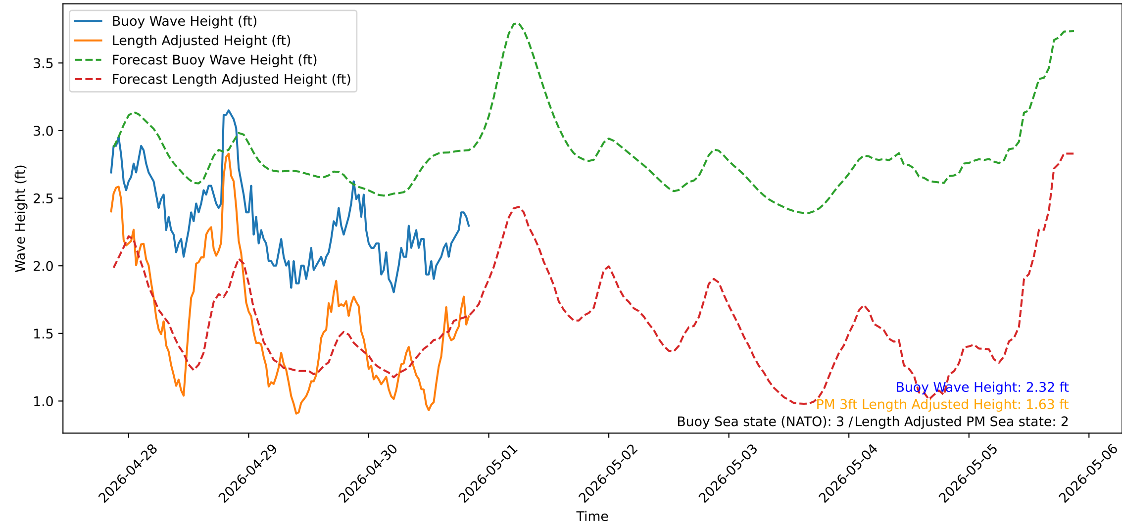
Wave Heights over Time for Green Beach at 2026-04-30 20:41:14
