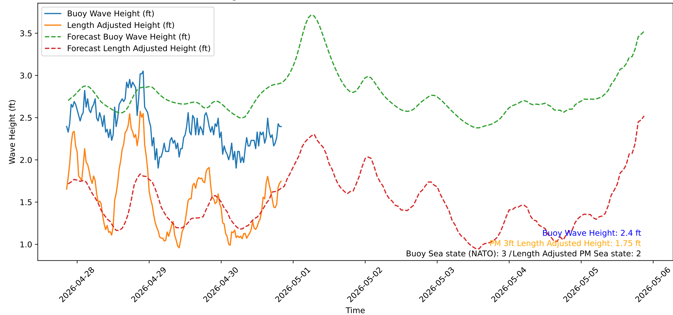
Wave Heights over Time for Oceanside Harbor at 2026-04-30 20:40:31
