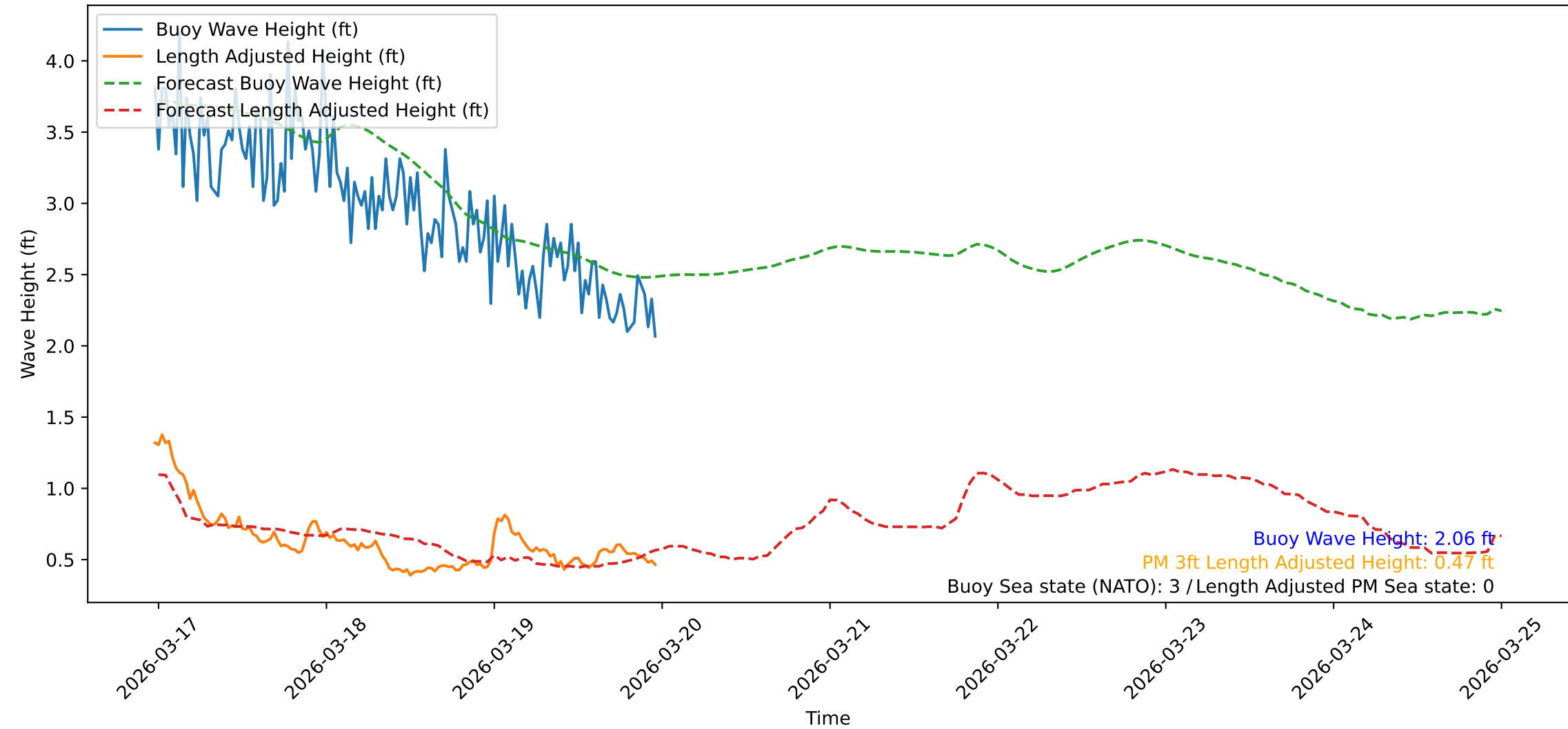
Wave Heights over Time for Green Beach at 2026-03-19 23:41:11
