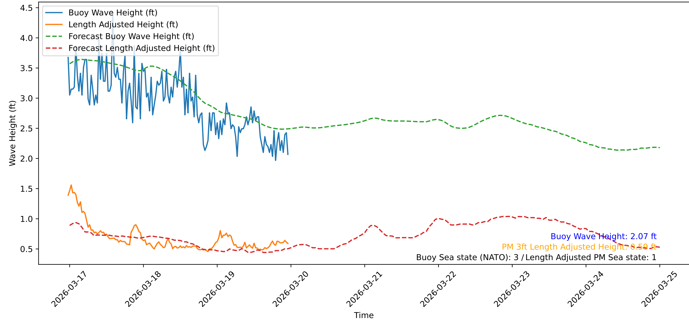
Wave Heights over Time for Oceanside Harbor at 2026-03-19 23:40:32
