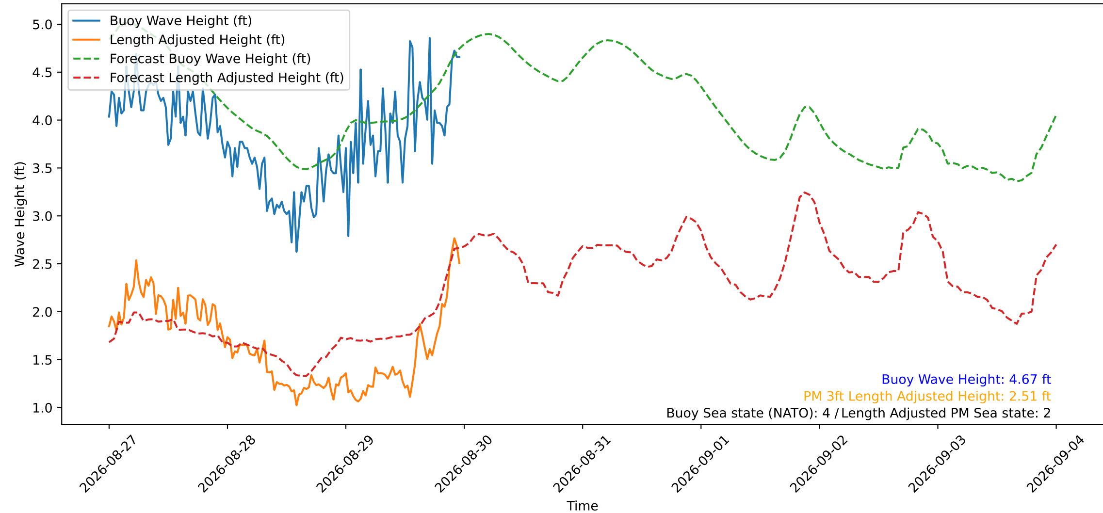
Wave Heights over Time for Green Beach at 2026-08-29 23:41:12
