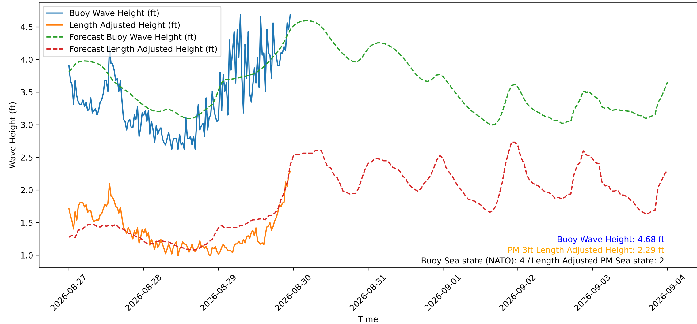
Wave Heights over Time for Red Beach at 2026-08-29 23:40:50
