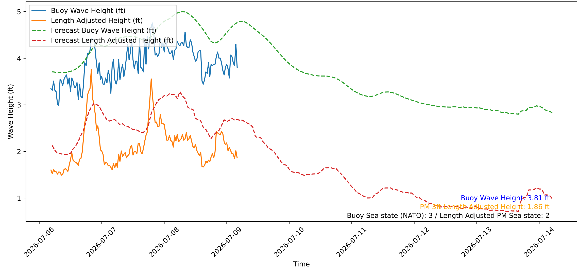
Wave Heights over Time for Green Beach at 2026-07-09 04:41:09
