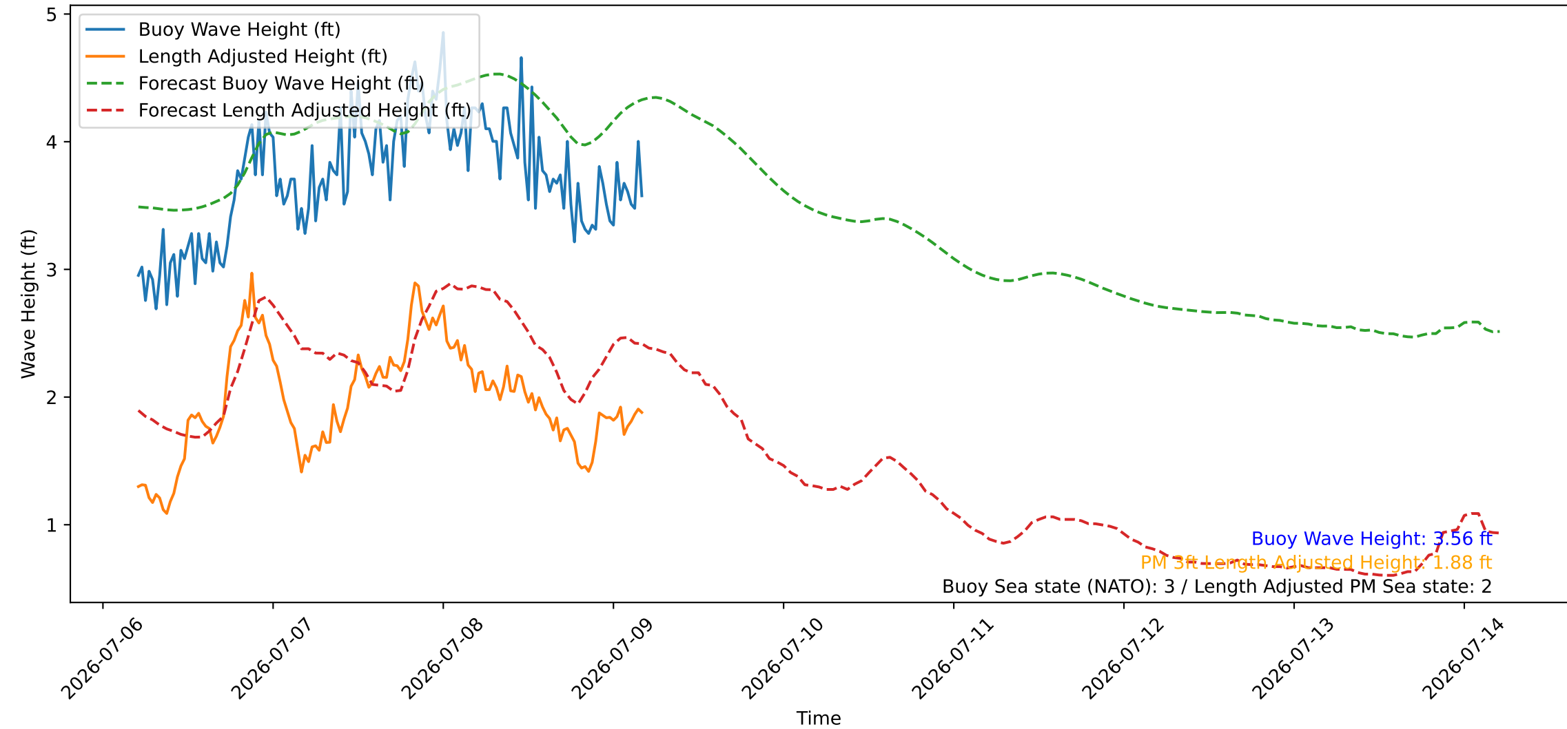
Wave Heights over Time for Red Beach at 2026-07-09 04:40:46
