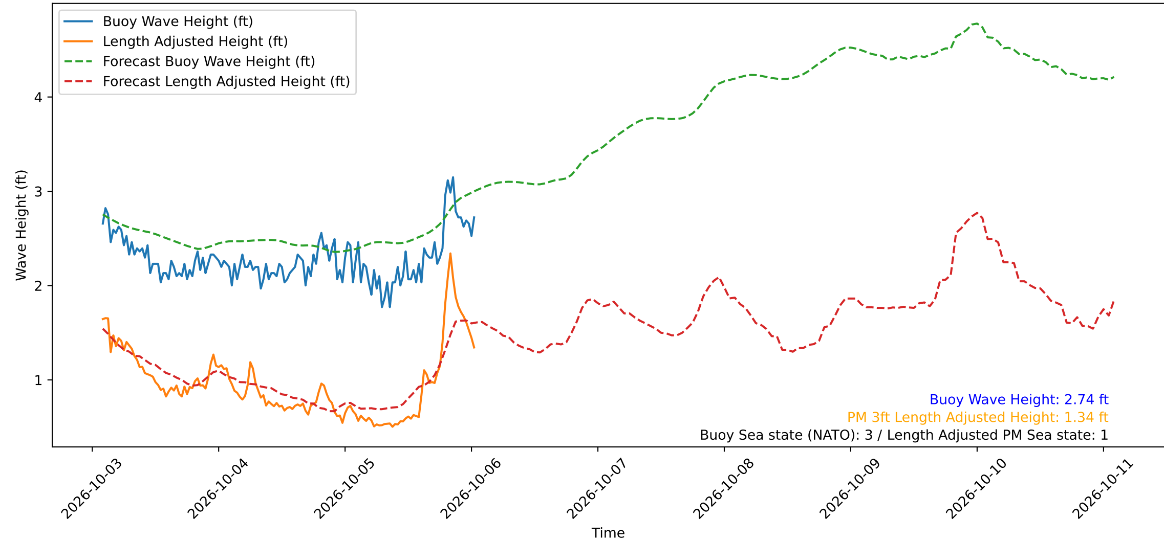
Wave Heights over Time for Green Beach at 2026-10-06 01:31:12
