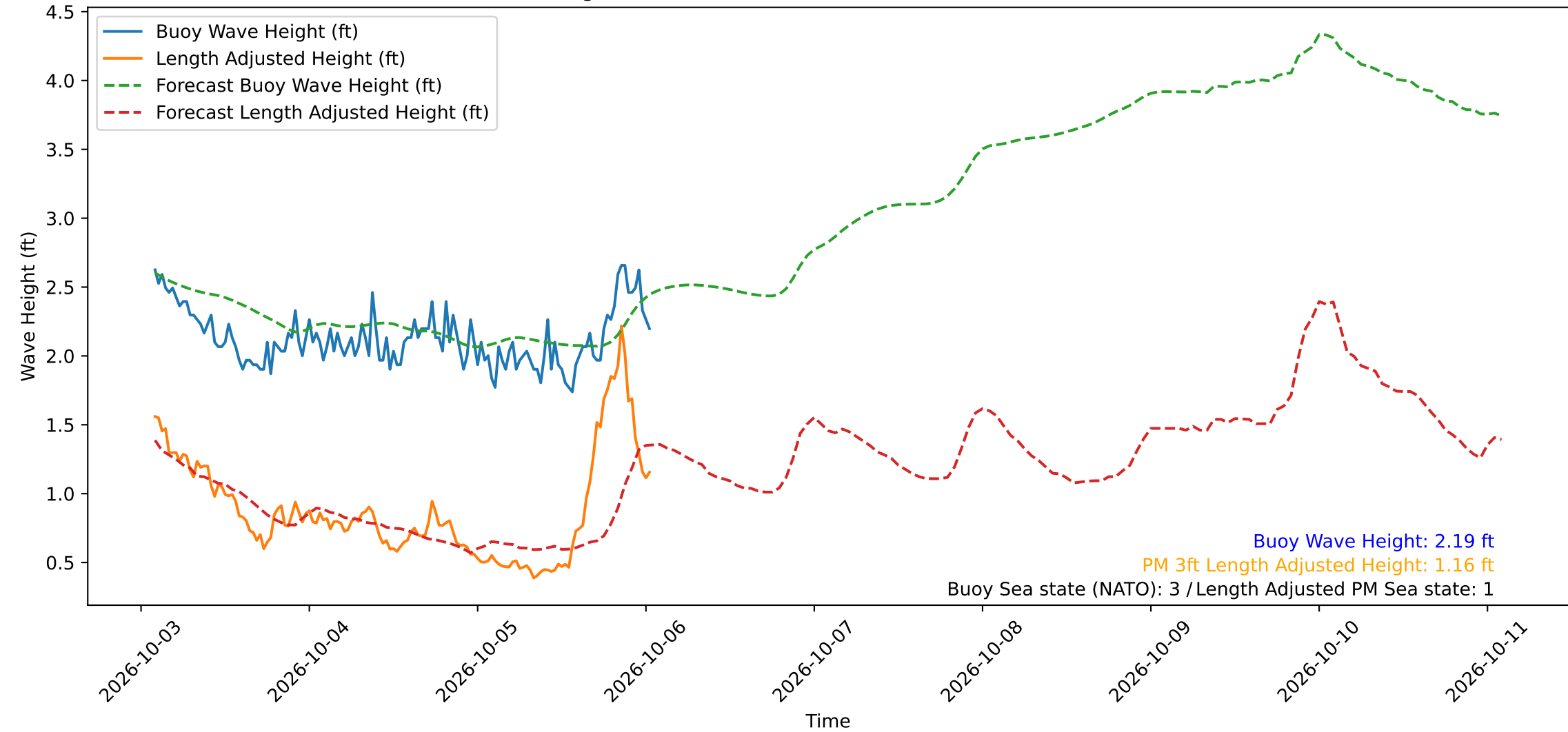
Wave Heights over Time for Red Beach at 2026-10-06 01:30:49
