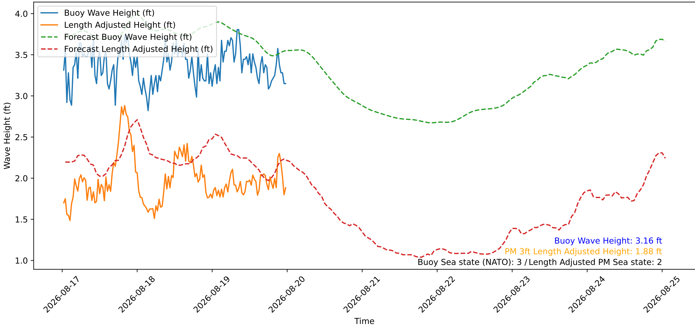
Wave Heights over Time for Oceanside Harbor at 2026-08-20 00:40:26
