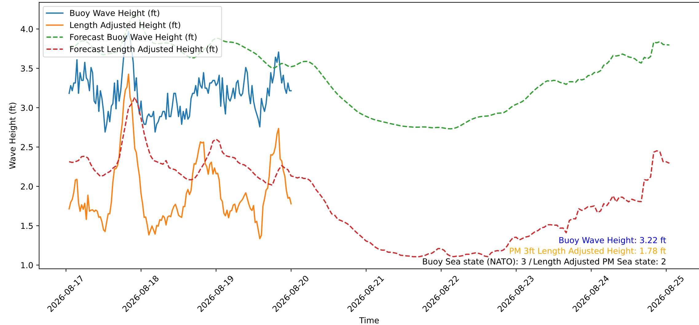
Wave Heights over Time for Green Beach at 2026-08-20 00:41:08
