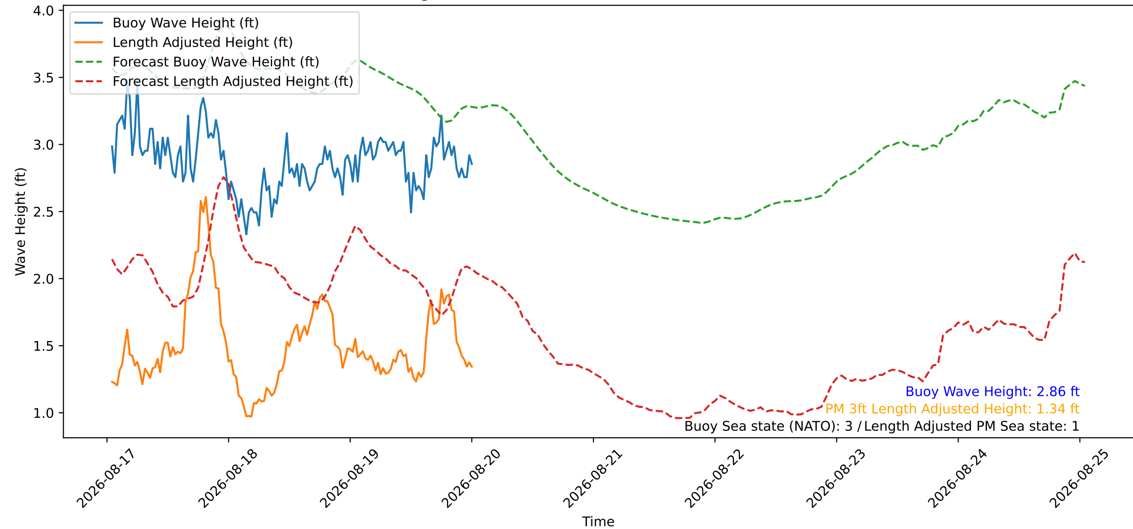
Wave Heights over Time for Red Beach at 2026-08-20 00:40:45
