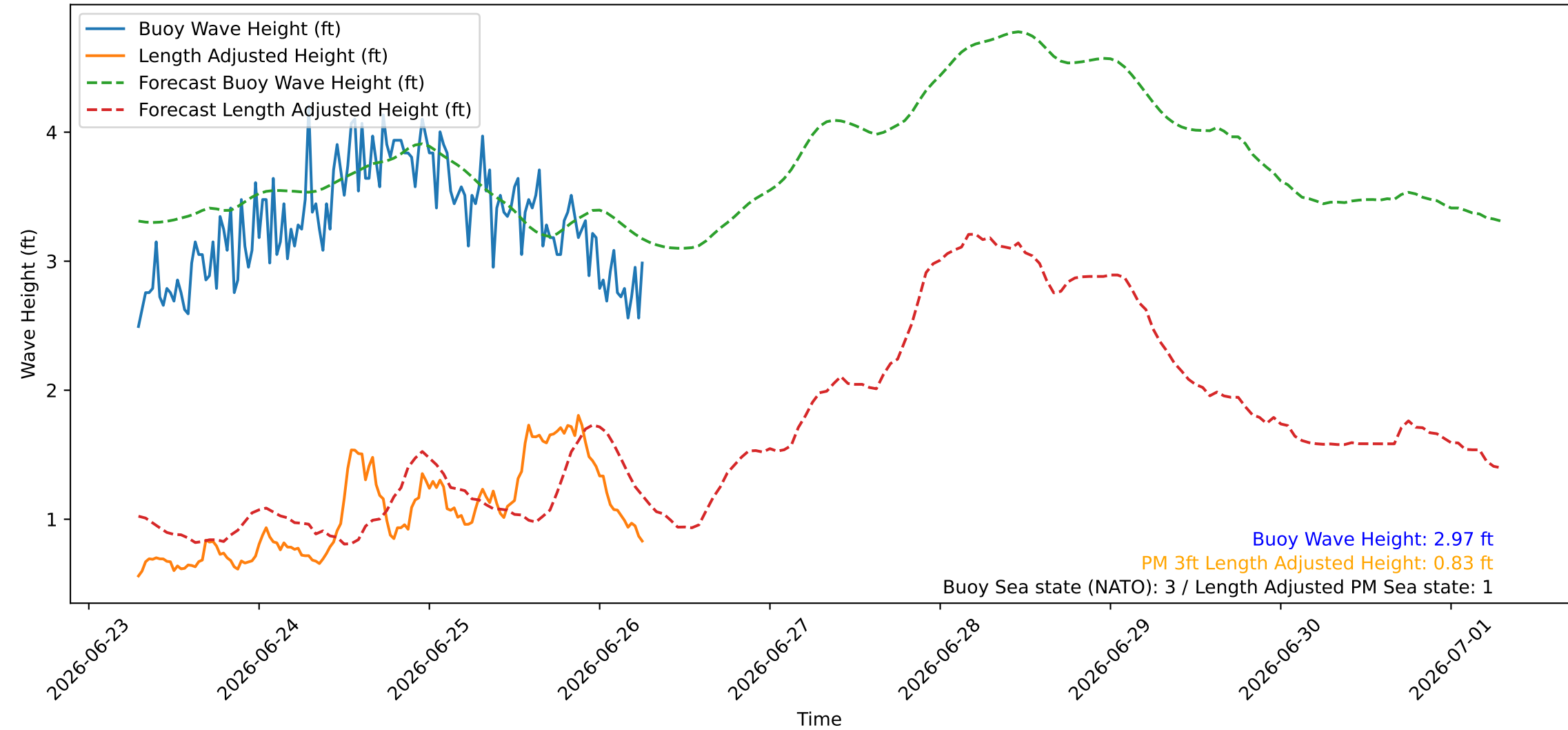
Wave Heights over Time for Green Beach at 2026-06-26 06:51:09
