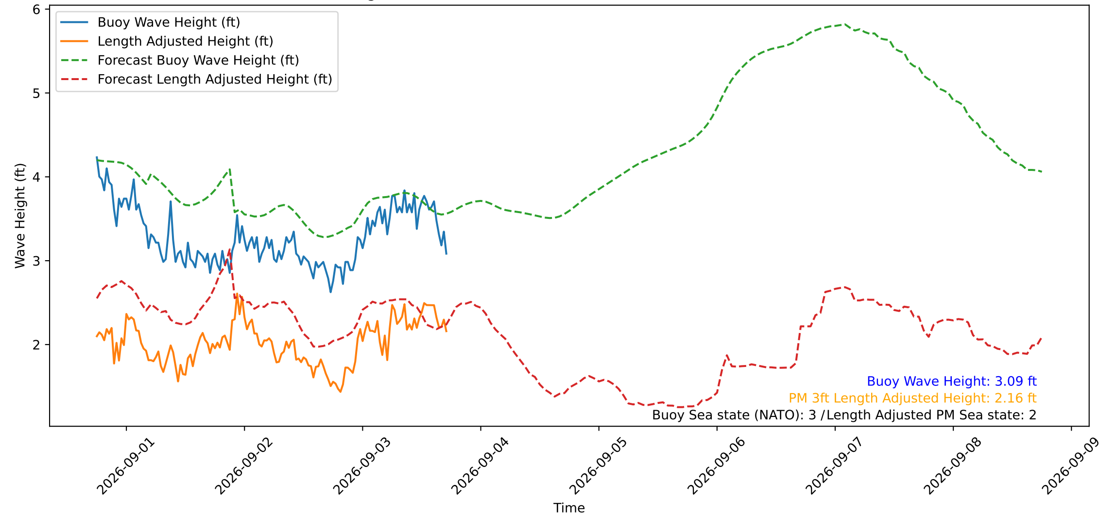
Wave Heights over Time for Oceanside Harbor at 2026-09-03 17:50:29
