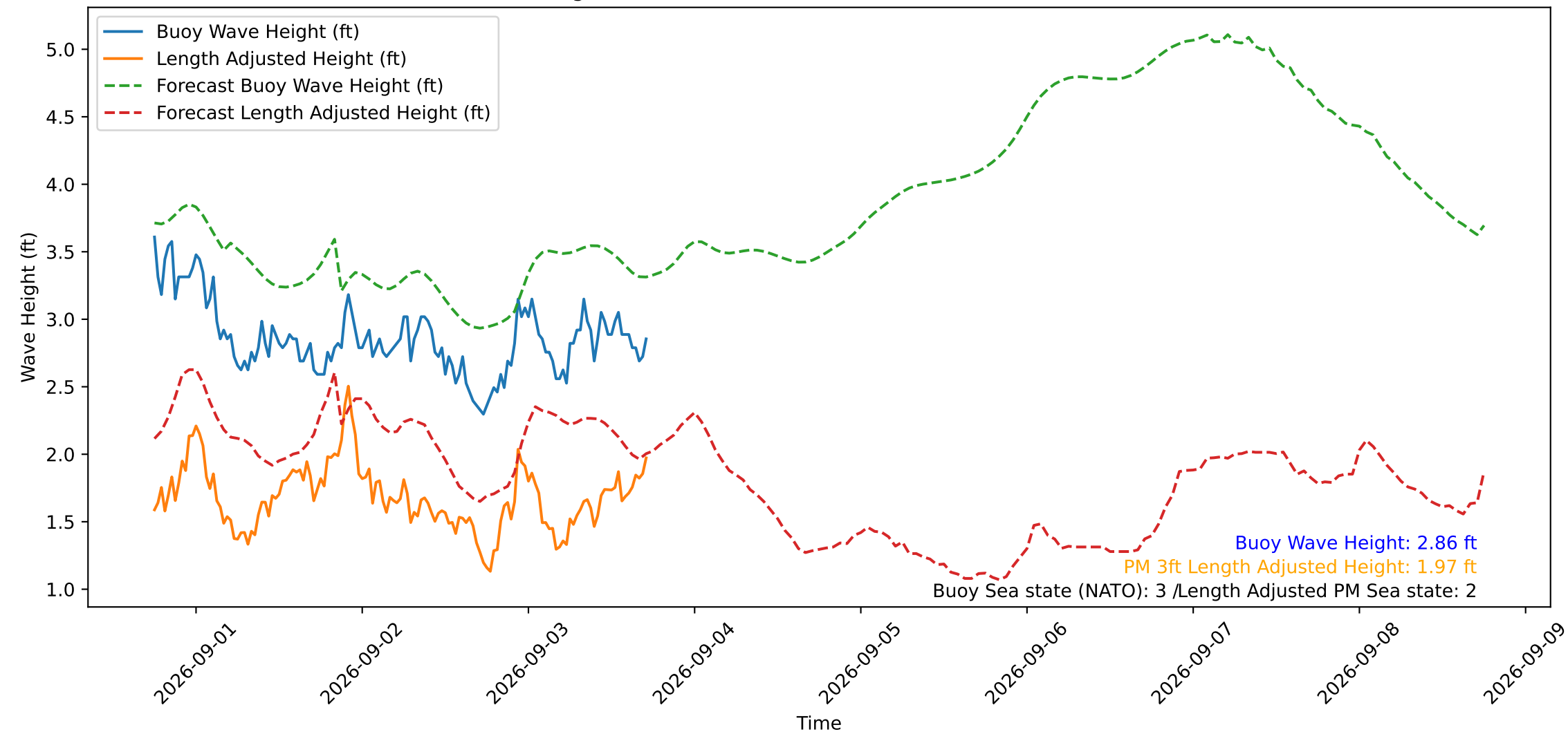
Wave Heights over Time for Red Beach at 2026-09-03 17:50:50
