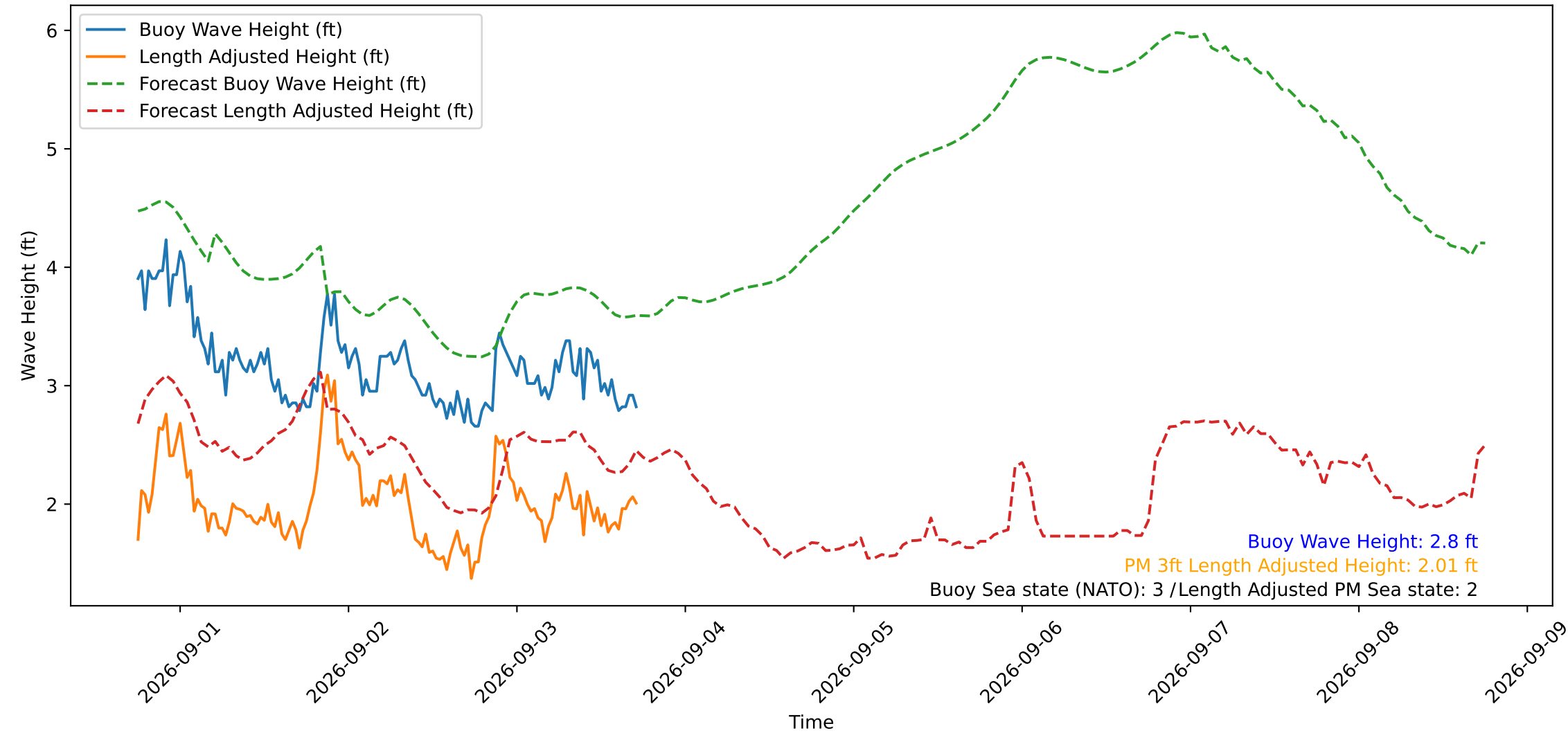
Wave Heights over Time for Green Beach at 2026-09-03 17:51:14
