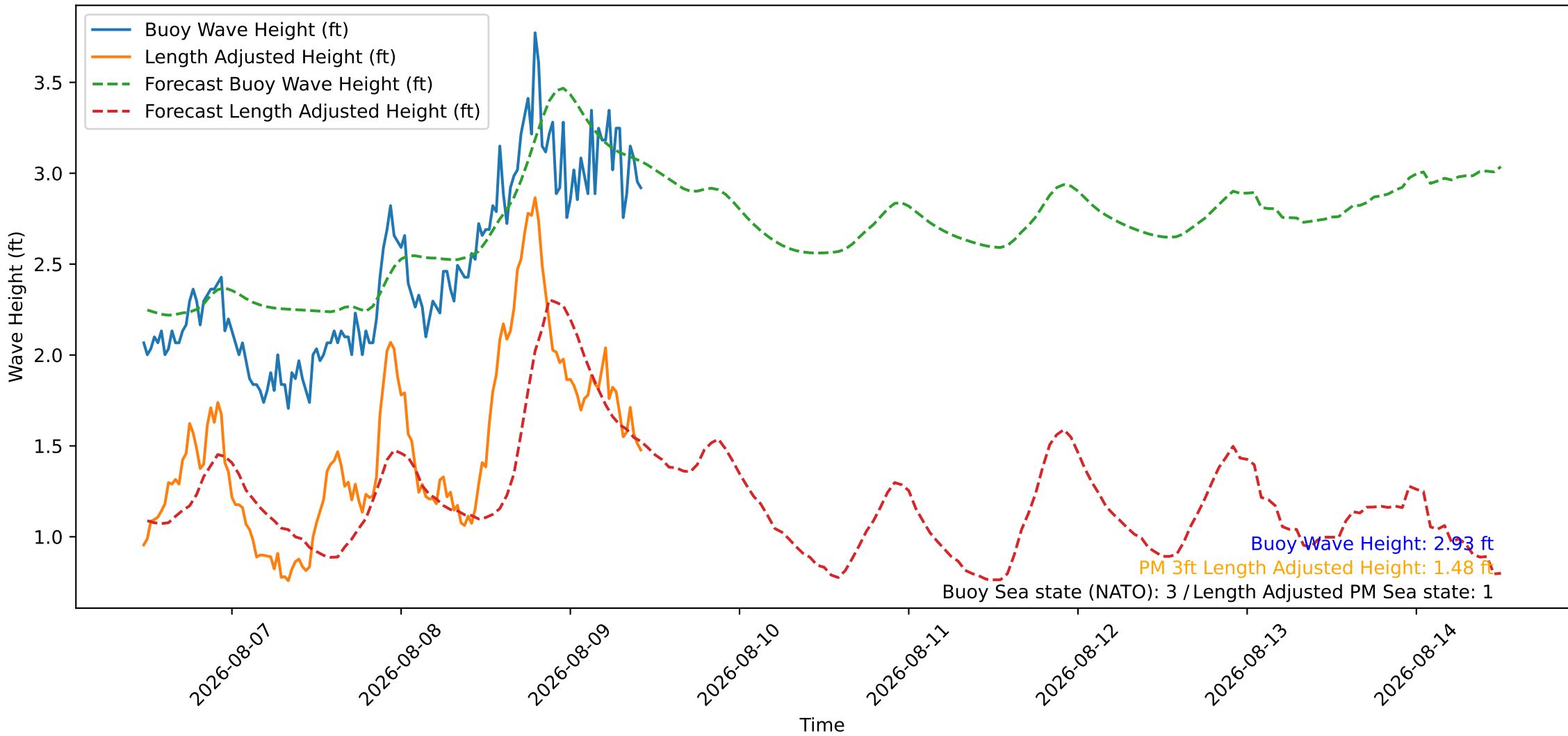
Wave Heights over Time for Green Beach at 2026-08-09 11:31:08
