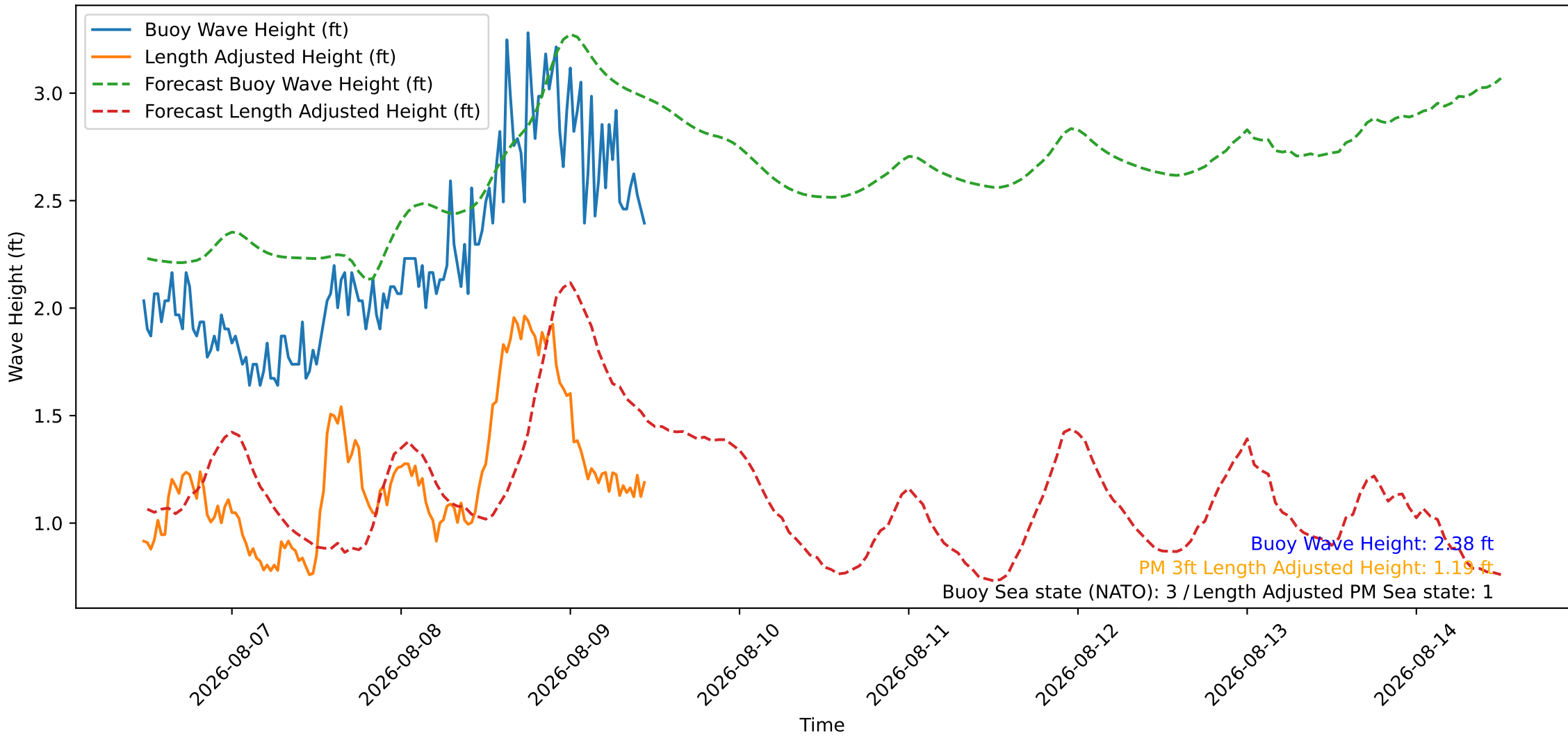
Wave Heights over Time for Oceanside Harbor at 2026-08-09 11:30:27
